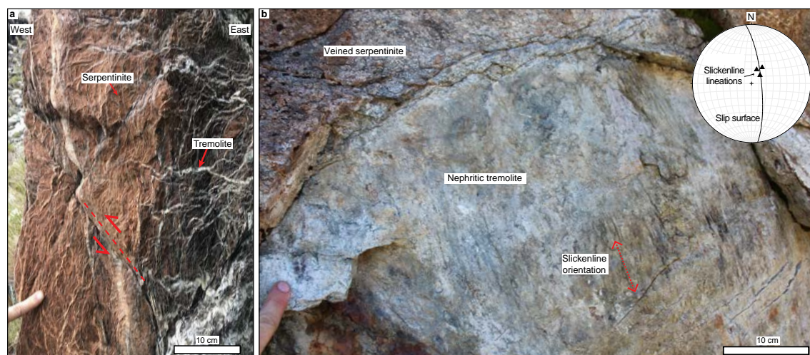
Figure 6. Tremolite vein networks and associated discrete slip surfaces. (a) Multigenerational tremolite vein network at the contact between serpentinite and Caples Terrane schist. Cross-cutting fault noted in red. (b) A discrete slip surface cross-cutting the metasomatic reaction zone between serpentinite and Caples Terrane schist displays steeply plunging slickenlines consistent with overall fault kinematics.
