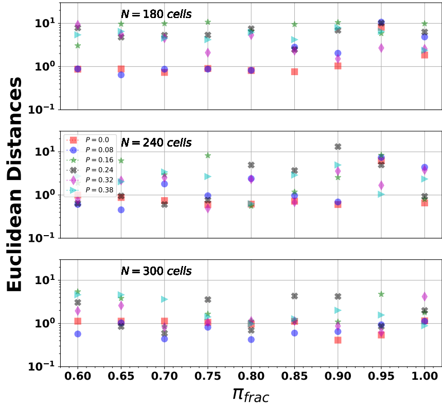
Figure 15. Euclidean parametric distance r_{E-M_{\min}} (Eq. 7), computed for the synthetic series ( M_{\min} = 2.0 ) considering three input parameters ( N , P , \pi_{frac} ). From top to bottom N=180 , N=240 , N=300 [cells per lateral size in the domain].
