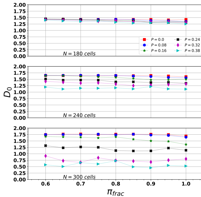
Figure 5. Fractal capacity dimension, D_0 (Section 5.1.1) computed for different synthetic series considering three input parameters: the domain size, N , (from top to bottom N=180 , N=240 , N = 300 cells per lateral size); the initial load order distribution, P ; and on-faults load-transfer value, \pi_{frac} .
