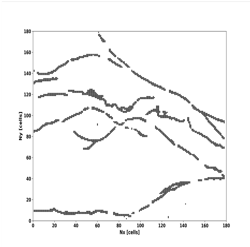
Figure 1. Map (azimuthal view) of the Northridge fault system. It is digitalized to include in our computing domain where each pixel of the map corresponds to a cell (x,y) in our array.
