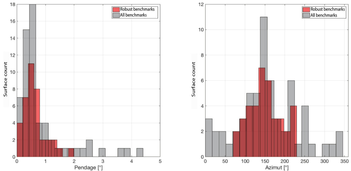
Figure 10: Tilt and azimuth distribution. Left panel is density distribution for surface maximum tilting in degree. Right panel is azimuth of maximum dipping relative to the north. For each histogram, red and grey populations are for robust and primary detected markers.
