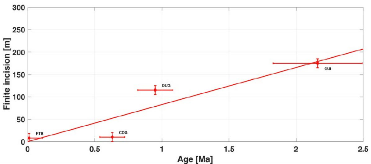
Figure 5: Relation of finite incision-burial age for the Rieutord canyon. Finite incision is the elevation of the sampling site relatively to the current riverbed. RTE for Route Cave, CDG for Camp de Guerre Cave, DUG for Dugou Cave and CUI for Cuillère Cave
