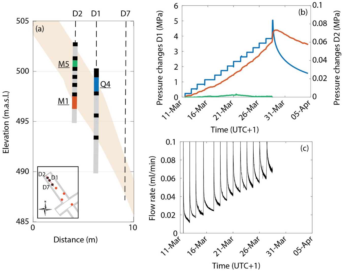
Figure 9: a) Projection on plane of boreholes BCS-D1 and BCS-D2 and their intervals. The inlet shows the location of the boreholes and the orientation of the plane. b) Pressure changes in the injection interval Q4 (blue) and response at two intervals in the fluid monitoring borehole (M1 in red and M5 in green). The positions of the monitor intervals with respect the injection interval is shown in panel (a). c) Flow rate at the syringe pump.
