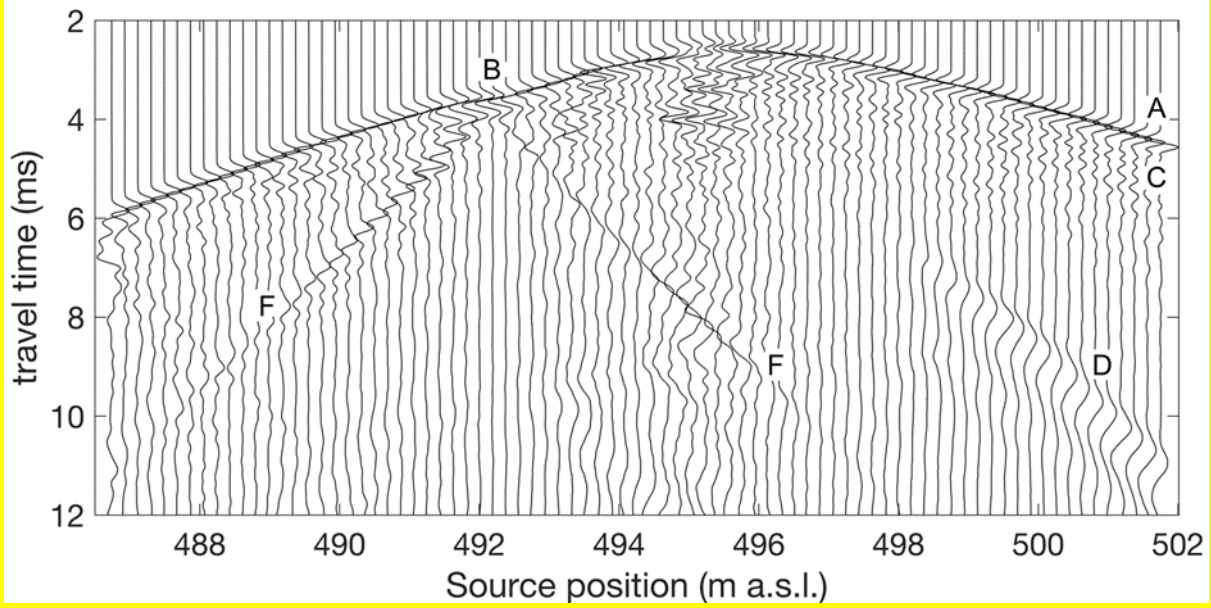
Figure 13: Common-receiver gather of processed seismic data, recorded with a cemented geophone in borehole BCS-D3, while a P-wave sparker source was employed at 25 cm intervals in borehole BCS-D4. . Labelled seismic events are the P-wave arrivals (A) with notable delay for sources fired within the Main Fault (B), slow and fast S-wave modes (C), tube wave propagating along the source borehole (D) and tube wave reflected at the Main Fault (F).
