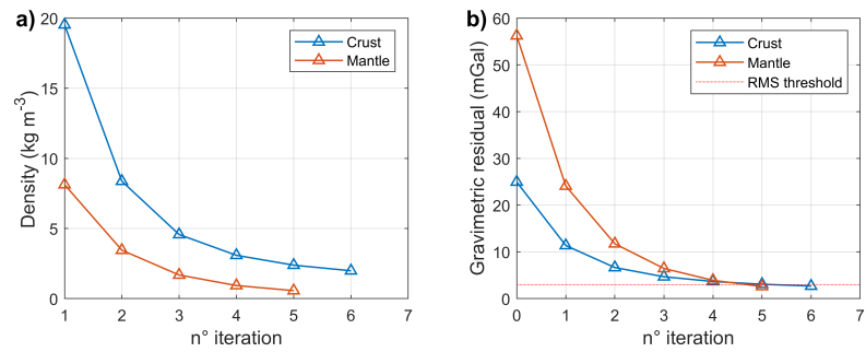
Fig. 1. Figure Rv-1: Illustration of the effectiveness of the iteration steps in crust and mantle. A) Root means square density correction over the volume of crust and mantle during iterations. B) Root mean s
