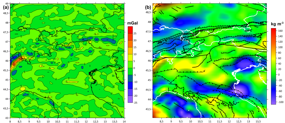
Fig. 2. Figure Rv-2 Final gravity residual (left) and density correction (right) in the last step of the iteration for the crustal modelling.
