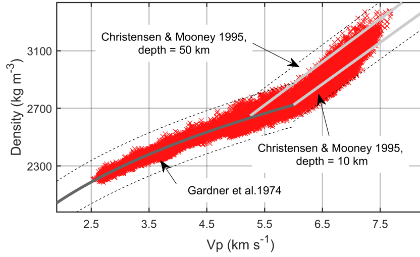
Fig. 3. Figure Rv-3: Comparison of published densities versus V_p relations discussed in (Brocher, 2005), dark grey continuous line represents the Gardner's equation, light grey continuous line represents Chri
