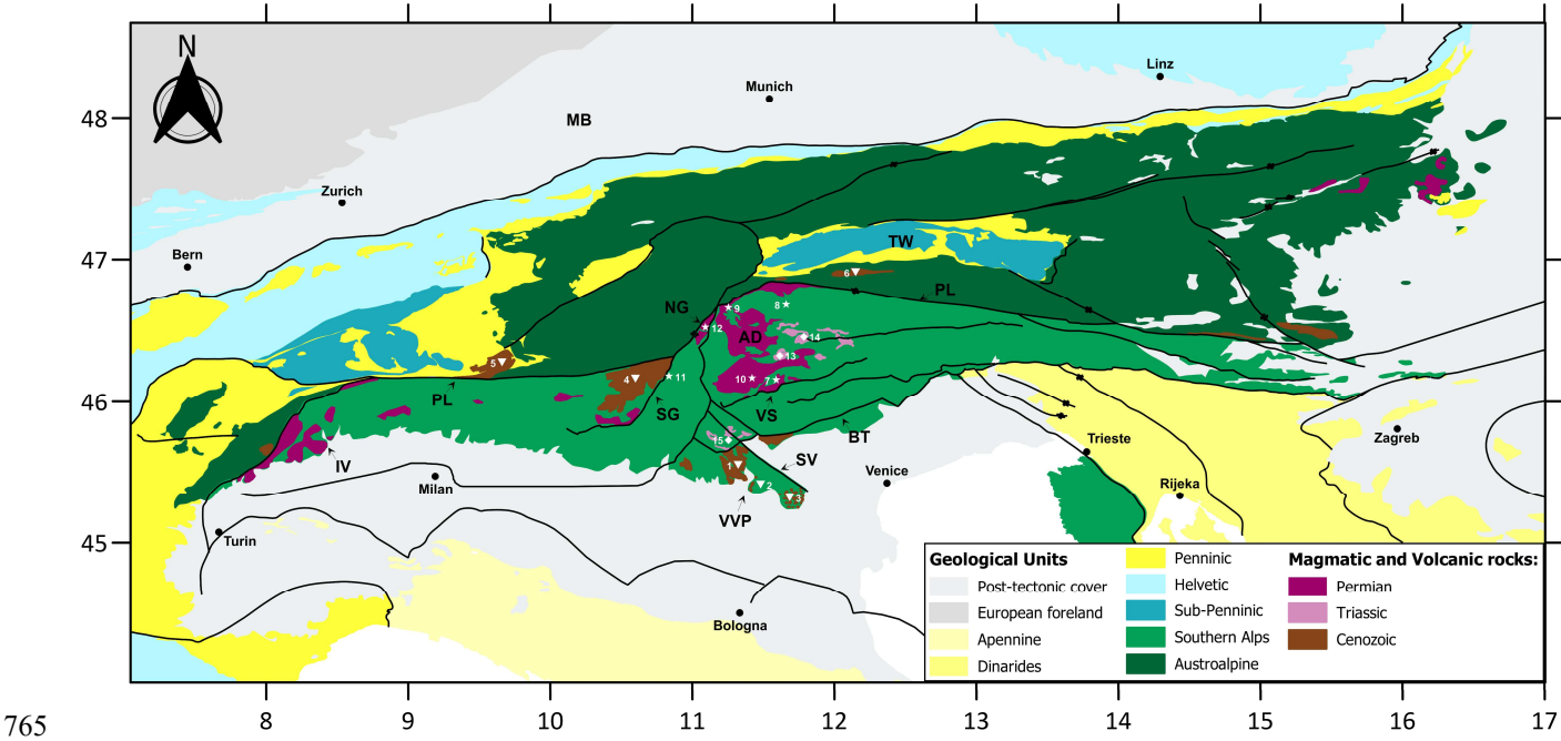
Figure 1 – Geologic chart of the Alps modified after (Pfiffner, 2015) and main magmatic and volcanic bodies (Bigi et al., 1990a, 1990b; Schuster and Stüwe, 2008). VVP: Venetian Volcanic Province; SV: Schio-Vicenza Fault; BT: Bassano-Montello Thrusts; VS: Val Sugana Thrust; SG: South Giudicarie Fault; NG: North Giudicarie Fault; AD: Athesian Volcanic District; PL: Periadriatic Line; IV: Ivrea-Verbano Complex; TW: Tauern Window; MB: Molasse Basin. 1) Lessini Mountains; 2) Berici Hills; 3) Euganei Hills; 4) Adamello Batholith; 5) Mesino-Bragaglia Batholith; 6) Vedrette di Ries/Riesen Ferner Batholith; 7) Cima d’Asta Intrusion; 8) Bressanone-Chiusa Intrusions; 9) Ivigna Intrusion; 10) Monte Croce Intrusion; 11) Monte Sabion Intrusion; 12) Monte Luco Intrusion; 13) Predazzo Intrusion; 14) Monzoni Intrusion; 15) Recoaro-Pasubio Intrusions.
