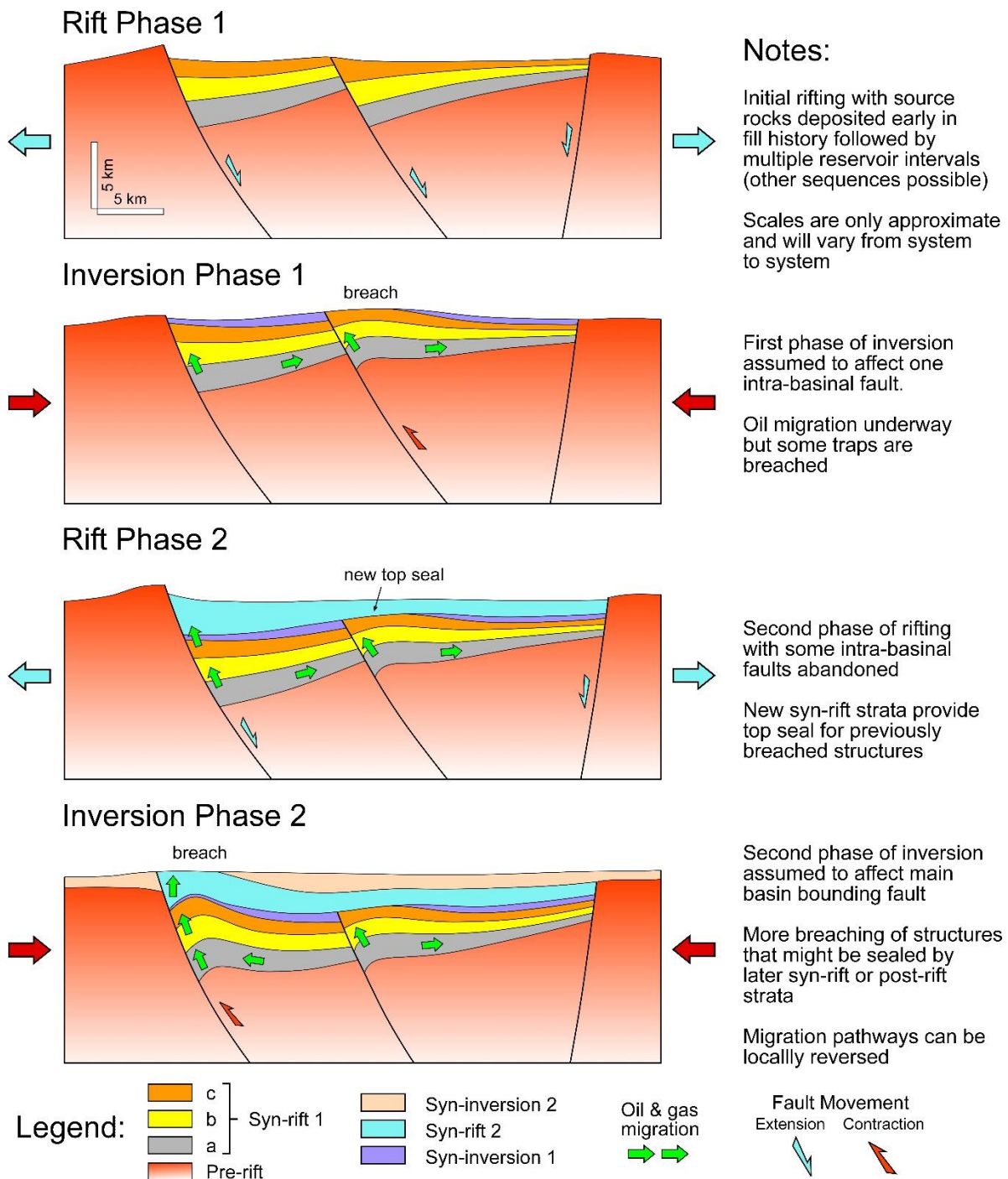
830 Figure 14a. Schematic illustration of some of the possible effects of superimposed, alternating phases of extension and inversion on a rift basin. For simplicity two inversion events are shown affecting different faults, which is commonly observed in the Western Desert of Egypt but will not always be the case.
