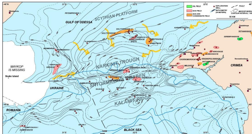
Figure 13. Isopach of the post-inversion Oligocene to Lower Miocene Maykop Suite in the Odessa Shelf, modified from Gozhik (2010). For location see Fig. 8. Contour intervals are in meters. Note that the thickest Maykop is not captured by the currently available well control (cf. Fig. 9). The depicted sediment entry points and the deep-water distribution patterns are entirely speculative and are shown here to highlight the stratigraphic trapping potential in the Karkinit basin.
