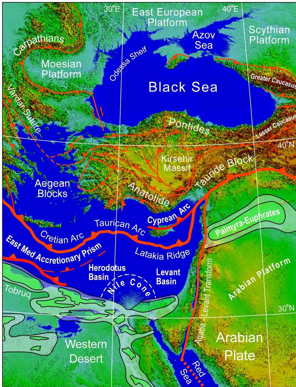
750 Figure 1: Tectonic setting of the Western Desert (Egypt), eastern Mediterranean and Black Sea. Plate boundaries and major faults are shown in red. Triangles are on upthrust block of thrust and reverse faults. Major sedimentary basins of the Western Desert and Arabian plate are shaded in green. Modified from Okay and Tüysüz (1999) and Bosworth et al. (2008) and references therein. Base is SRTM digital elevation model (Jarvis et al., 2008). UTM Zone 36 projection.
