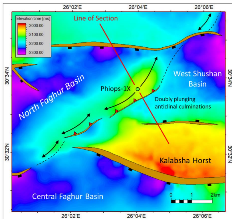
Figure 6: Detailed time structure map of the Phiops inversion trend. Other wells have been removed for clarity. See Fig. 4 for location and legend.
