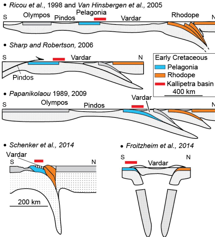
820 Figure 2: Geodynamic interpretations of the Hellenides in the Early Cretaceous according to different authors. Note that there is no consensus on the Early Cretaceous geodynamic framework at the onset of the Kallipetra Basin between the Pelagonian zone and the Vardar domain.
