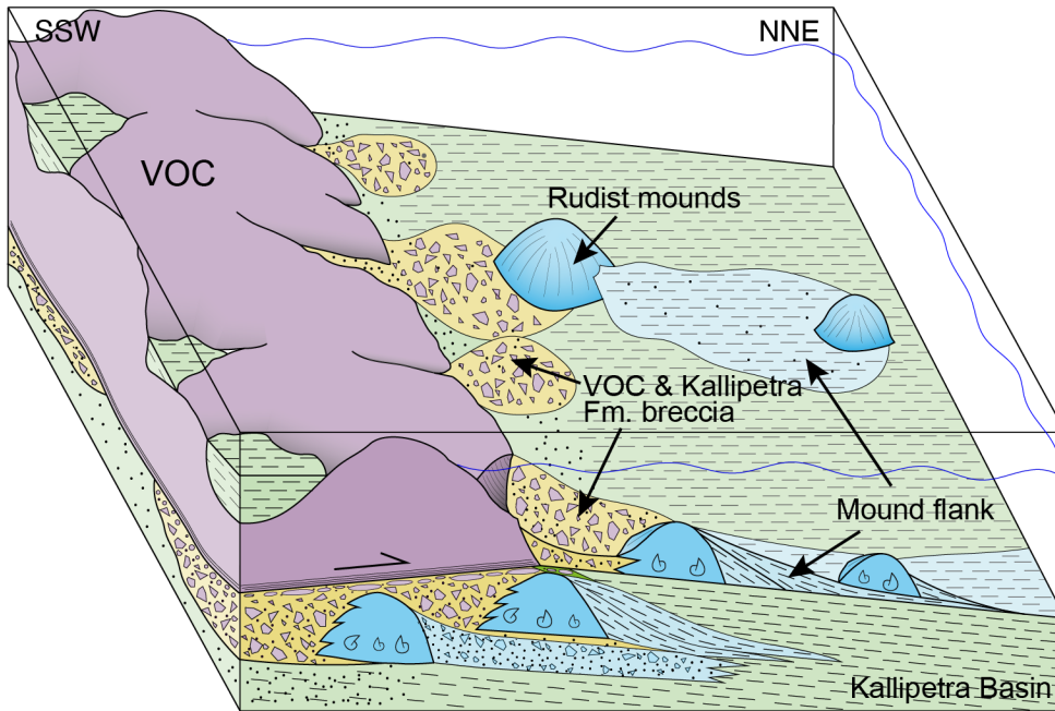
880 Figure 13: Schematic diagram showing the sedimentary and tectonic environment of the Kallipetra Basin during the Turonian, and the overriding of rudist mounds by the resumed thrusting of the VOC. Colors correspond to those on the geological map (Fig. 3).
