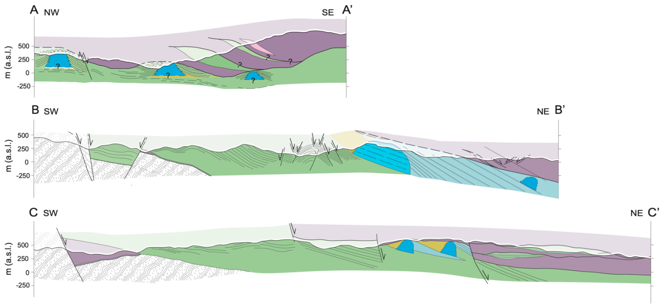
860 Figure 8: Geologic cross-sections of the mapped area, colors corresponding to those on the geological map (Fig. 3).
