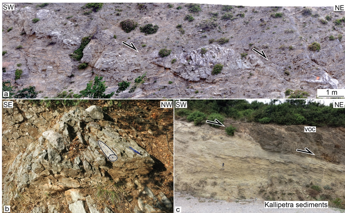
855 Figure 7: (a) Asymmetric boudin of a limestone showing top-to-the NE shear sense. (b) Cigar-shaped clasts in a polymictic conglomerate of the mound top within the shear zone below the VOC (with sketch of the uniaxial ellipsoid mimicking the shape of the clasts). The stretch axis (X) of the prolate finite strain is parallel to the regional mineral and stretching lineation. (c) Tectonic contact between the Kallipetra Basin and the VOC with a top-to-the NE shearing.
