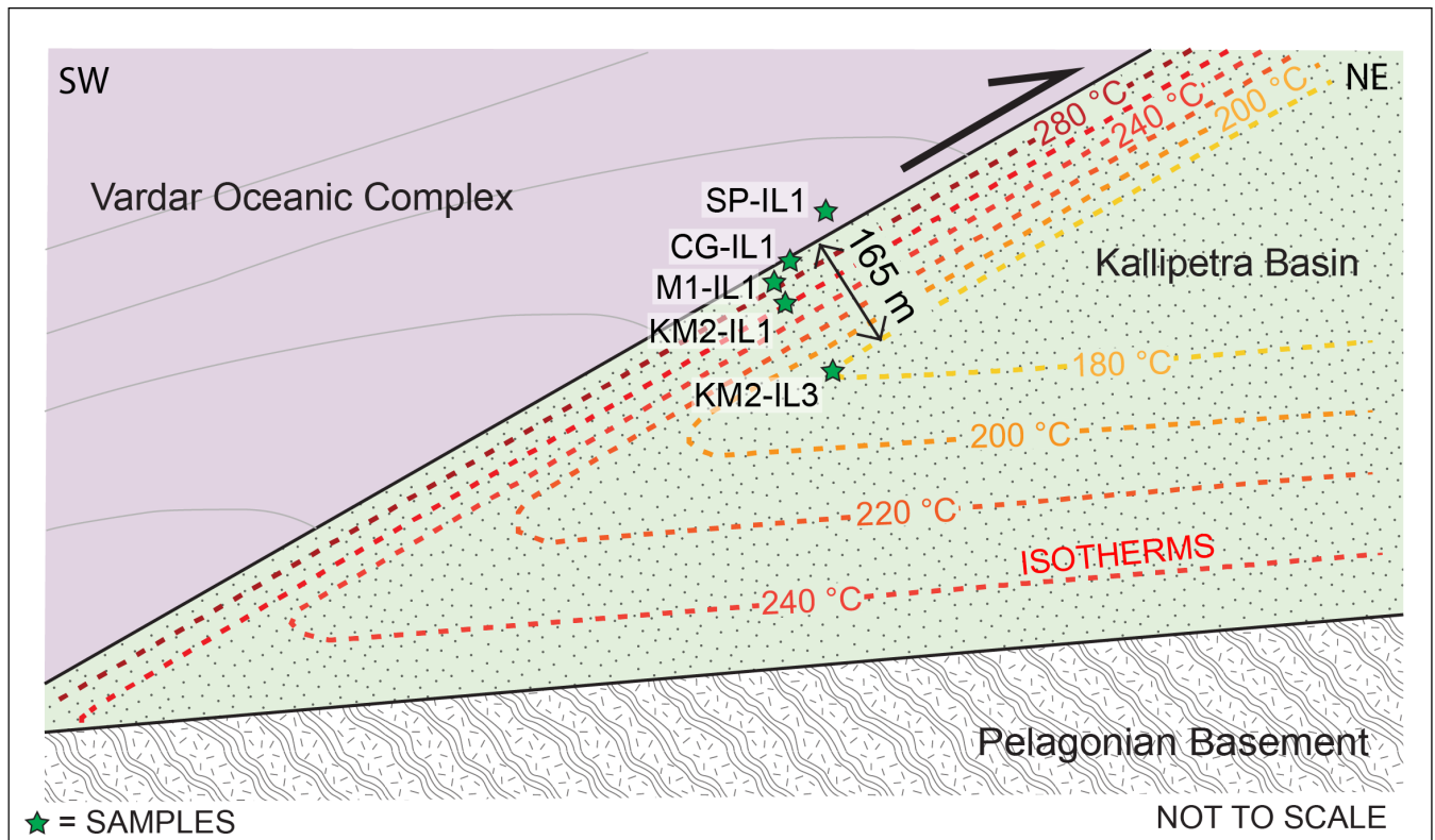
870 Figure 11: Schematic diagram showing the inverse geothermal gradient at the contact between the VOC and Kallipetra Basin.
