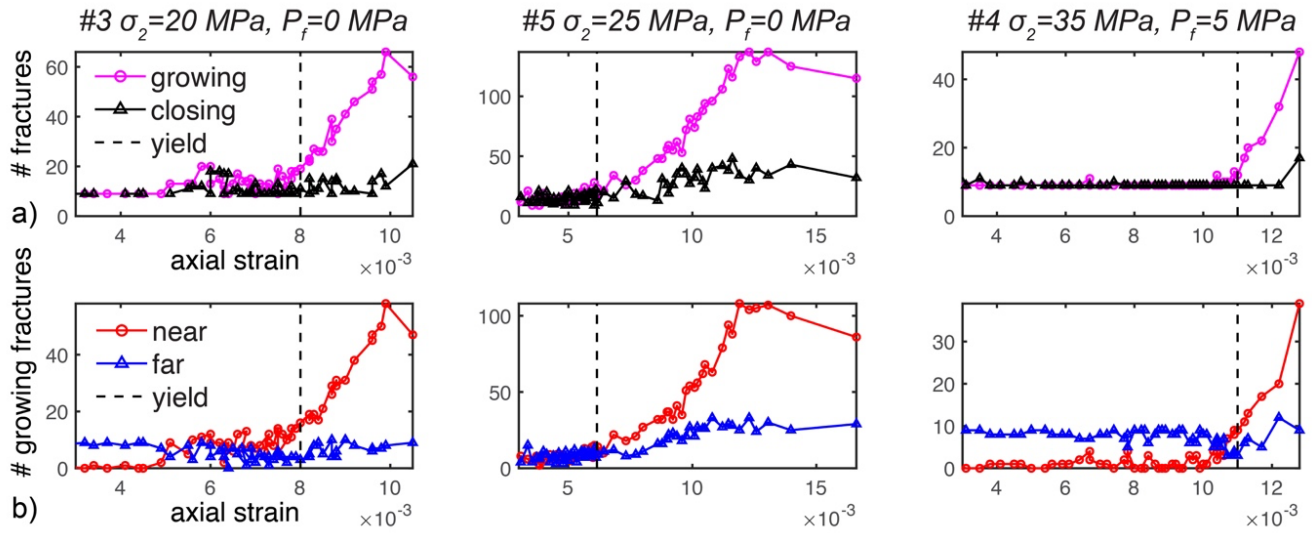
605 Figure 6: The influence of stress perturbations on fracture growth. a) The number of growing (magenta circles) and closing (black triangles) fractures. b) The number of growing fractures that do ( near , red circles) and do not ( far , blue triangles) have other fractures within one fracture length of them throughout loading. If one fracture (fracture #1) is located within y distance of another fracture (#2) with length y , then fracture #1 is counted in the near category. Following the macroscopic yield point, the number of growing fractures located near to other fractures exceeds the number located far from others. This observation suggests that the local perturbations of the stress field produced by fracture growth tend to promote the growth of other fractures following yielding.
