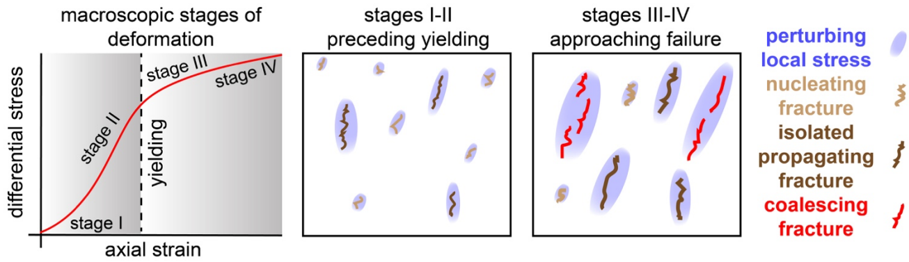
610 Figure 7: Schematic of varying modes of fracture development observed preceding yielding and approaching macroscopic failure. Nucleating, propagating, and coalescing fractures shown in light brown, dark brown and red, respectively. Blue ellipsoids show the 615 approximate extent of the perturbation of the local stress field produced by fracture network development. When the rock experiences lower differential stress and the fracture network is more distributed, 1) similar numbers of new fractures nucleate and preexisting fractures grow, 2) isolated propagation dominates coalescence, and 3) local stress perturbations do not appear to promote fracture growth. When the system approaches macroscopic failure, 1) preexisting fracture propagation dominates new fracture nucleation, 2) coalescence dominates isolated propagation in the experiments with the lowest confining stress and dry conditions, and 3) local stress perturbations promote fracture growth.
