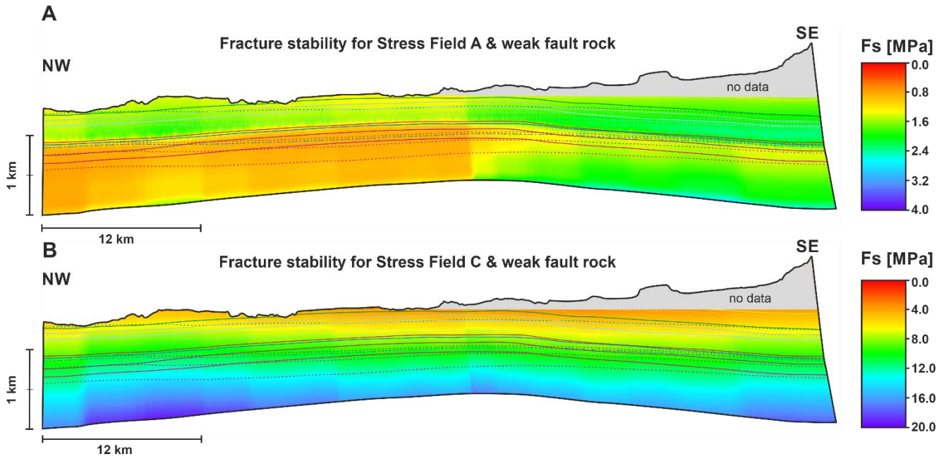
305 Figure 8: Fracture stability plotted onto the Coyote Wash Fault surface. (A) for stress field A and a low friction fault rock. (B) For stress field C and a low friction fault rock. Note the differences in the colour scale. F_s is more critical in the NW part of the fault for stress field A while F_s for stress field C is far from critical. Dashed lines represent hangingwall, straight line footwall cut-off lines, see Figure 5 for stratigraphic context.
