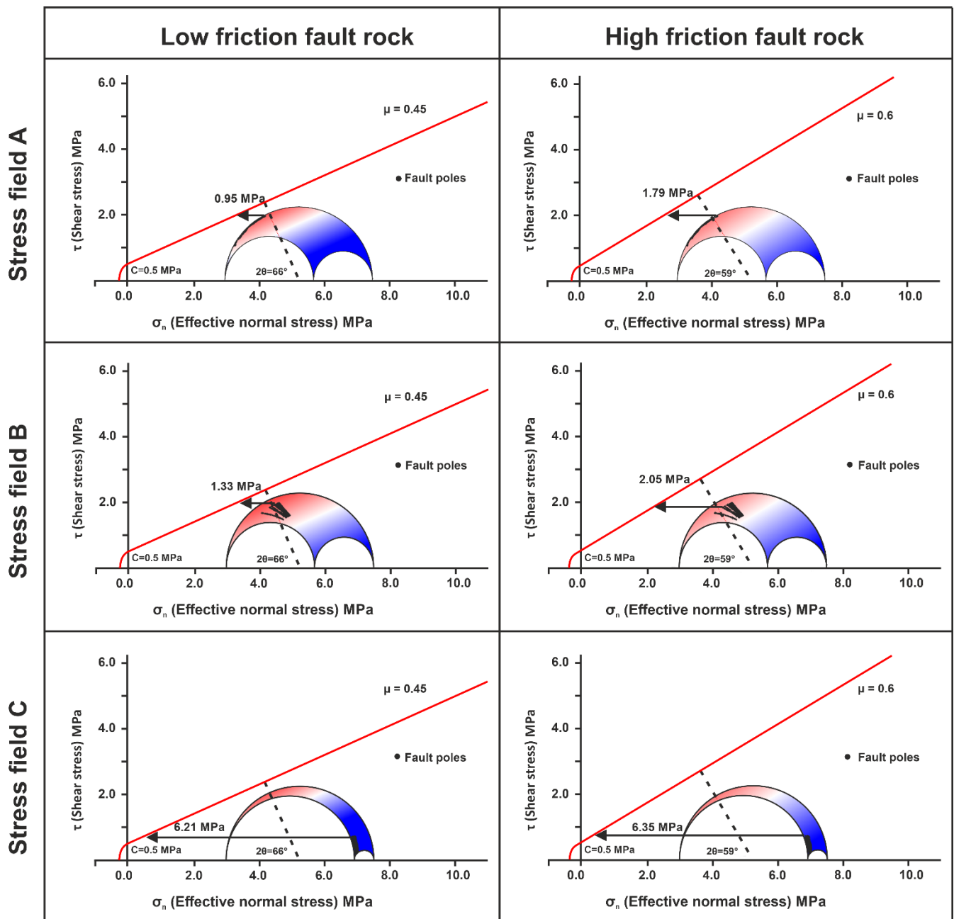
300 Figure 7: Mohr diagrams illustrating the fracture stability for the Coyote Wash Fault within the three stress fields for two types of fault rocks. Black arrows indicate the increase in pore-pressure needed to force the fault into failure. Number of fault poles in each plot is 3525.
