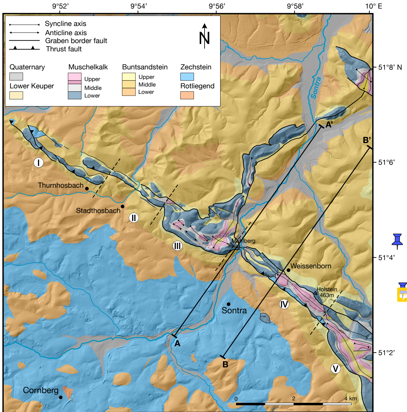
435 Figure 4 Geological map of the study area. Lines marked A-A' and B-B' indicate the position of the balanced cross sections in Fig. 6. Roman letters define sections of the graben between the dashed lines, which are referred to and further discussed in the text. DEM courtesy of Hessian Agency for Nature Conservation, Environment and Geology (HLNUG).
