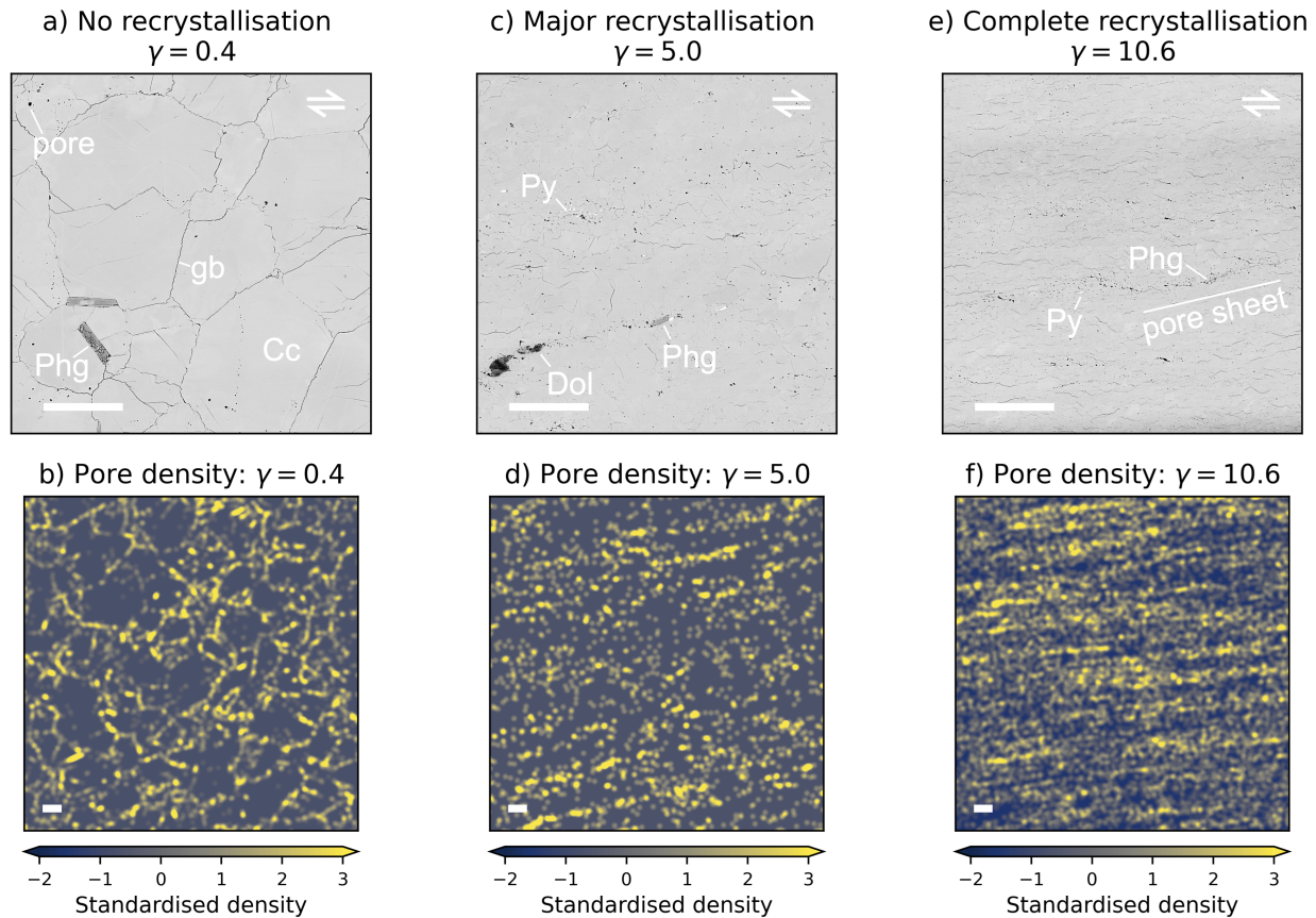
Figure 1. Microstructure and pore density in samples with increasing strain. The samples document the production of a mylonite through dynamic recrystallisation. Panels a,c and e are backscatter electron images while b, d and f are pore density maps. In all images the white scale bar is 100 \mu\text{m} . The pointed ends of the colour bars refer to the fact that some data values are larger than the max and min of the colour map. (Py = pyrite, Dol = dolomite, Phg = phengite, Cc = calcite, gb = grain boundary).
