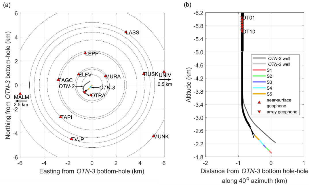
570 Figure 1. Seismic network used for monitoring the stimulation in 2018. (a) Map view showing the near-surface geophones framing the EGS site with the injection borehole OTN-3 and the OTN-2 well drilled in 2019 and 2020. Radius of concentric circles presents distance between the end of the OTN-3 borehole and each station. (b) Side view of the boreholes with the geophone-array placed at the already existing part of the OTN-2 well. The injection intervals S1-S5 of the stimulation in 2018 are color-coded at the end of the injection borehole. For further details about location of the EGS site at the suburban area of Helsinki in Finland see Kwiatek et al. (2019).
