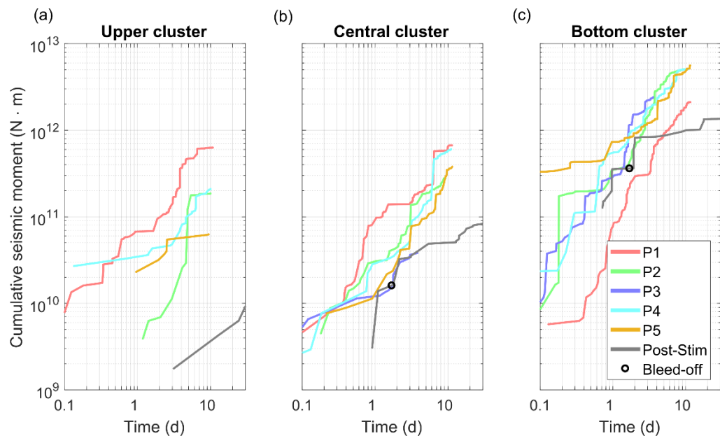
595 Figure 5. Temporal evolution of the cumulative seismic moment release with time for each of the three hypocenter clusters separately: (a) The uppermost hypocenter cluster, (b) the central hypocenter cluster and (c) the deepest and main hypocenter cluster.
