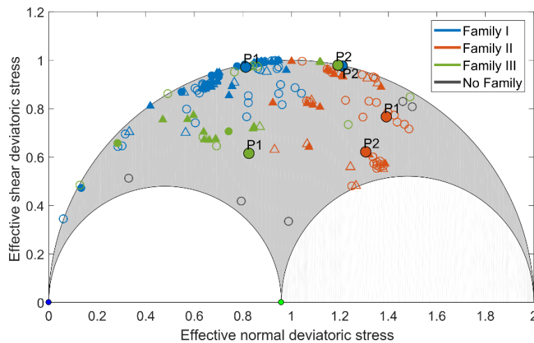
630 Figure 10. Deviatoric Mohr circle representing the local stress field with the fault plane solutions having the highest fault instability coefficient of the estimated focal mechanisms. A stress ratio of R = 0.53 was used for stress inversion. Events with M_w \geq 1 and M_w < 1 are plotted as triangles and circles, respectively. Filled and unfilled markers represent events with manually picked and estimated polarities, respectively. The mean and its auxiliary fault plane solution of each family are plotted as filled large dots labelled with P1 and P2, respectively. Most family I events (blue symbols) occurred on critically stressed faults.
