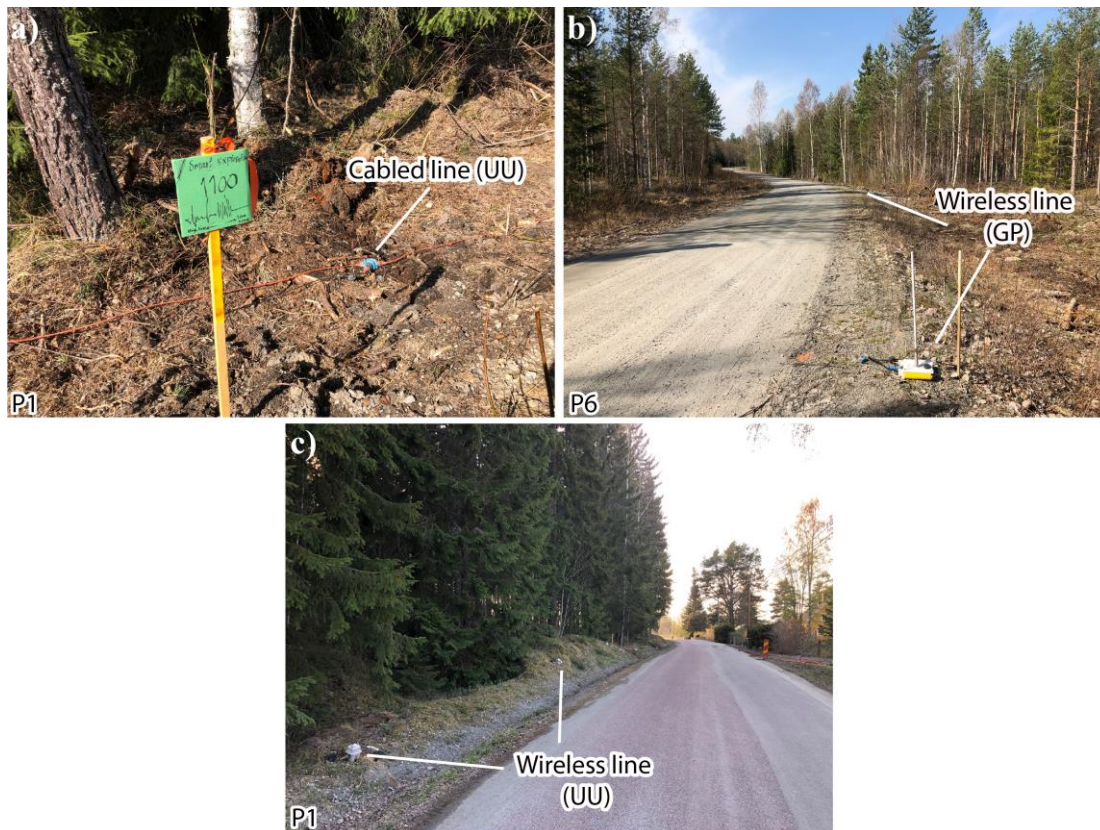
185 Figure 4. Field photos showing different seismic recorders used during the 3D survey. (a,c) With the exception of P1 and P3 where a Sercel recording system was used (cabled and wirelesses along P1 and only cabled along P3), (b) all other profiles were acquired using RT2 Wireless Seismic requiring a maximum distance of 50 m for data crosstalk and live data harvesting. The choice of the recorders was solely dictated by their availability to the research team. UU: Uppsala University; GP: Geopartner. Photos by Alireza Malehmir.
