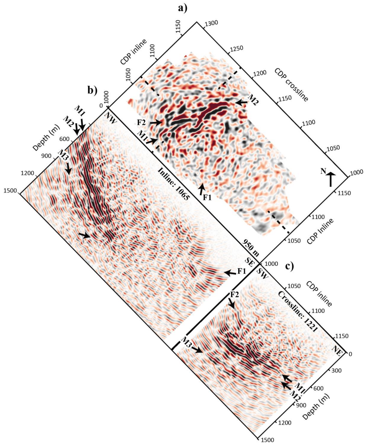
365 Figure 11. A series of slices (a) depth slice, (b) inline and (c) crossline through the migrated and time-to-depth converted stacked volume showing two major sets of southeast-dipping reflections (M1 and M2) terminated by a northwest-dipping one (F1). The crossline section shows these two sets of reflections have gentle but different dips towards the west. F2 reflection appears to submerge (downlap) with M1. In the footwall of M1 and M2, another submerging reflection (M3) appears although weaker.
