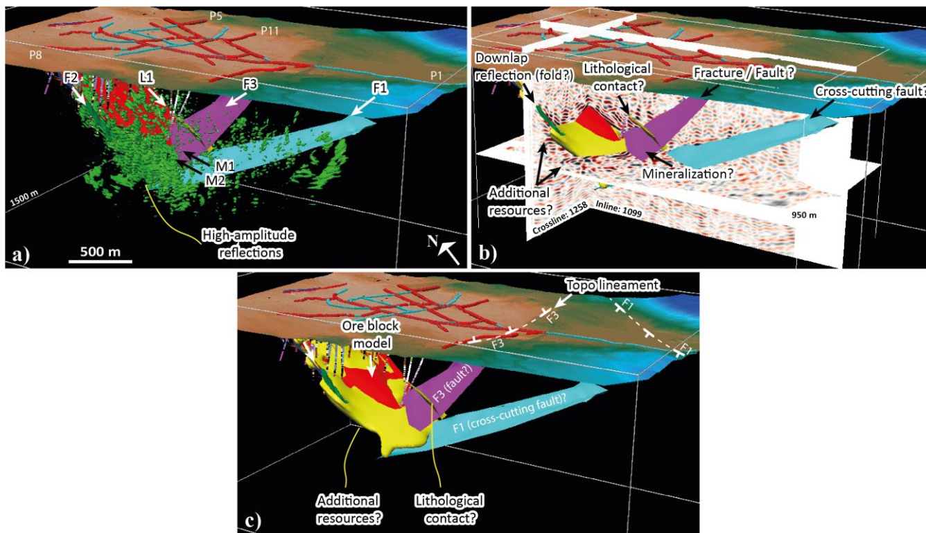
Figure 13. 3D views showing how additional potential resources were identified from the 3D seismic volume. (a) High-amplitude reflections were first extracted through a thresholding procedure as iso-shells (green shells) and then (b) matched with the boreholes intersecting the mineralization and merged with the ore block model to produce an updated resource model (yellow shell). (c) The refined resource model shows both lateral (to the west) and vertical extension (approximately of 300 m) than the ore block model from the available boreholes.
