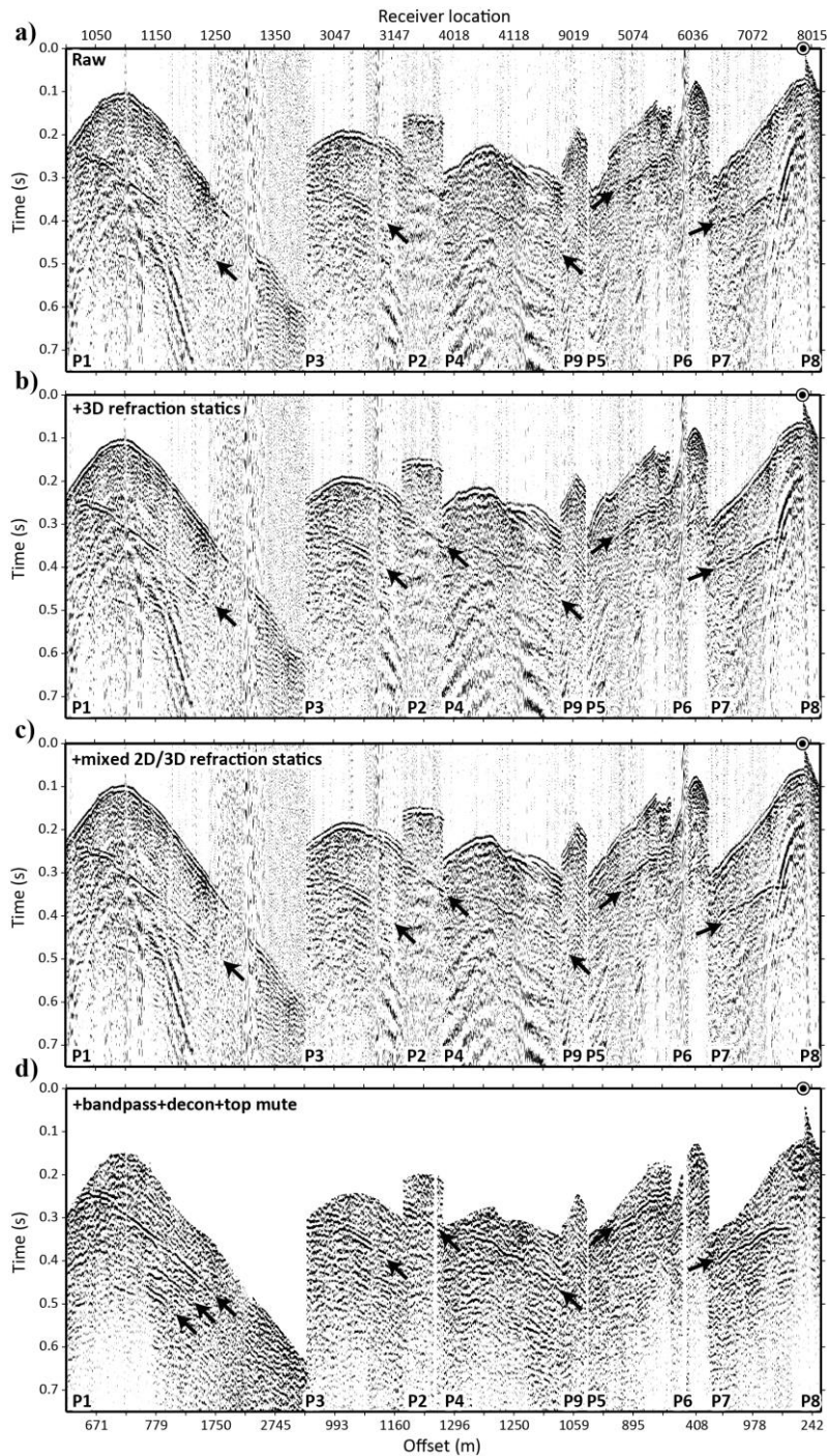
Figure 7. (a) An example of raw shot gather along P8 after (b) 3D static corrections, (c) mixed 2D and 3D static corrections (used for processing) and (d) bandpass filter, deconvolution (zero-phase or spectral whitening), and top-mute. Note the increase in the signal quality in and especially coherency of the reflections marked using the arrows (we expect these to be from the mineralization from the earlier 2D surveys and downhole logging data).
