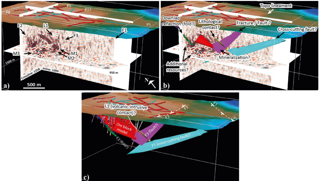
Figure 12. 3D views from the migrated and time-to-depth converted stacked volume showing (a) a series of strong southeast-dipping reflections (e.g., M1 and M2) and a number of northwest dipping ones (e.g., F1 and F2) and how (b) they have been picked to represent various surfaces within the volume. The red surface is the ore block model derived from borehole data. (c) F1-F3 are interpreted to be either from fault and fracture systems or from folds. Note also how F1 and F3 may be correlated with the topographic lineaments observed on the LiDAR data. Reflection L1 is interpreted to be from the contact between volcanic and intrusive rocks.
