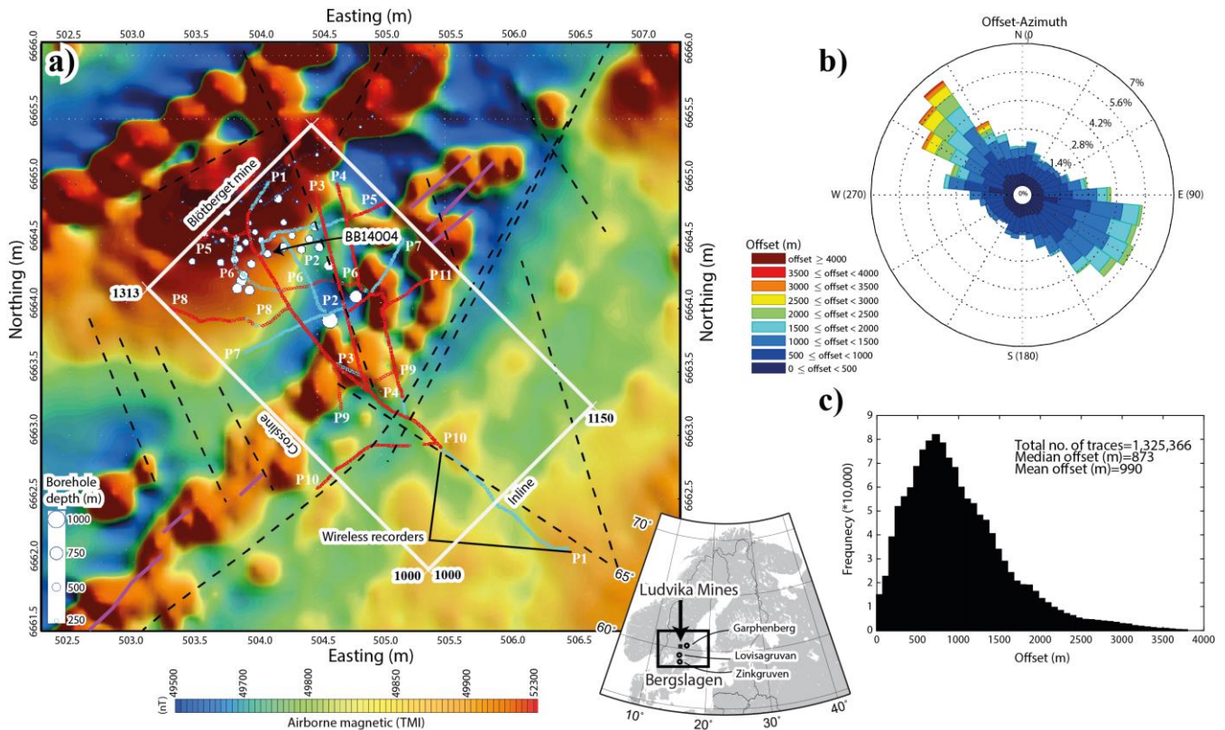
105 Figure 1. (a) Total-field aeromagnetic map of the Blötberget mine in central Sweden, and the sparse 3D seismic survey area. P1-P11 were 110 setup as part of the survey (fixed geometry). The red dots show the shot locations (1056 points) and blue dots are the receiver locations (1266 points). P10 and P11 were added later to improve fold and azimuth coverage and comprise only shots. Along P1 several collocated 2D profiles have since 2015 been acquired (landstreamer survey in 2015 and conventional plant-type geophones in 2016). Downhole logging data from BB14004 is presented in this study. (b) Offset-azimuth coverage showing a narrow azimuth survey setup for primarily targeting the known southeast dipping of the iron-oxide deposits and (c) offset distribution showing a median offset of approximately 900 m for the whole dataset. Magnetic data were provided by the Geological Survey of Sweden. Dashed lines in (a) are topographic and structural lineaments extracted from the geological map of the study area. Purple solid lines are interpreted dykes.
