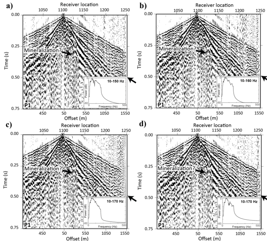
225 Figure 6. Shot gathers (after cross-correlation) and their corresponding amplitude spectra along cabled part of P1 showing sweep parameter tests (a) 10-150 Hz, 60% force and 17 s sweep length, (b) 10-160 Hz, 60% force and 17 s sweep length, (c) 10-170 Hz, 60% force and 20 s sweep length, and (d) 10-170 Hz, 70% force and 20 s sweep length. Both higher end frequencies of 160 and 170 Hz were judged suitable however we decided to choose 160 Hz because it produced less ground-roll energy compared to 170 Hz. The arrow shows expected reflection from the mineralization also judged for choosing the sweep parameters.
