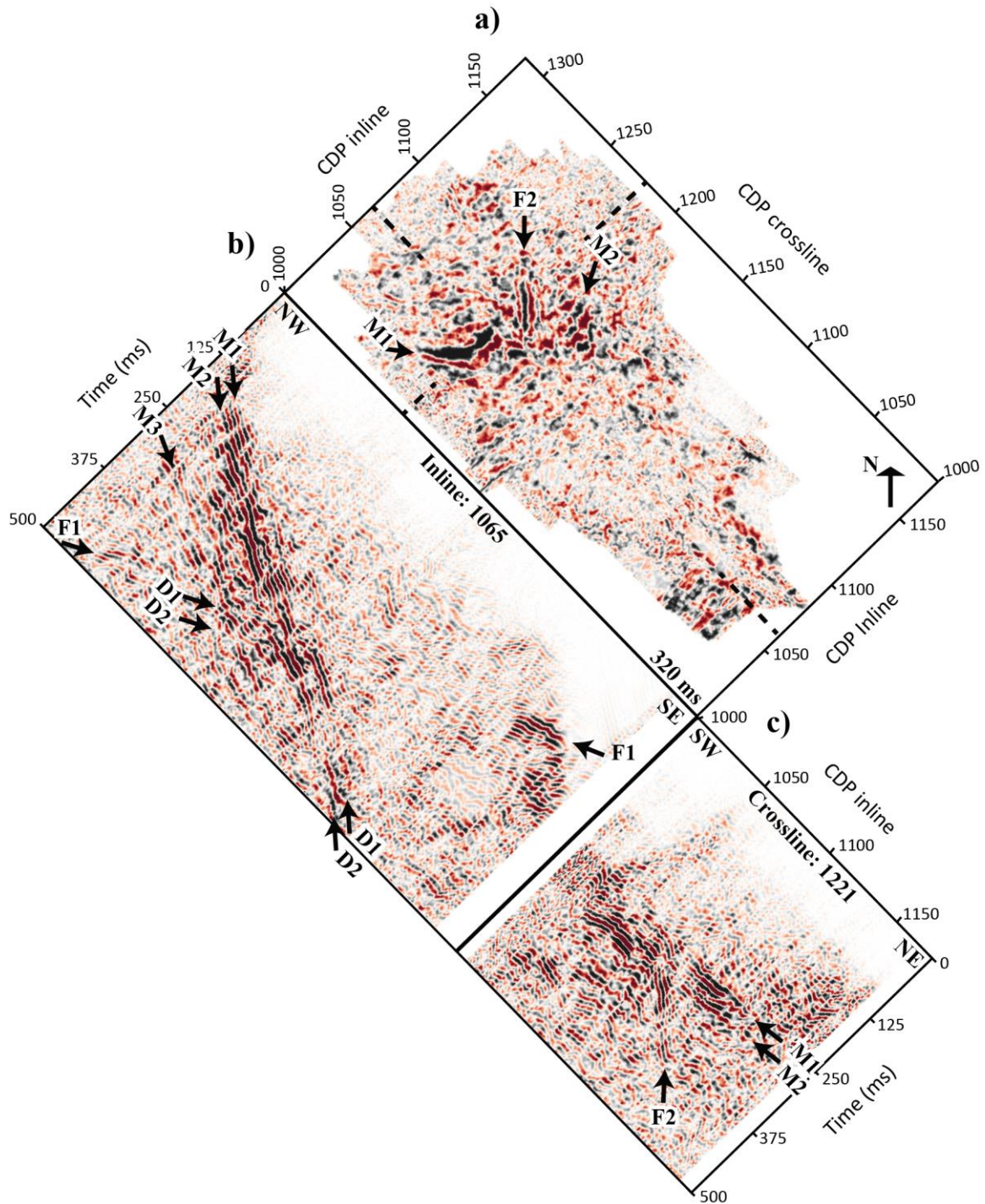
360 Figure 10. A series of slices (a) timeslice, (b) inline and (c) crossline through the unmigrated stacked volume showing two major sets of southeast-dipping reflections (M1 and M2) terminated by a northwest-dipping one (F1) at where two sets of diffractions (D1 and D2) are present at the intersection between F1 and M1 and M2 reflections. The crossline section shows these two sets of reflections have gentle but different dips towards the west. A reflection (F2) appears to cut through these two sets.
