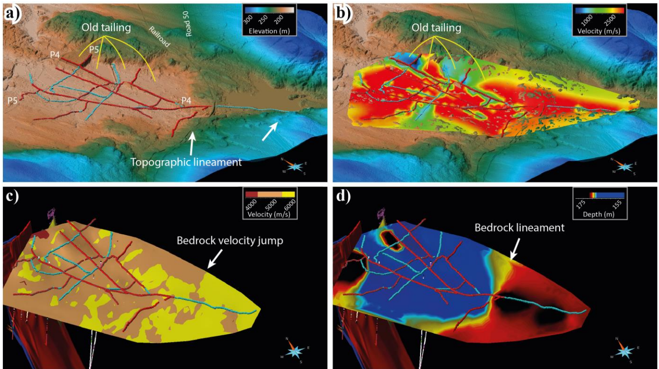
325 Figure 9. (a) LiDAR elevation map of a portion of the 3D survey area showing built-up roads and a historical tailing where P4 and P5 were 330 positioned. (b) Near-surface velocities derived from the 3D refraction static solution showing the clear position of the tailing as low-velocity 335 materials and the two separate ponds immediately south of it. (c) Bedrock velocities and a sharp jump in the velocity south of the survey 340 area and (d) bedrock level from the 3D refraction static solution showing a clear lineament (higher ground) immediately south of the road 50 (and the railroad). We attribute the bedrock lineament to a (or set of) normal fault.
