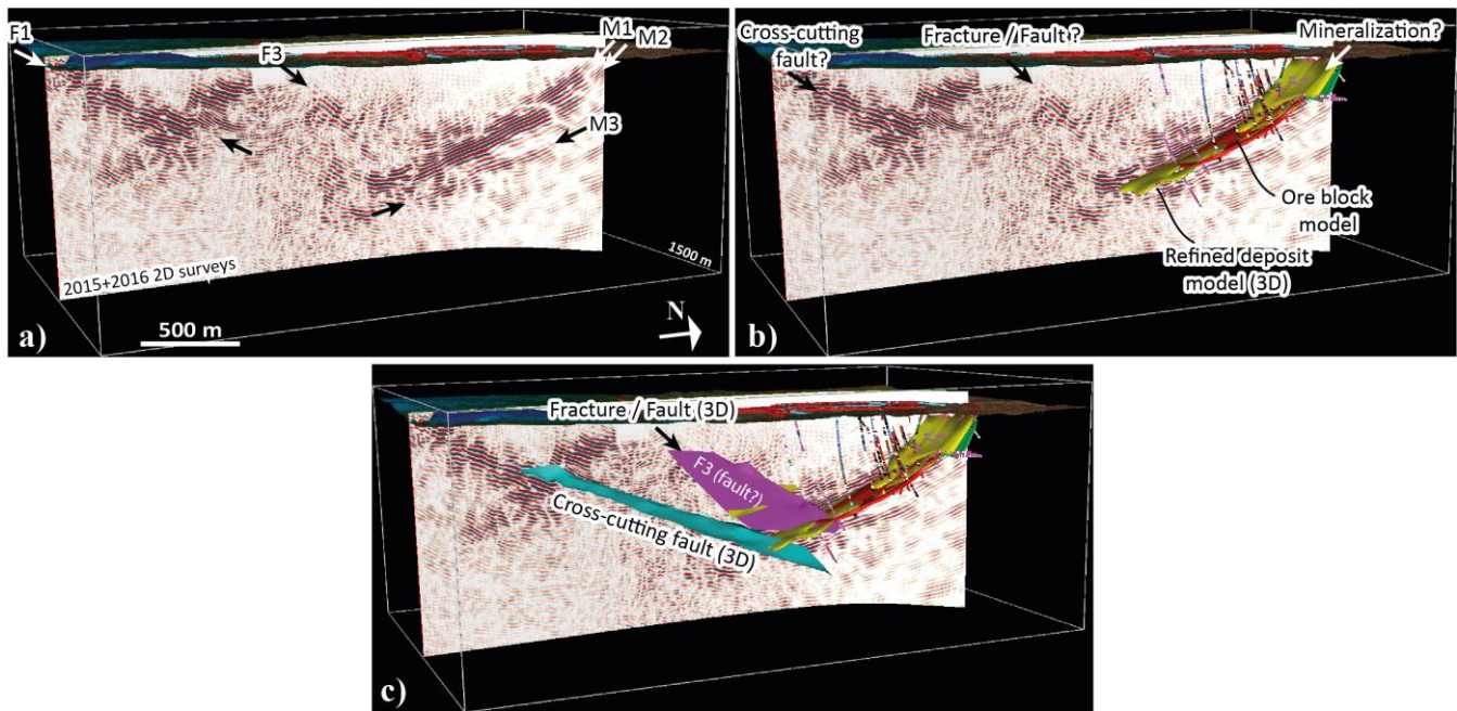
Figure 14. 3D views from (a) the earlier 2D surveys (Markovic et al., 2020) and (b) interpretation of the main features in the 2D profile (along P1 of the 3D survey) and (c) how various features extracted from the 3D volume manifest themselves in this 2D profile result. In particular, note that the F1 and M3 are better defined in the 3D volume (Figs. 12 and 13) showing a westward plunge for F1 and a submerging character for M3 implying they have a major out-of-the-plane nature in the 2D profile.
