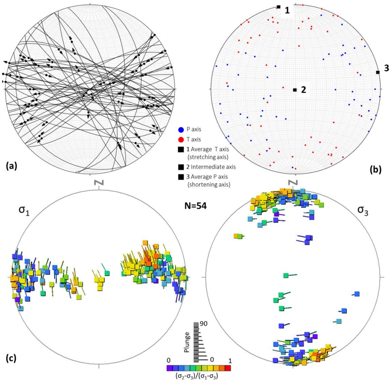
635 Figure 10: (a) Lower-hemisphere, equal-area projection of the 54 fault planes with kinematic information, showing also the slickenline attitudes and the sense of movement. (b) Results of the kinematic analysis for the fault planes shown in (a). P = pressure, T = tension. (c) Results of the dynamic analysis for the fault planes shown in (a). Colors represent the \Phi value calculated for each stress tensor.
