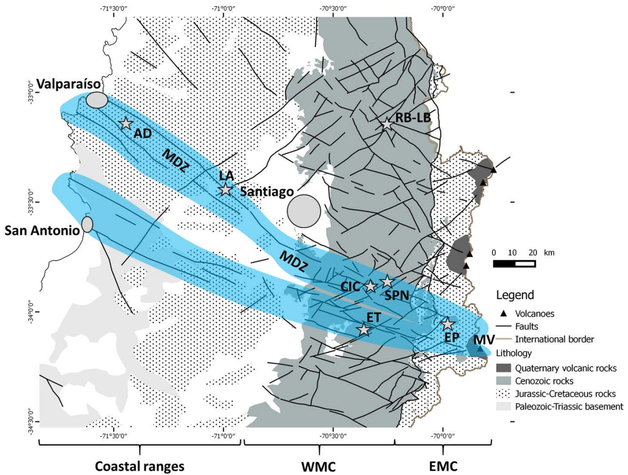
Figure 167: Continental-scale expression of the Maipo deformation zone (MDZ), highlighted in light blue; the PFS correspond to its manifestation in the Cenozoic rocks of the Western Main Cordillera. Background geology from SERNAGEOMIN (2002); faults in the Western Main Cordillera from Piquer et al. (2016). RB-LB = Río Blanco-Los Bronces; ET = El Teniente; EP = Escalones prospect; SPN = San Pedro de Nolasco veins; CIC = Carlota Intrusive Complex; LA = Lo Aguirre stratabound deposit; AD = Antena District of orogenic Au veins; MV = Maipo Volcano; WMC = Western Main Cordillera; EMC = Eastern Main Cordillera. The main cities of Santiago and Valparaíso are also shown.
