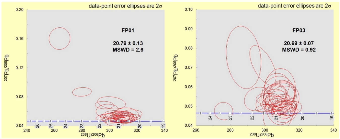
620 Figure 6: Tera-Wasserburg plots for the two U-Pb analyses completed for this study. Numbers on the reference concordia traces are millions of years.
