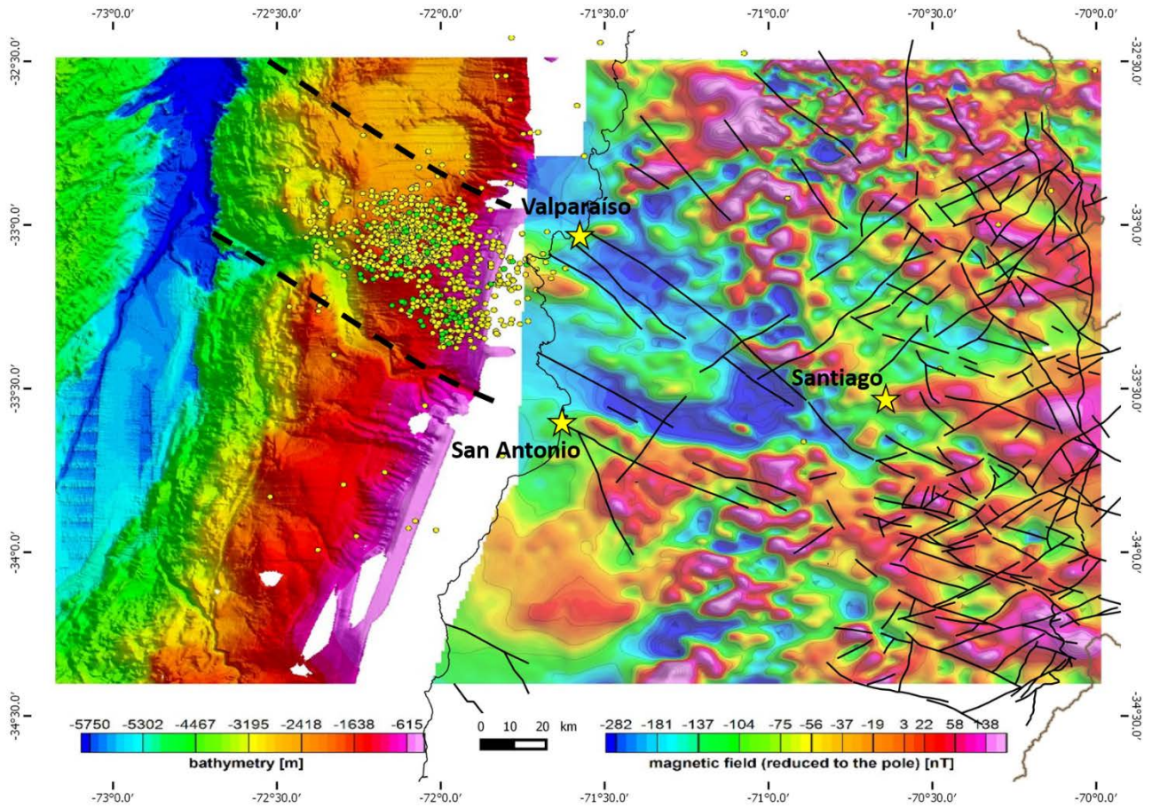
Figure 178: Geophysical expressions of the PFS, the Maipo Deformation Zone and the Teniente-San Antonio fault system. The submarine continental shelf is colored according to its bathymetry (Weinrebe and Hasert, 2012); thick dashed lines represent the possible submarine prolongation of the two main branches of the MDZ. Colors in the continent correspond to RTP aeromagnetic map (SERNAGEOMIN, 1980). Yellow and green small circles show the location of earthquake hypocenters related to the 2017 Valparaíso sequence (yellow data set extracted from CSN data repository, green data set, relocated events from Nealy et al 2017, data repository). The Chile-Argentina international boundary, the coastline and fault architecture from Fig. 17 Fig. 16 are also shown.
