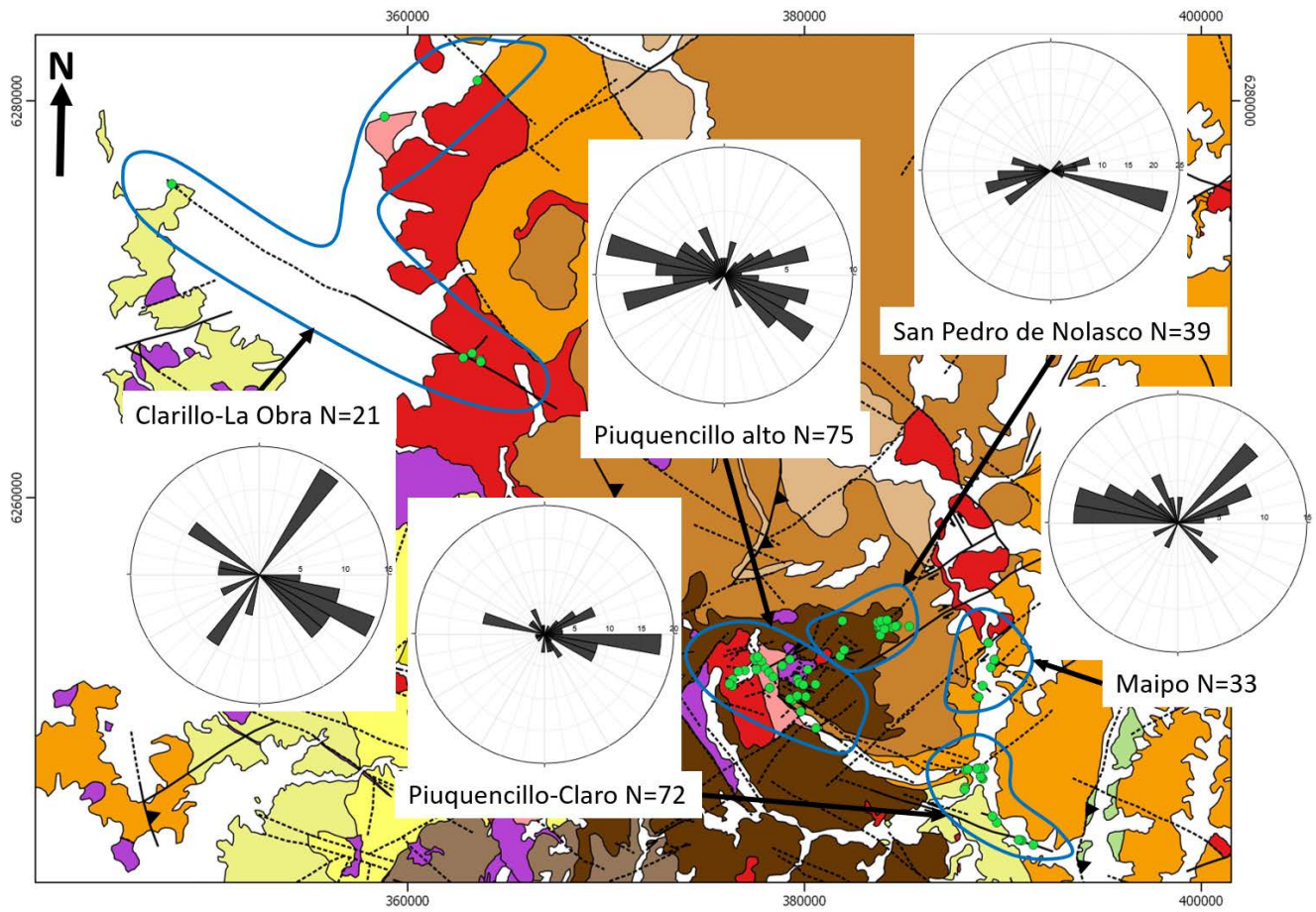
630 Figure 9: Preferred orientations of fault planes in the five sectors into which the study area was subdivided. Geological map on the background as in Figure 5.
