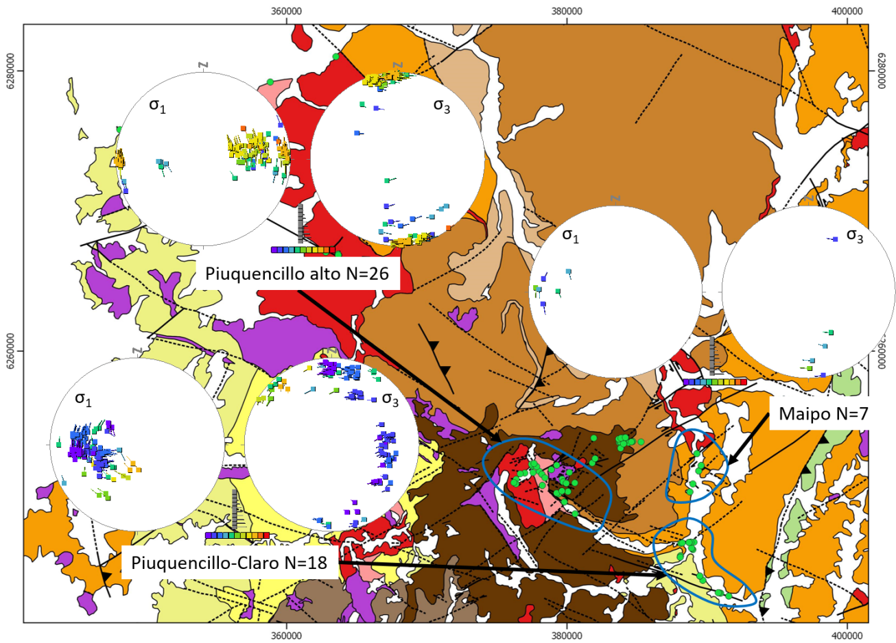
645 Figure 13: Dynamic analysis of fault plane data by sector. Clarillo-La Obra and San Pedro de Nolasco sectors are not considered, as the minimum of four fault planes with reliable kinematic indicators, necessary for stress state calculations, was not achieved in these areas. Geological map on the background as in Figure 5.
