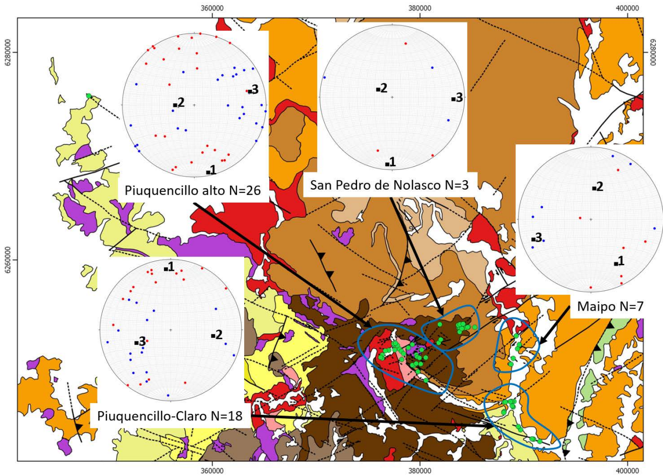
Figure 12: Kinematic analysis of fault plane data by sector. Clarillo-La Obra sector is not considered, as no reliable kinematic indicators were found. Geological map on the background as in Figure 5.
