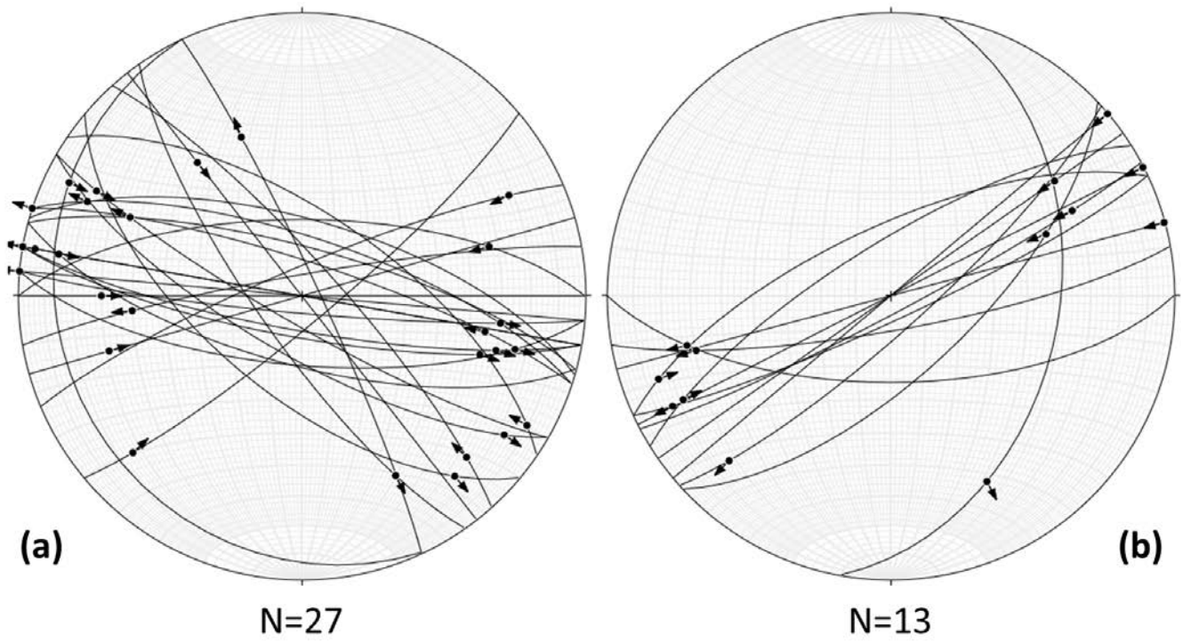
Figure 156: (a) Lower-hemisphere, equal-area projection of fault planes with a sinistral strike-slip component and striations with pitch \leq 45^\circ . (b) Same as in (a) but for fault planes with a dextral slip.
