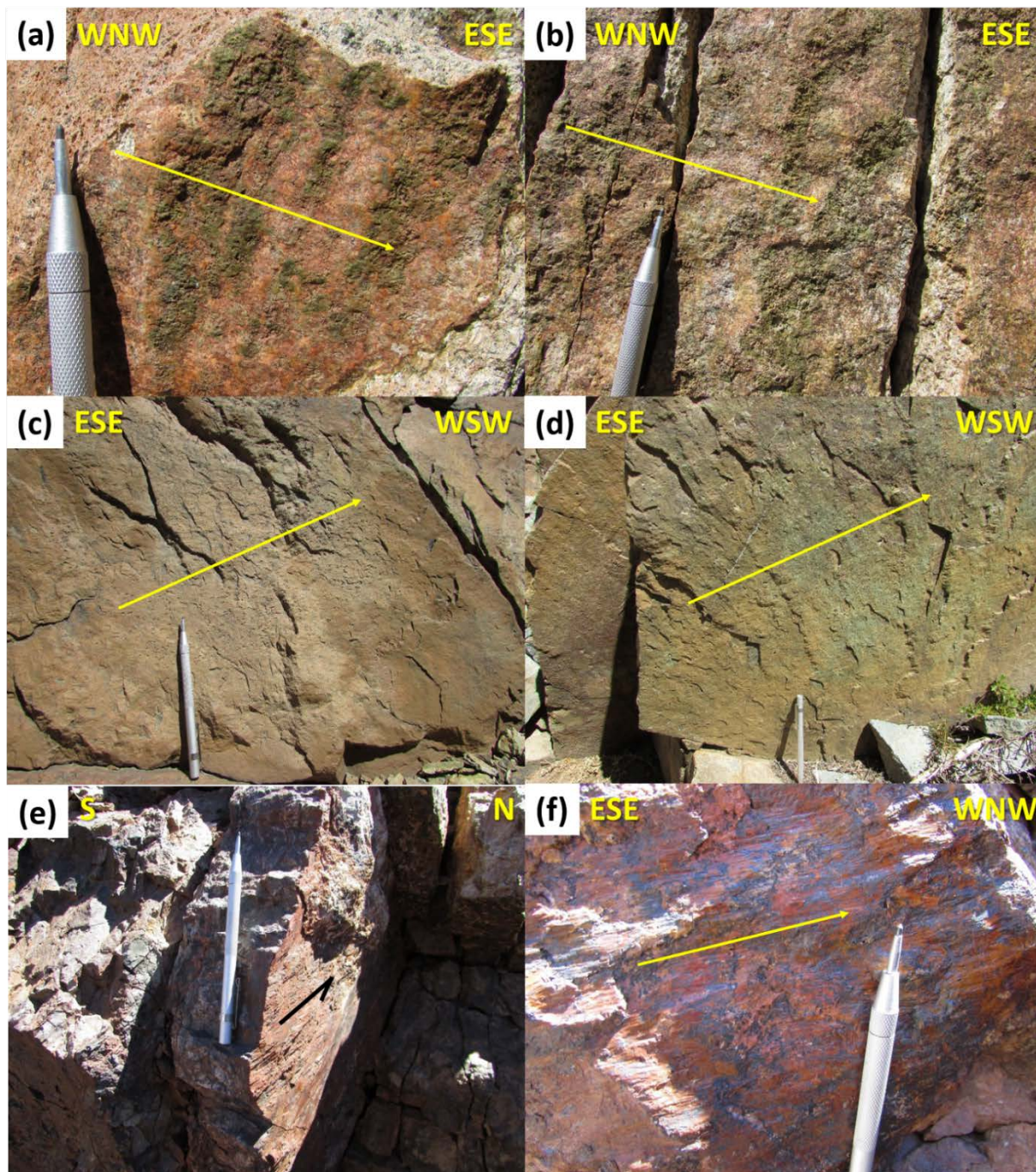
610 Figure 4: Fault planes in different branches of the PFS. All of them show evidences of sinistral strike-slip movements. Arrows indicate the sense of movement of the missing block. (a) and (b) correspond to fault planes affecting the Miocene plutons of the Carlota Intrusive Complex, with syn-tectonic epidote (a) and actinolite (b) forming steps and crystallizing in strain fringes. (c) and (d) correspond to fault planes affecting volcanic rocks of the Teniente Volcanic Complex, with sense of movement indicated by RM criteria (Petit, 1987). (e) and (f) illustrate the syn-tectonic, quartz-barite-calcite-hematite San Pedro de Nolasco veins, with the sense of movement indicated by steps in quartz and hematite.
