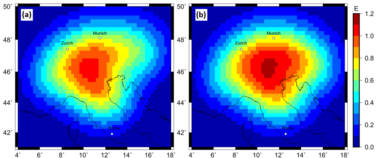
Figure 15 Forward calculated gzz gravity signal at a station height of 225 km from predefined sub-crustal slab geometries with a content density contrast of 60 \text{ kg/m}^3 and a constant thickness of 80 km. (a) slab configuration of hypothesis 1 (b) slab configuration of hypothesis 2.
