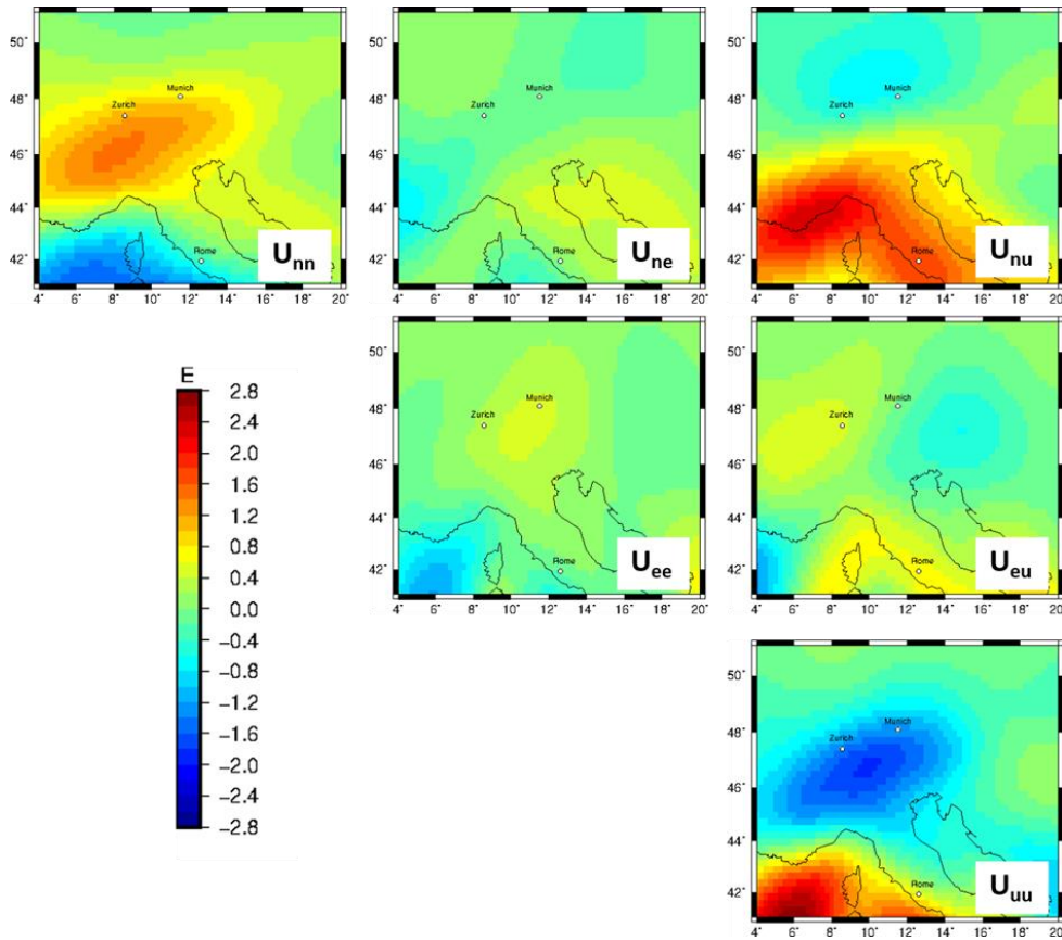
Figure 13 GOCE gradients at 225 km height after Bouman et al. (2016) corrected for topography and bathymetry with a 5° extension to remove far field effects. The gravity gradients are presented in a North-East-Up coordinate system.
