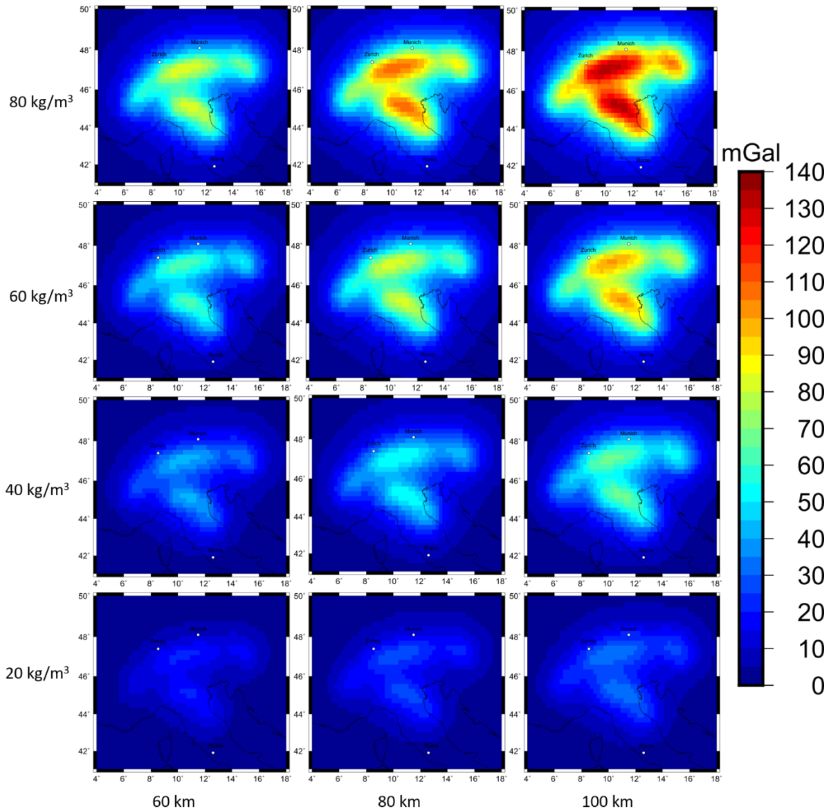
Figure 7 Forward calculated gravity disturbance signal for 12 different combination of density contrast and slab thickness for sub-crustal slab configuration 1 at a station height of 6040 m.
