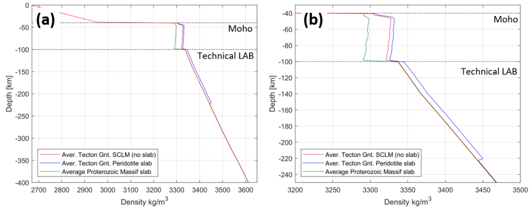
Figure 9 (a) density profile at 11° longitude and 45° latitude for the full vertical model space of 400 km depth. Density profiles for 3 different models ( M_0 , M_1 , M_9 ) with different compositional properties are shown. (b) Zoomed in profile at the depth range of present slab segments.
