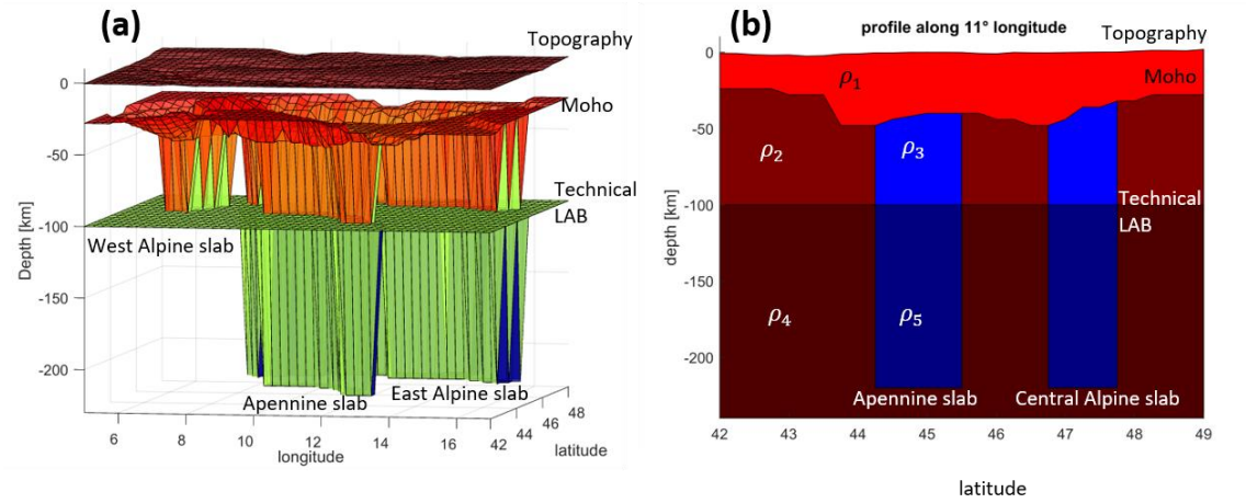
Figure 8 (a) 3D model set up using LitMod 3D. Topography, Moho and LAB depth as well as the vertical incorporated slab models are used as input layers with assigned petrophysical and thermal properties. (b) Profile along 11° longitude through a LitMod model containing Topography, crustal and lithospheric thickness as well as a slab segment. \rho_{01-5} indicate petrophysical and thermal property variations for each layer.
