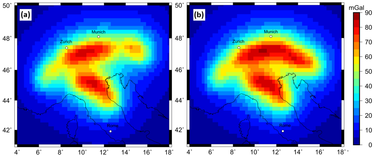
Figure 6 Forward calculated gravity disturbance signal at a station height of 6040 m for predefined sub-crustal slab geometries with a content density contrast of 60 \text{ kg/m}^3 and a constant thickness of 80 km. (a) predefined slab configuration 1 (b) predefined slab configuration 2.
