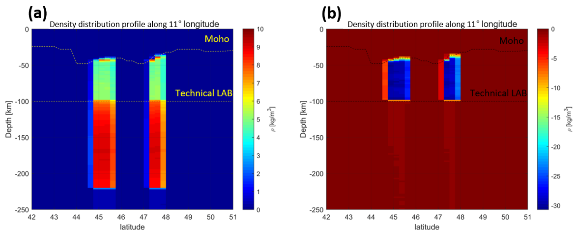
Figure 10 (a) residual density contrast for lithospheric and sub lithospheric slab segments of model ( M_3 ) with Tecton like composition within the lithosphere and PUM and DMM composition in the sub lithosphere with an additional thermal anomaly of -100^\circ \text{ K} for the sub lithospheric slab segment to the background model ( M_0 ). (b) Residual lithospheric density contrast of a Proterozoic lithospheric slab segment ( M_8 ) to a Tecton compositional surrounding mantle ( M_0 ). Residual density contrast is limited to the technical LAB as the sub-lithospheric part is identical to the reference model (see also Fig. 9b)
