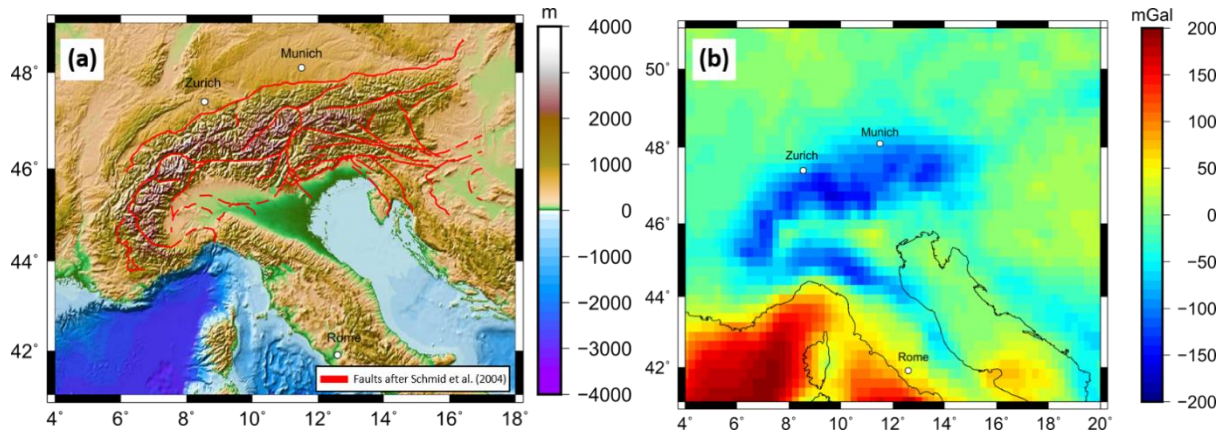
Figure 1 (a) Topography from ETOPO1 from Amante and Eakins (2009). Faults in red after Schmid et al. (2004). (b) Bouguer Anomaly based on XGM 2019 (Zingerle et al., 2020) with a maximum spherical harmonics degree of 719 at a station height of 6040m above the ellipsoid, just above the surface of the Alps. Correction density for rock: 2670 kg/m 3 and for water: 1030 kg/m 3
