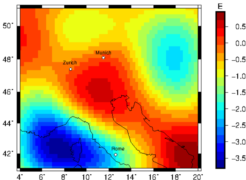
Figure 14 Forward calculated gzz gravity signal from relative density distribution converted from relative seismic velocities using a conversion factor of 0.3 for the at 225 km station height.
