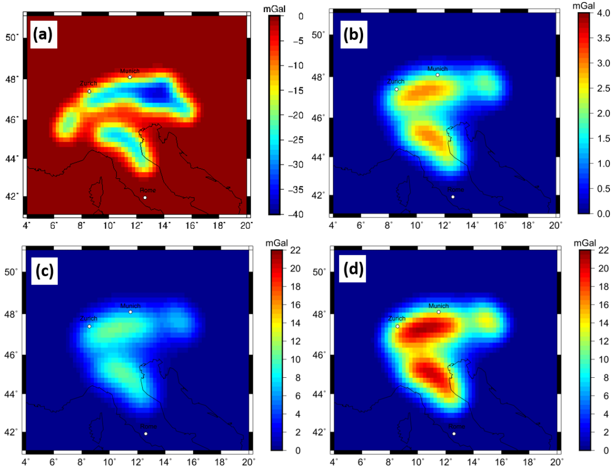
Figure 12 (a) Forward calculated gravity effect of a Proterozoic lithospheric slab segment to a Tecton compositional surrounding mantle for configuration 2, obtained by calculating the residual between M_8 and M_0 . (b) gravity signal produced by purely compositional effect in the sub lithosphere between a PUM and DMM composition, obtained by calculating the residual between M_5 and M_6 . (c) gravity signal produced by purely thermal anomaly of -100^\circ\text{K} for a sub lithospheric slab segment, obtain by calculating the residual between M_3 and M_6 . (d) gravity signal produced by purely thermal anomaly of -200^\circ\text{K} for a sub lithospheric slab segment obtained by calculating the residual between M_6 and M_7 .
