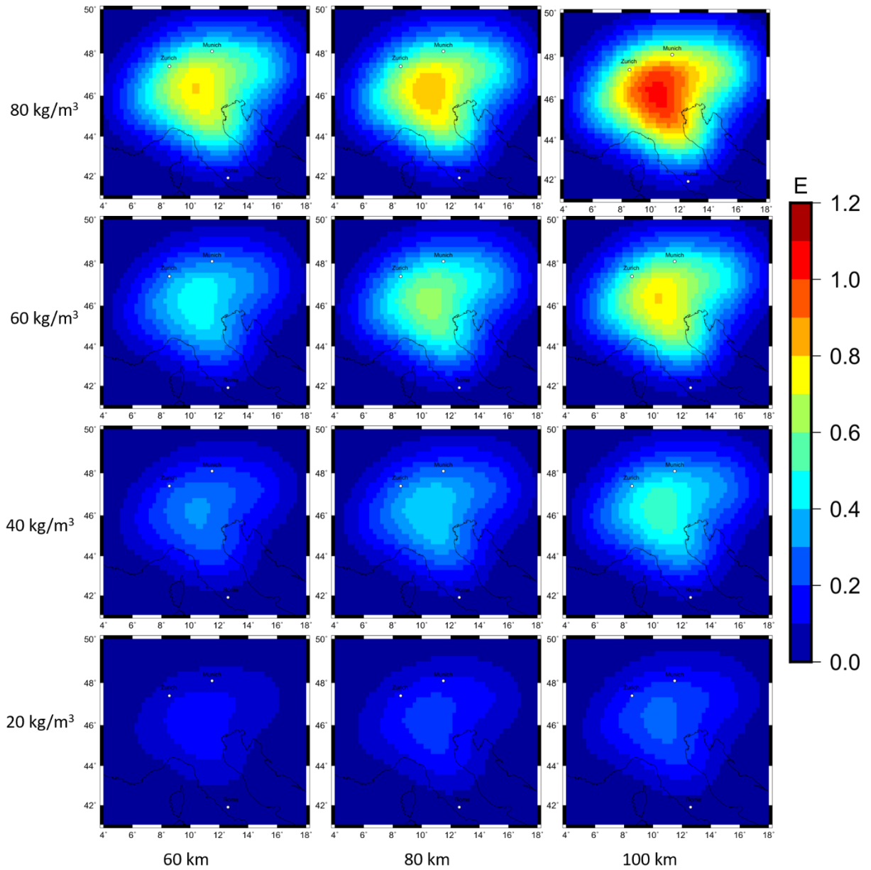
Figure 16 Forward calculated gzz gravity signal for 12 different combination of density contrast and slab thickness at a station height of 225 km for sub-crustal slab configuration 1.
