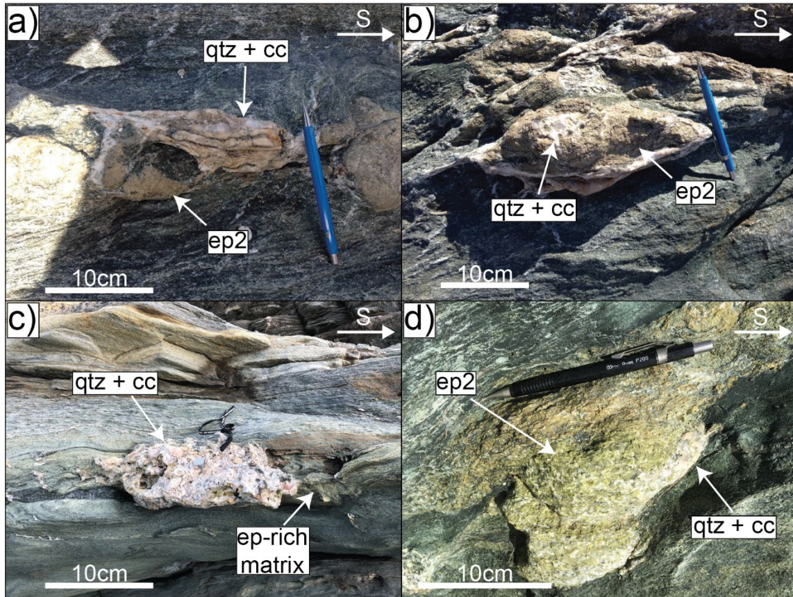
881 Figure 3. Outcrop photos of epidote boudins sampled for oxygen isotope thermometry. a) SY1613 (Lotos), b) SY1617 (Delfini), c) 882 SY1618 (Delfini), d) SY1623 (Delfini). Boudins formed during D 2 , parallel to F 2 fold hinge lines.
