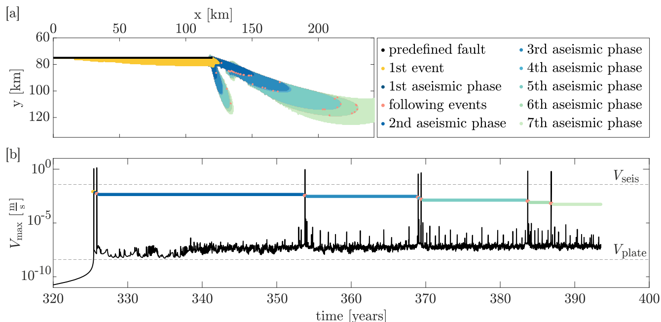
Figure 5. Temporal and spatial evolution of model RT with indication of aseismic and seismic fault growth stages in color. [a]: Accumulated plastic strain exceeding \epsilon_p > 4e-5 for different growth stages. [b]: Logarithm of the global maximum slip velocity \log(V_{max}) . A video of the simulation can be found in the online material link to video model RT, 1.1 Gb
