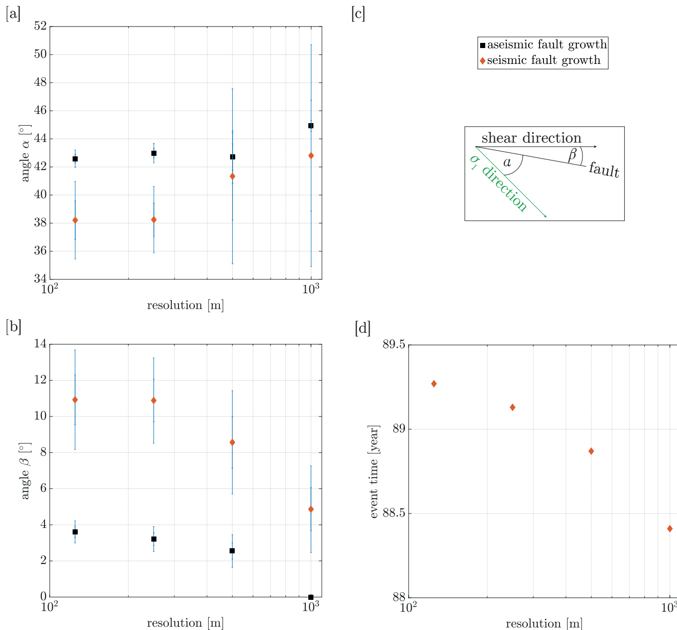
Figure A1. Convergence analysis of fault angle and earthquake time as relation between grid resolution and fault angles and grid resolution and earthquake time start, respectively. Analysis is showing that all seismic and aseismic fault angles as well as earthquake timing converge with grid size. Color-filled symbols indicate different faulting stages. Blue errorbars correspond to errors in measuring the absolute angle \beta and to spatial variations of the \sigma_1 -direction at the fault tip (details are explained in Preuss et al. (2019)). The solid line corresponds to the standard deviation [-1\sigma, 1\sigma] , the dashed line to the standard deviation [-2\sigma, 2\sigma] . [a]: Grid resolution in meter versus relative fault angle \alpha = \sigma_1 - \beta (see schematic illustration in [c]). [b]: Grid resolution in meter versus absolute fault angle \beta . [c]: Fault angle legend and schematic illustration of fault angles. [d]: Grid resolution in meter versus temporal onset of the earthquake in years.
