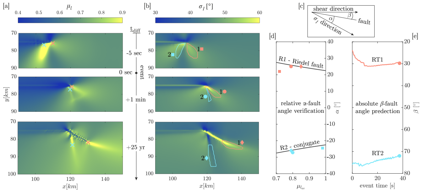
Figure 4. Evolution of friction coefficient and stress orientation over time and prediction of the absolute fault angle. 3 different times are: 1) Five seconds before fault extension (symbol ■), 2) One minute after the initiation of the first fault extension (symbol ●), and 3) 25 years after the initial fault extension (symbol ◆). Red color represents the Coulomb angle of R1 and turquoise refers to the conjugate fault R2. [a]: Snapshot zooms of the local friction distribution \mu_l at different times. Crosses indicate the location of the two maxima of \mu_l at the rupture tip or at the tip of the newly formed fault, respectively. [b]: Snapshot zooms of the distribution of the maximum compressive stress orientation \sigma_1 at different times. Red and turquoise polygons indicate the locations around the frictional maxima inside the two stress lobes where \mu_l and \sigma_1 are sampled and averaged according to two standard deviations of the mean (95th percentile). [c]: Schematic geometrical relation in physical space between horizontal shear direction, \sigma_1 -direction and forming fault. \beta represents the absolute fault angle, \alpha is the angle between fault and \sigma_1 -direction, such that \alpha_{1,2} = \sigma_1 - \beta_{1,2} . [d]: Relation between averaged friction \mu_{l,av} and fault angle \alpha_{1,2} , which is obtained from the average \sigma_1 -directions for the three different instants shown in [a] and [b] for R1 and R2, respectively. The values from the frontal lobe result in the data converging on the R1-Riedel angle \alpha_1 , the data from the back lobe converge on the R2-conjugate \alpha_2 . Black lines indicate the theoretical angle given by equation 16. [e]: Prediction of the absolute fault angles \beta_{1,2} for both RT1 and RT2 from sampling averages of \mu_l and \sigma_1 during the entire first dynamic earthquake.
