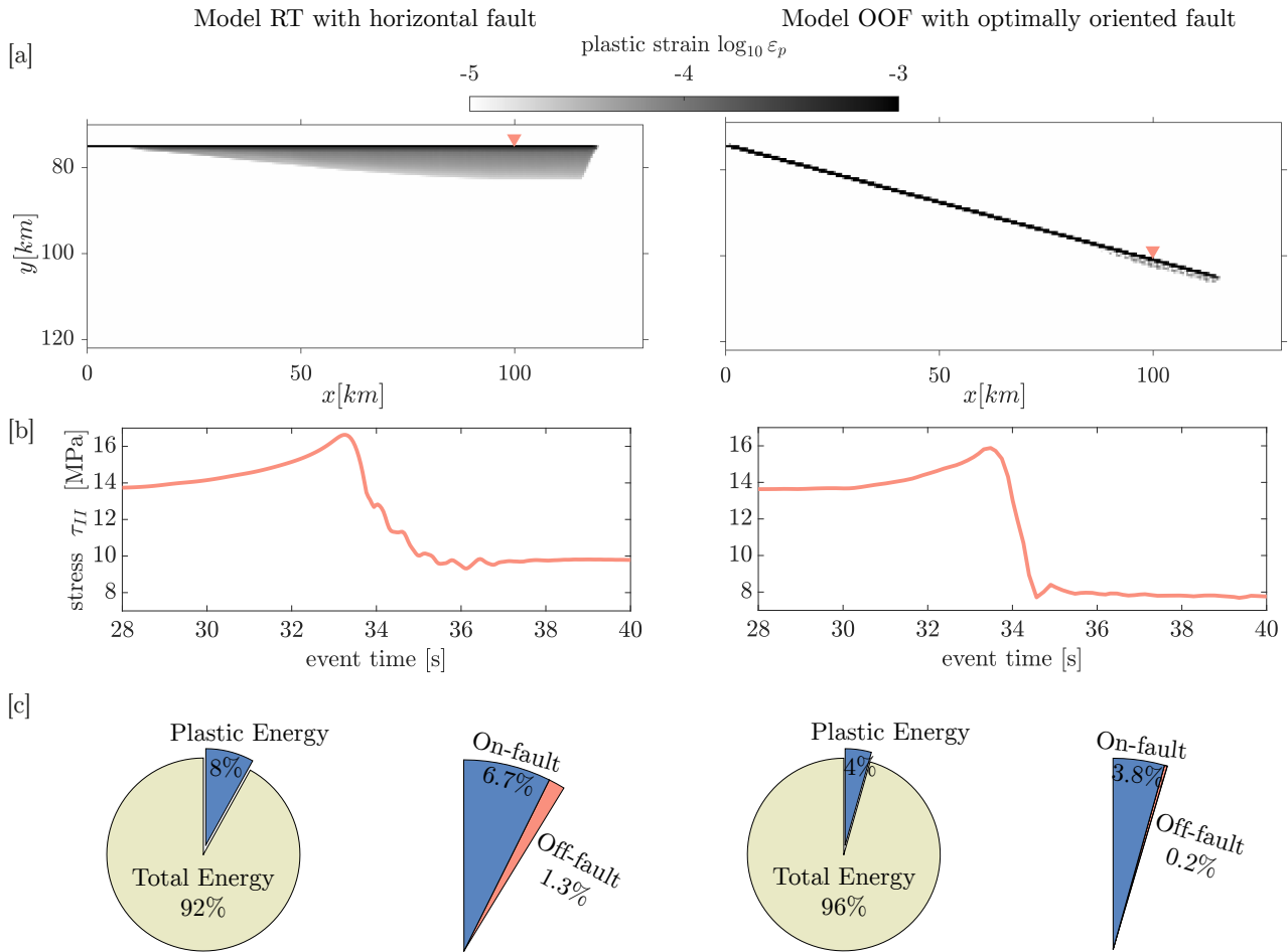
Figure 8. Comparison of plastic off-fault strain and energy between model RT and OOF. [a]: Accumulated plastic off-fault strain for both models in gray-scale during the first earthquake. Red triangles indicate the sample location of the stress data plotted in [b]. Panel [c] shows the ratio of the plastic energy opposed to the total energy in percentage. The plastic energy is subdivided in an on-fault (blue) and an off-fault (red) part.
