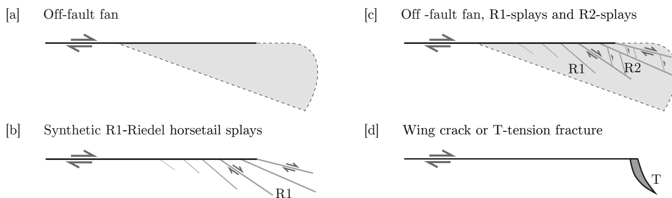
Figure 1. Fault structures developing at the tip of a sliding strike-slip fault. Modified from (Kim et al., 2004) and combined with schematic interpretations from (Faulkner et al., 2011) and (Perrin et al., 2016b). R1 = synthetic Riedel shear fracture, R2 = antithetic conjugate Riedel shear fracture and T = tension fracture or wing crack.
