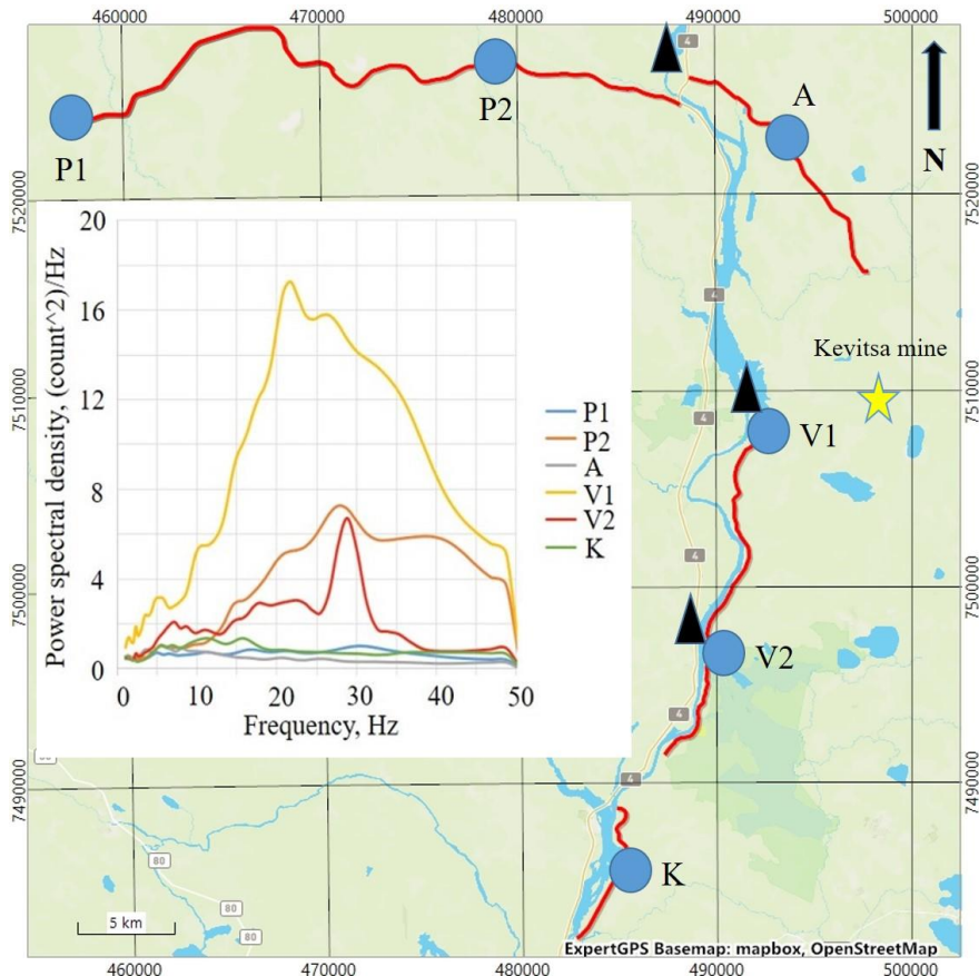
495 Figure 2: Illustration of noise level at six stations located in different profiles of the XSoDEx experiment. Position of strong noise sources (Keyitsa mine (yellow star) and dams of waterpower stations (black triangles)) and seismic stations selected for analysis (blue circles) are indicated. Brown and white Yellow lines show roads. Inset figure shows comparison of ambient noise power spectral density estimated at selected stations.
