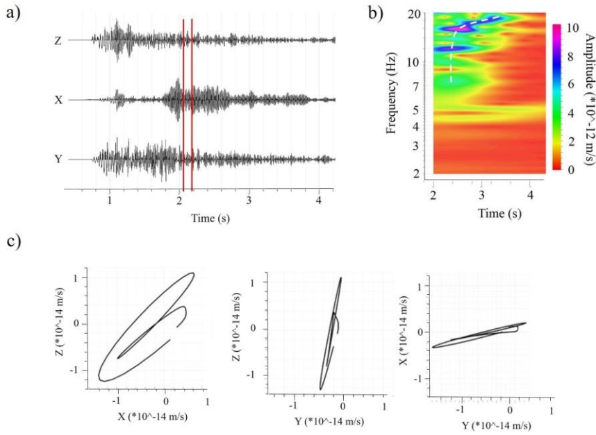
Figure 5: Result of analysis of scattered arrivals in synthetic seismograms with apparent velocity of 2100 -2500 m/s for frequencies 2-20 Hz (Fig. 4): a) 3C seismogram for synthetic receiver located at distance of 2000 m from the source (Fig. 4); b) spectrogram of the scattered arrival, recorded by vertical component of synthetic receiver (white dashed line illustrate dispersion properties of the scattered arrival); c) particle motion diagrams, calculated using part of seismogram indicated by red lines in Figure 5 (a), which corresponds to scattered arrival.
