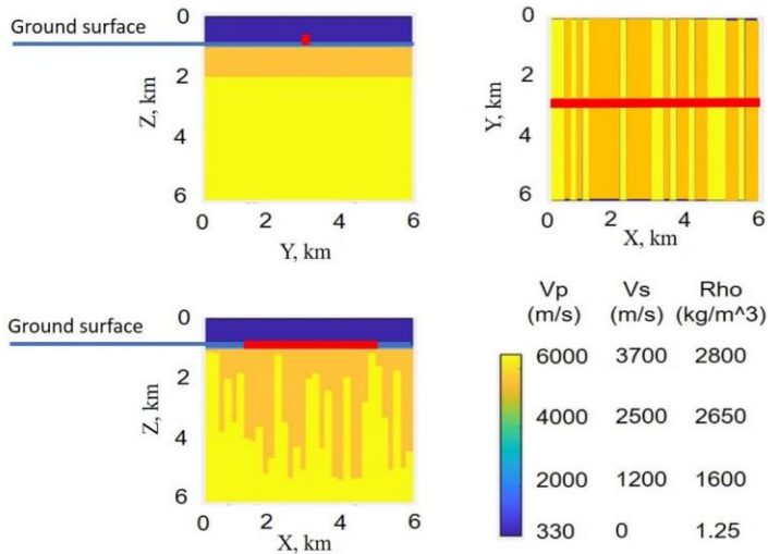
Figure 3: The synthetic model used for investigation of wave propagation. Position of the seismic profile marked by the red line.
