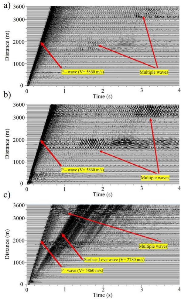
Figure 6: Synthetic seismograms of the blast. The coordinate of source was located at offset of is -300 m : a) vertical channel Z; b) horizontal channel X; c) horizontal channel Y.
