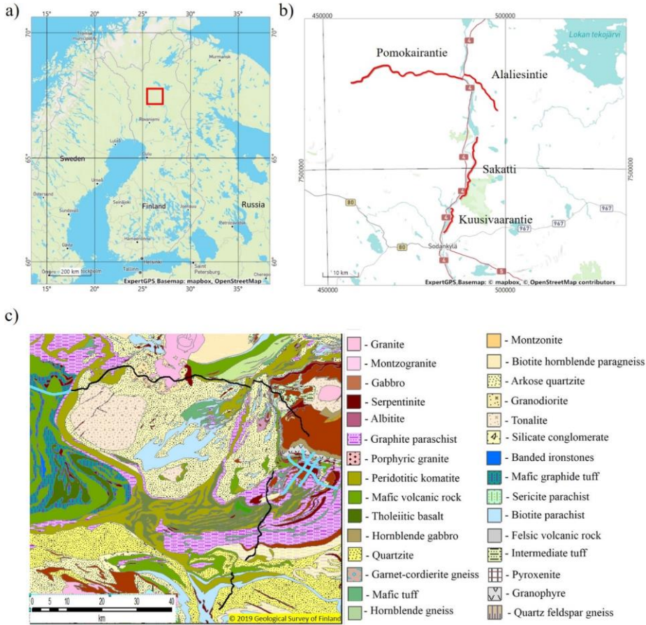
Figure 1: The XSodEx seismic experiment: a) geographical location of the studied area (red rectangle); b) the XSodEx survey lines (coordinate system EUREF FIN TM35FIN); c) Geological map of XSodEx study area (Buske et al., 2019). The XSodEx survey lines are shown with black lines. Previous seismic reflection survey lines are plotted with blue lines.
