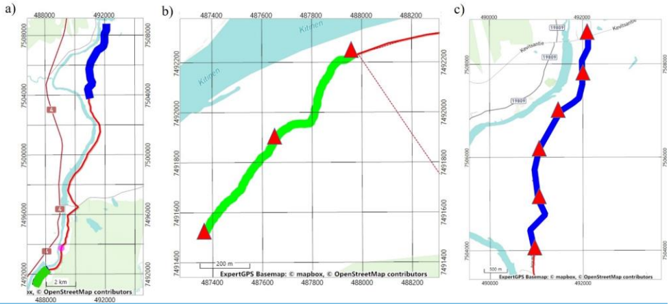
525 Figure 9: Location of passive seismic profiles of XSODEx Sakatti line: a) positions of high-resolution line (green color) and profile of lower resolution (blue line); b) The high-resolution line in which -r-Red triangles marks positions of virtual sources; c) profile of lower resolution (red triangles indicate -r-positions of virtual sources).green-line-indicates-high-resolution-profile; blue-line-indicates profile-of-lower-resolution.
