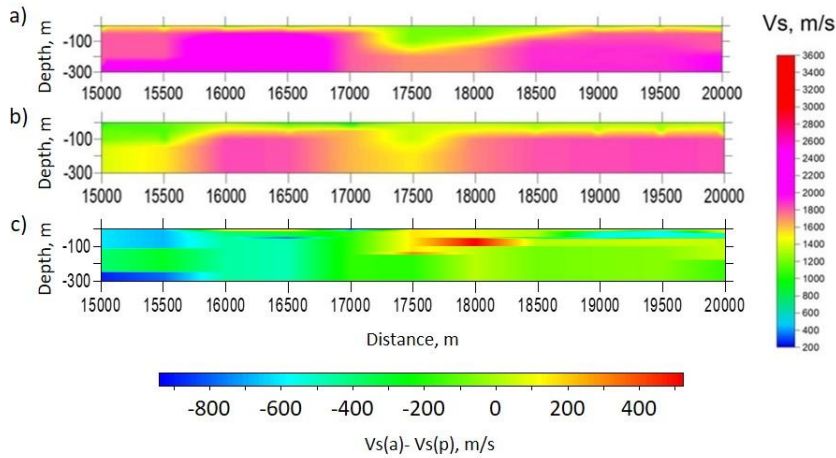
Figure 14: Velocity models calculated by inversion of dispersion curves along the part of Sakatti profile marked by blue in Fig. 9. (a) S-wave velocity model obtained using passive seismic data; (b) S-wave velocity model obtained using seismic data, which contain signals produced by controlled source; c) differences between S-wave velocity models in plots (a) and (b), obtained using seismic data, which contain signals produced by controlled source and obtained using passive seismic data.
