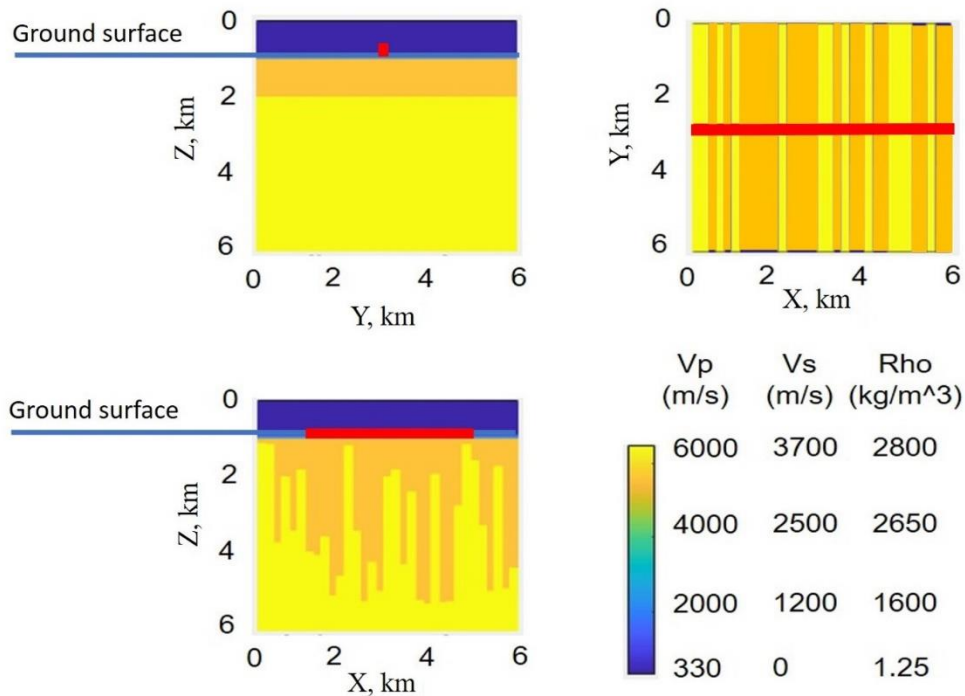
475 Figure 3: The synthetic model used for investigation of wave propagation. Position of the seismic profile marked by the red line. Low velocity corresponding to the air is indicated on the top by blue colour.
