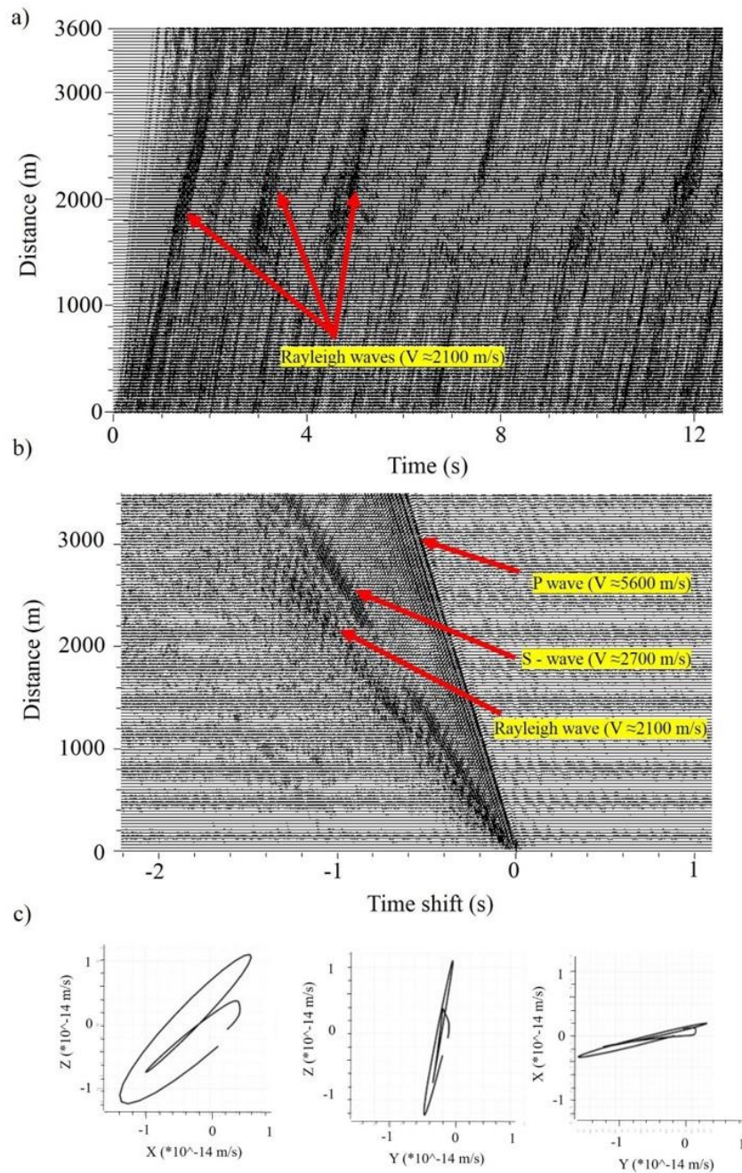
495 Figure 8: Synthetic seismograms of the signal with the spectrogram presented in Fig. 7 and propagating in synthetic model shown in Fig. 3. The virtual source is located at offset of 0 m: a) seismograms of vertical components; b) cross-correlation functions of vertical components, calculated between the first trace and all other traces in Figure 8 (a); c) particle motion diagram of Rayleigh wave part in Figure 8 (b).
