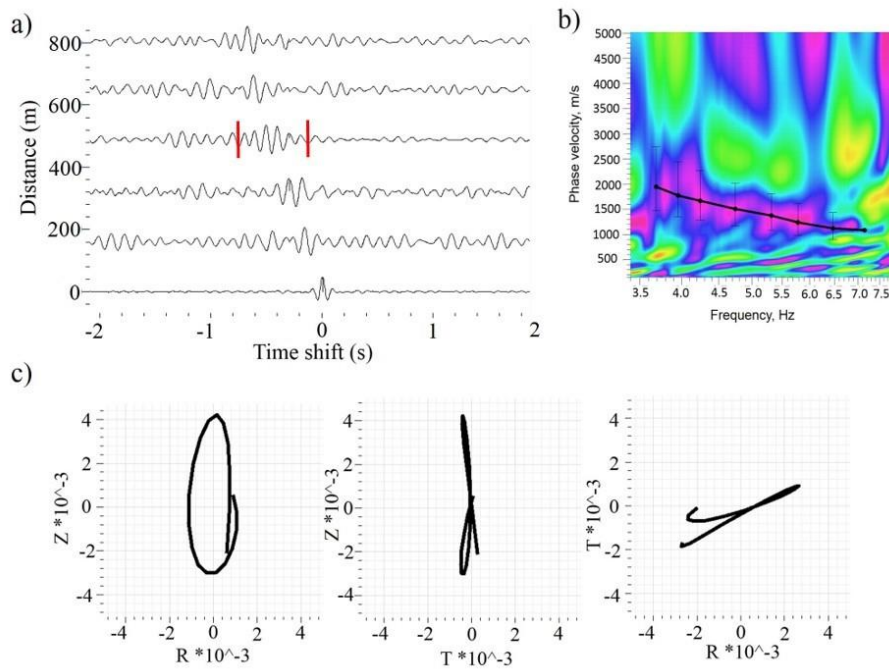
520 Figure 13: Example of EGFs with correspondent dispersion curve, obtained from passive seismic data: a) EGFs on frequency band 3-8 Hz; b) dispersion curve, calculated from EGFs by MASW technique; c) particle motion diagrams of a surface wave part of an EGF indicated by red lines.
