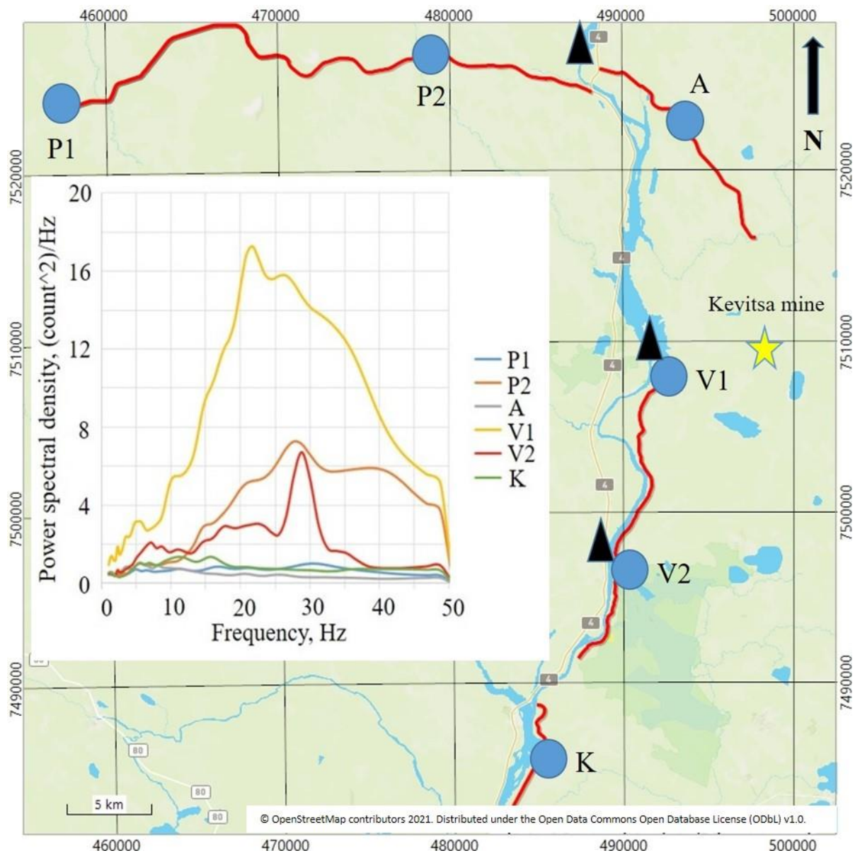
470 Figure 2: Illustration of noise level at six stations located in different profiles of the XSoDEX experiment. Position of strong noise sources (Kevitsa mine (yellow star) and dams of waterpower stations (black triangles)) and seismic stations selected for analysis (blue circles) are indicated. Brown and white lines show roads. Inset figure shows comparison of ambient noise power spectral density estimated at selected stations.
