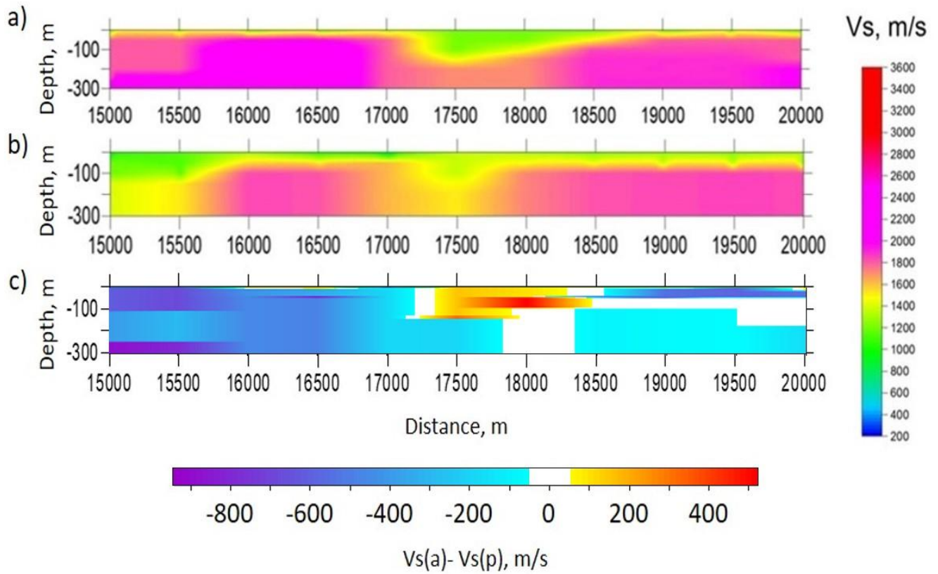
525 Figure 14: Velocity models calculated by inversion of dispersion curves along the part of Sakatti profile marked by blue in Fig. 9. (a) S-wave velocity model obtained using passive seismic data; (b) S-wave velocity model obtained using seismic data, which contain signals produced by controlled source; (c) differences between S-wave velocity models in plots (a) and (b).
