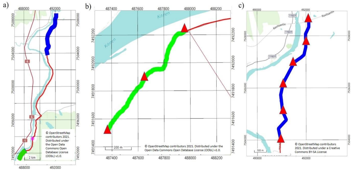
500 Figure 9: Location of passive seismic profiles of XSoDEx Sakatti line: a) positions of high-resolution line (green color) and profile of lower resolution (blue line); b) The high-resolution line in which red triangles marks positions of virtual sources; c) profile of lower resolution (red triangles indicate positions of virtual sources).
