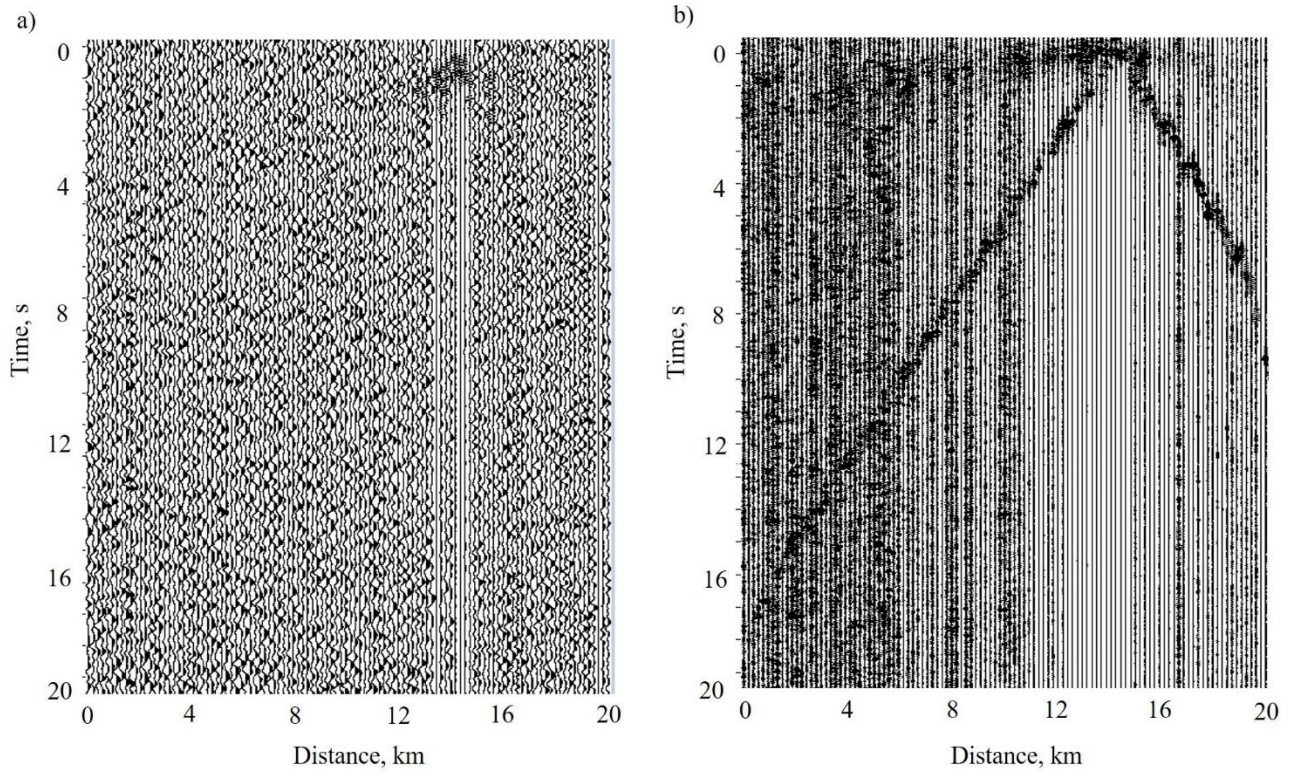
530 Figure 15: Cross-correlation functions of signals, produced by Vibroseis© with the data recorded by wireless equipment at large offsets in frequency band of: a) 1-10 Hz, amplitudes normalized at maximum of each trace; b) 20-100 Hz. The signal used for cross-correlation is shown in Fig. 16.
