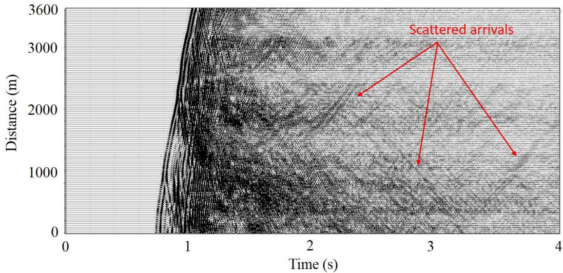
480 Figure 4: An example of synthetic seismogram (vertical component) of plane wave arrived with incidence angle of 45 degree and propagated through the synthetic model (0-4 sec). The seismogram shows first arrivals and numerous reflections. From about 1.5 seconds we can see scattered arrivals of different directions with apparent velocities of 2100 -2500 m/s. Several arrivals of scattered waves are indicated by red arrows.
