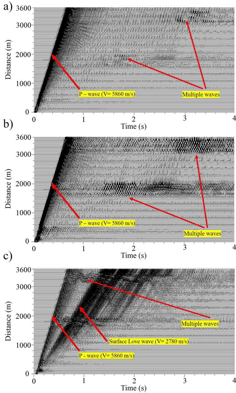
490 Figure 6: Synthetic seismograms of the blast. The source was located at offset of -300 m: a) vertical channel Z; b) horizontal channel X; c) horizontal channel Y.
