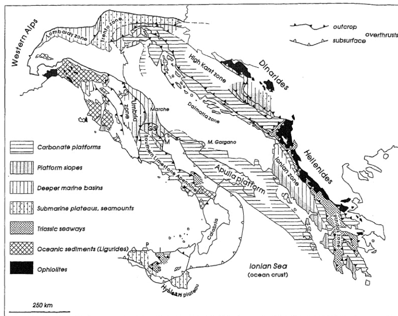
Figure 18.1 Tectonic units and late Jurassic palaeogeography in the peri-Adriatic area. No palinspastic correction was made (after Bernoulli, 1972; with additions from Cati et al. , 1987 and Argnani et al. , 1996). (GS, Gran Sasso d'Italia; I, Imerese basin; L, Lagonegro basin; M, Montagna della Maiella, P, Panormic platform; S, Sicani basin; T, Toscanides; the Umbria seamounts are too small to be indicated at this scale).
