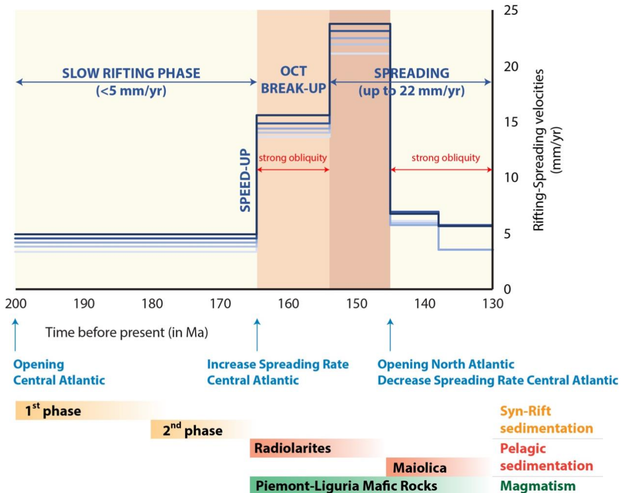
525 Figure 5. Velocities (full-rate) of rifting and spreading along the PL basin between Europe (Corsica-Briançonnais) and Adria (blue vectors on Fig. 4) in Jurassic-Early Cretaceous time. Timing of syn-rift sedimentation from Froitzheim and Eberli (1990), deep-sea pelagic sedimentation from Bill et al. (2001) and Ferrando et al. (2004), and U/Pb ages on zircons from mafic rocks of the PL ocean from Manatschal and Müntener (2009 and references therein). Note the slight increase in velocities from NE to SW (light to dark blue curves) and the strong acceleration at 164.7 and 154 Ma for all curves.
