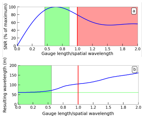
475 Figure 2: The signal-to-noise ratio (SNR) (a) and resulting wavelength (b) for different ratios of gauge length to spatial wavelength for a 10-112 Hz Klaunder wavelet with a velocity of 4800 m/s. The green boxes indicate the range of ratios where SNR>90% of the maximum, and the resulting wavelength is within 3 m of the actual wavelength. If the gauge length is larger than the spatial wavelength (red box), the wavelet shape is distorted. The optimum conditions satisfying both constraints are found in the region where the two green boxes in (a) and (b) overlap.
