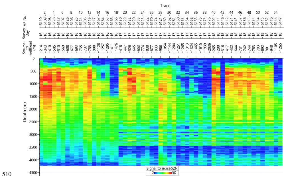
Figure 8: Signal-to-noise ratio (dB) for DAS-VSP data from well GrSk3.
