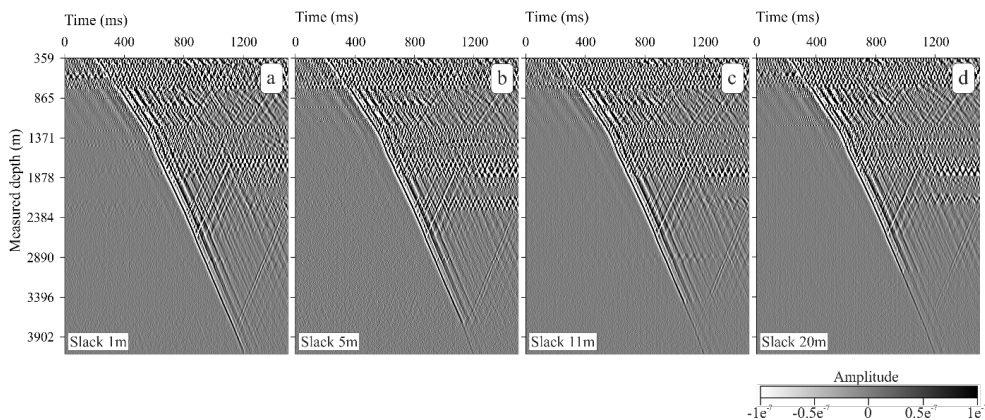
Figure 7: Comparison of common-source gathers recorded with cable slack of 1 m (a), 5 m (b), 11 m (c), and 20 m (d) for VP10 in well GrSk3.
