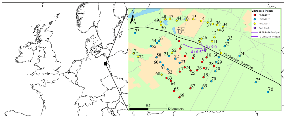
470 Figure 1: Overview map of central Europe with location of survey area in NE Germany. Inset shows detail of survey area with VSP source point positions and borehole trajectories of wells E GrSk 3/90 and Gt GrSk 4/05.
