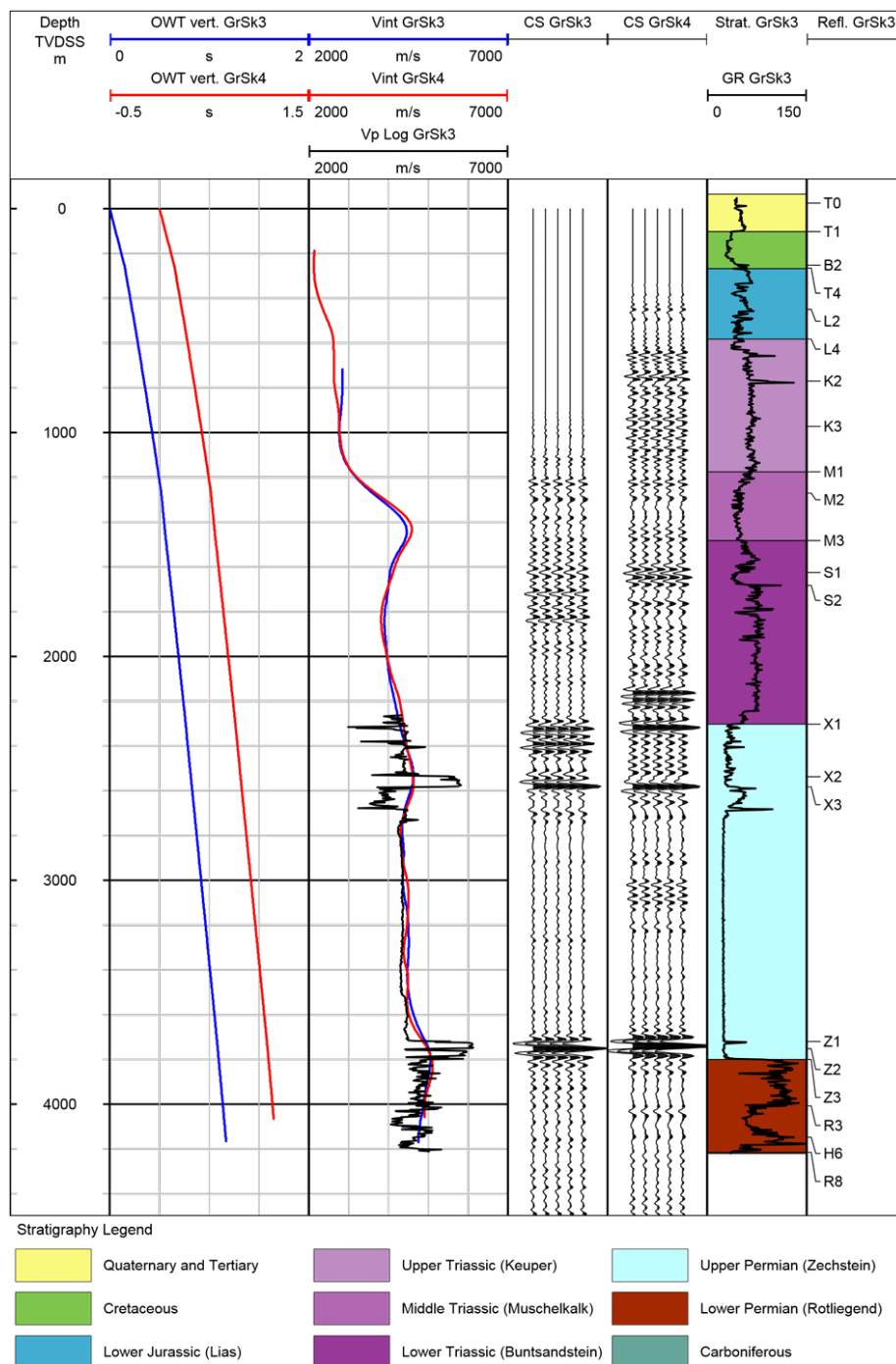
Figure 10: Vertical one-way travel times (OWT vert), VSP interval velocities (Vint), acoustic log sonic velocities (Vp log), and corridor stacks (CS), together with stratigraphic units, gamma-ray log (GR) and seismic reflectors. TVDSS: True vertical depth below mean sea level.
