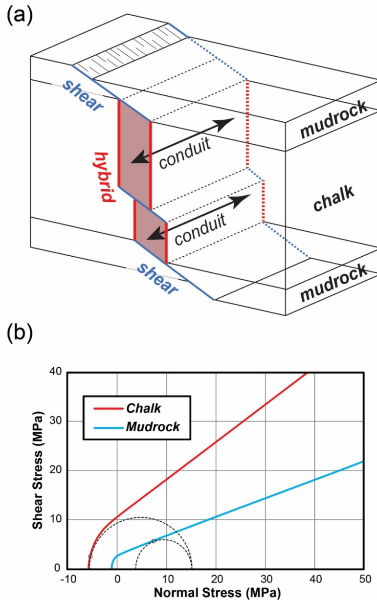
215 Figure 6. (a) Schematic block diagram illustrating the change in failure angle and mode from mudrock to chalk, and the associated dilation of the steeper hybrid segment and formation of a fault conduit parallel to the fault-bedding intersection direction. (b) Interpreted failure envelopes and stress circles for chalk and mudrock at the time of failure with a uniform effective overburden stress of 20 MPa (corrected for pore fluid pressure) with hybrid failure predicted for the more competent chalk beds and shear failure predicted for the less competent mudrock.
