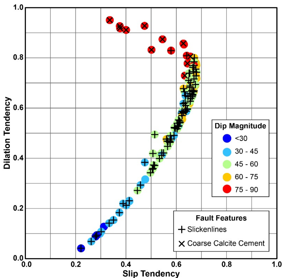
180 Figure 5. Comparison of dilation tendency and slip tendency for measured fault segments of the Textbook, Spanish Goat, and Big Indigo faults, color-coded by dip, with + and × symbols indicating presence of slickenlines or coarse calcite cement, respectively. The few colored dots that lack additional symbols represent shear segments that either lack slickenlines, or slickenlines could not be seen due to the planar outcrop surface in some locations. The moderate to high slip tendency and high dilation tendency of the steep segments (dips >75^\circ , red points) are consistent with hybrid failure, whereas the moderate to low slip tendency and low dilation tendency of the most gently dipping segments (dips <45^\circ , light blue and dark blue points) are suggestive of compactive shear. See Fig. 1 for comparison.
