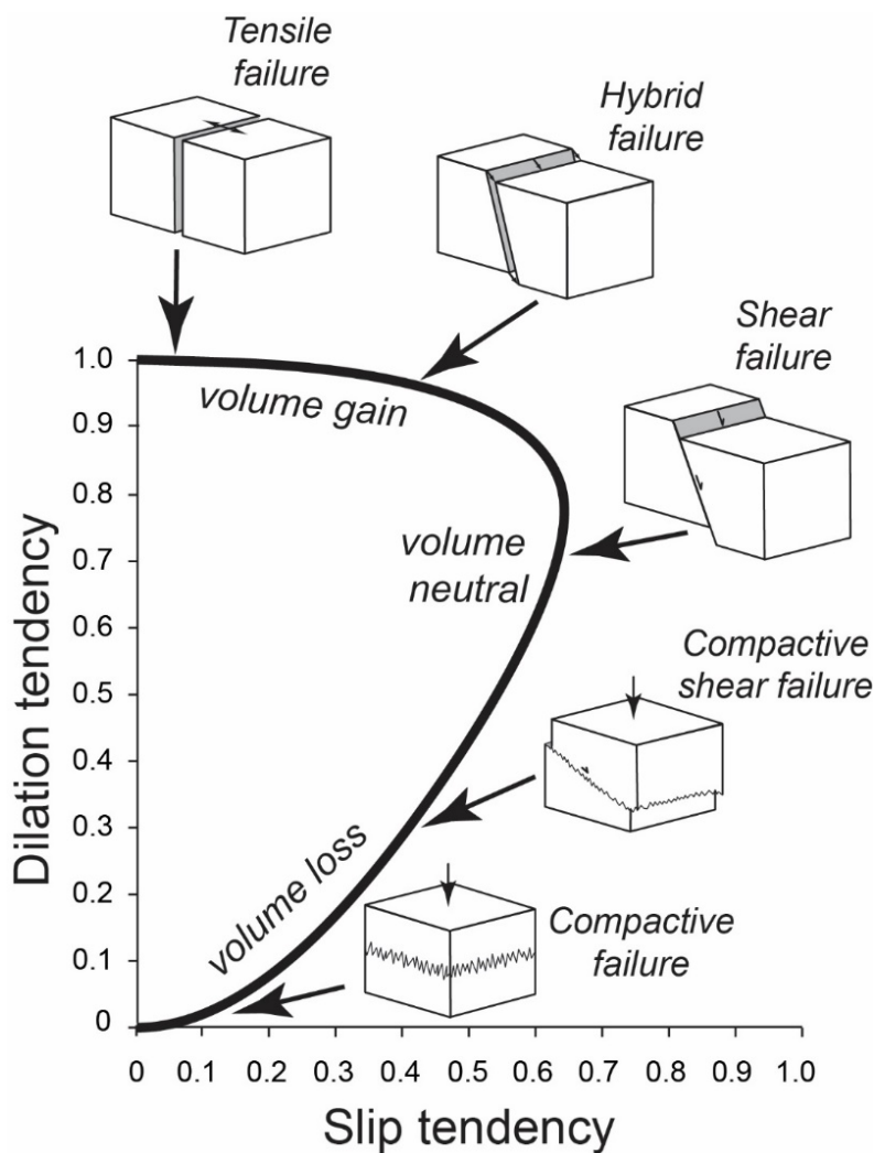
Figure 1. General graphical relationship between maximum slip tendency and dilation tendency, and associated rock failure modes and volume change (from Ferrill et al., 2019a). As discussed by Ferrill et al. (2019a), analysing faults in this parameter space shows promise for prediction of the failure or deformation modes and the associated conduit versus seal behaviour. For purposes of this illustration, representative deformation features are shown for a normal faulting stress regime.
