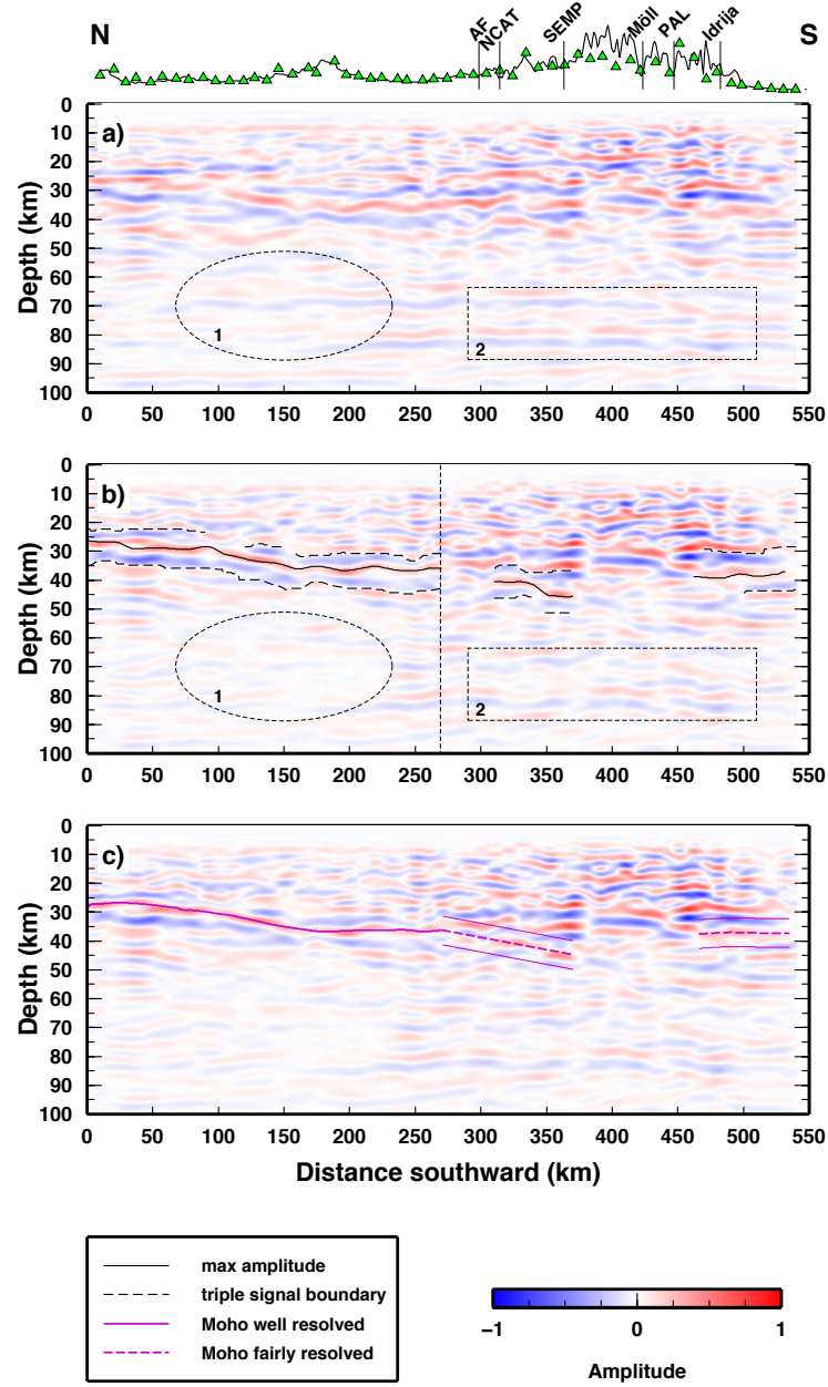
Figure 4. Reflectivity images of the crust and upper mantle along EASI; in the background the interpolated figure ( bilinear interpolation ), in which blue-red-blue triplet marks the presence of a positive interface (i.e. an increasing impedance contrast with depth). a) Depth migrated GloPSI image generated by using 64 27 events. b) Depth migrated GloPSI image generated by using 27 64 events, black solid line marks the lower-zero-crossing maximum amplitude within the blue-red-blue triplet, black dashed line marks the upper and lower boundary of the triplet; features 1 and 2 are described in the text. c) background same as (b), solid and dashed purple line show the picked Moho depths reported in Table S2.
