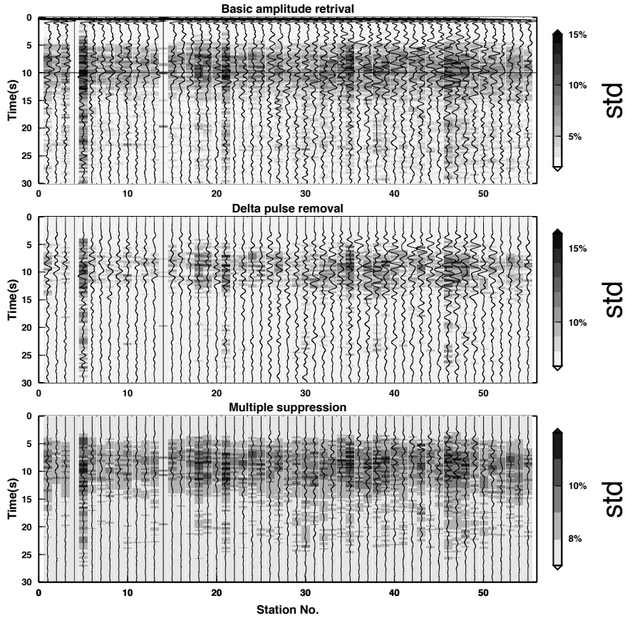
Figure 3. Standard deviation calculated over 100 samples generated by bootstrapping events ensembles by the pool of 27-selected 64 events (marked by the asterisk in Table S1). Mean wiggles are displayed on top of the std.
