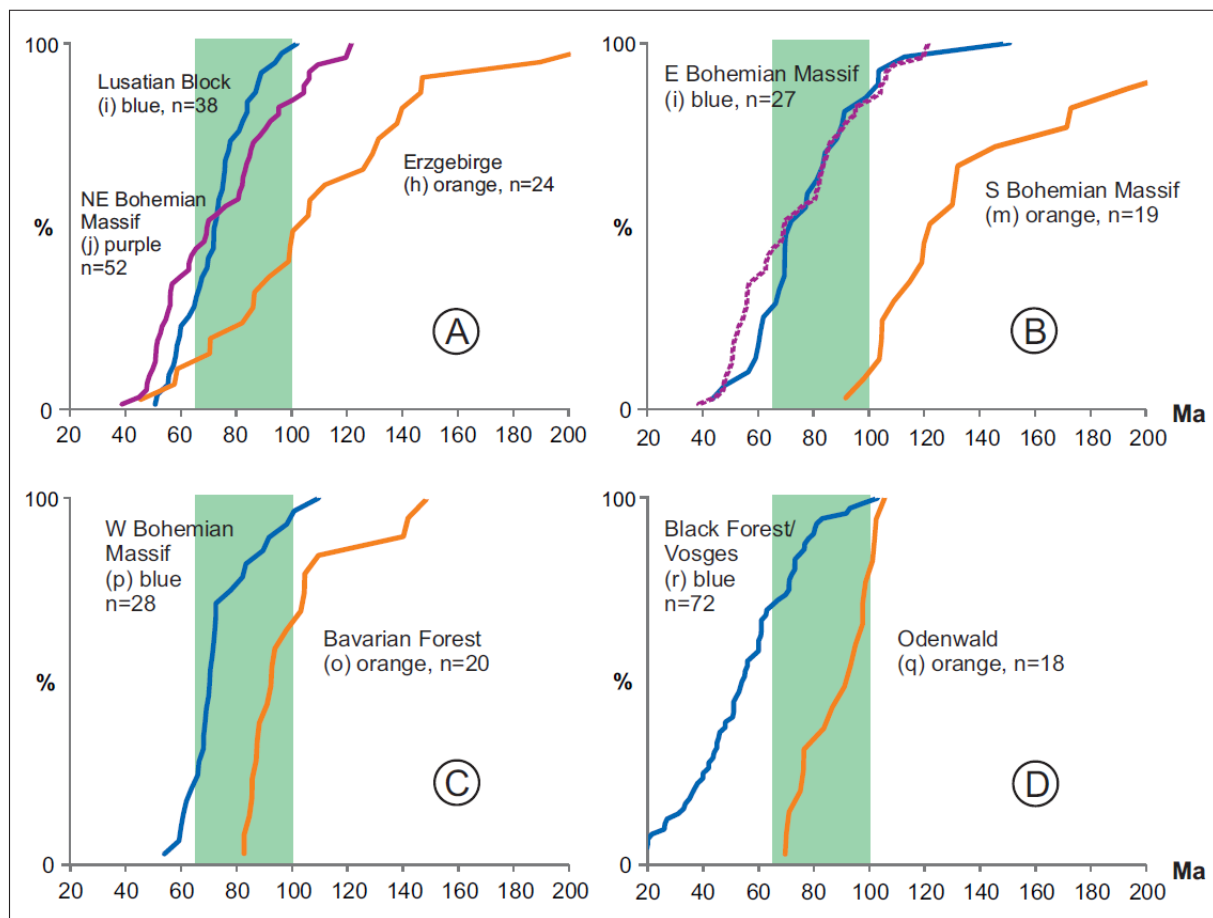
Figure 2: Cumulative frequency distributions of apatite fission track data from various regions across Central Europe. Characters in brackets refer to locations in Figure 1; for references see caption to Fig. 1. Stippled purple line in B is from NE Bohemian Massif like in A, for reference. Green area indicates the time interval of the Late Cretaceous.
