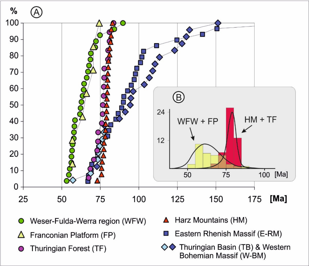
Fig. 8: (A) Cumulative distribution of apatite fission track ages assorted for the individual regions outlined in Figure7. Note that the central Thuringian Basin data (TB) are plotted together with its eastern transition in to the Bohemian Massif (W-BM) in a single cumulative curve, but with different color. The Harz Mountain data are taken from von Eynatten et al. (2019) and the Thuringian Forest data set is composed of our new results and data published by Thomson and Zeh (2000). (B) Histograms and kernel density estimates (KDE, Vermeesch, 2012) to emphasize the highly significant contrast of Werra-Fulda-Weser (WFW) and Franconian Platform (FP) data versus Harz Mountains (HM) and Thuringian Forest (TF) data, which differ by 15 to 20 Myr.
