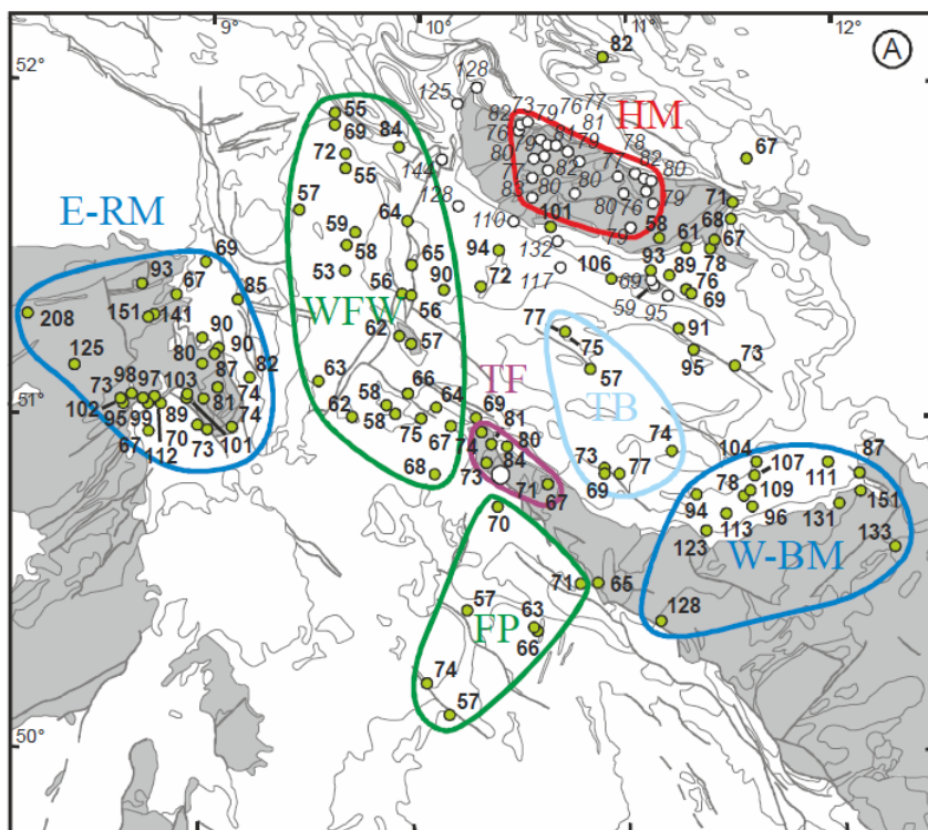
Figure 7: Spatial presentation of the new apatite fission track (A) and (U-Th)/He ages (B). The map is a simplified version of Figure 3; grey color represents Permian Rotliegend and older formations (i.e. pre-Zechstein). Colored envelopes in (A) highlight the regions defined in the text and Figure 3, where most of the samples are clustering. Small white circles in and around the Harz Mountains indicate localities of low-T thermochronology data by von Eynatten et al. (2019). The bigger white circle in the Thuringian Forest indicates the locality of the AFT samples from the Ruhla Crystalline Complex, Thomson and Zeh (2000).
