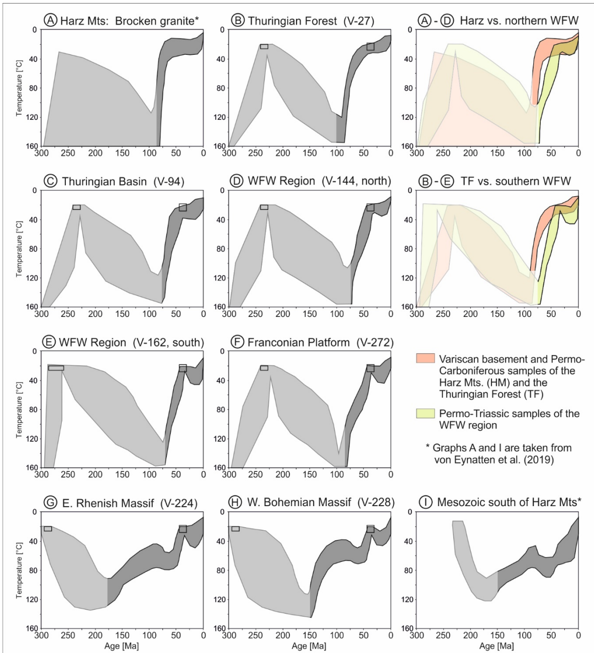
Figure 9: Time-temperature (tT) plots showing the envelopes of the good results of the modelling series performed on selected samples from the different regions. The modelling has been performed by HeFTy software (Ketcham, 2005) using the AFT data. Only tT-paths classified as good fits by the program are considered. The dark grey sections represent the well constrained intervals of the cooling histories, while the light grey fields indicate the time-temperature regime where the modelling results carry insignificant information, as these ranges are older than the oldest fission tracks in the samples. Grey boxes indicate the time-temperature constraints when the dated samples experienced surface temperature conditions. The graphs in the upper right emphasize the contrast in the post-climax cooling paths between the exhumed basement blocks (A, B) and the Permo-Triassic of the WFW core region (D, E).
