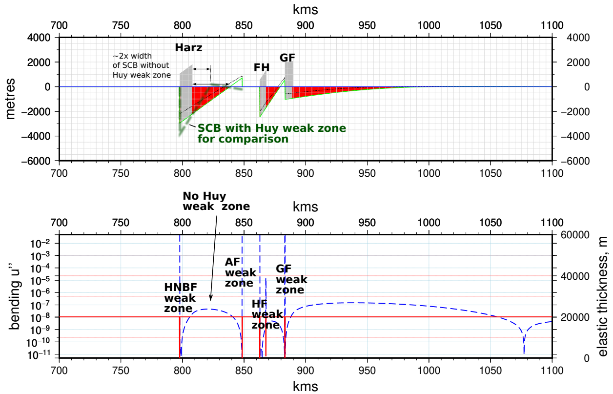
Figure 8. Flexure model, same as Fig. 6, but not including the Huy weak zone, to simulate the situation in the western part of the basin. Basin width of the model including the Huy weak zone is shown for comparison (dark green, dashed line). Abbreviations: HNBF - Harz Northern Boundary Fault; AF - Allertal Fault; HF - Haldensleben Fault; GF - Gardelegen Fault; SCB - Subhercynian Cretaceous Basin
