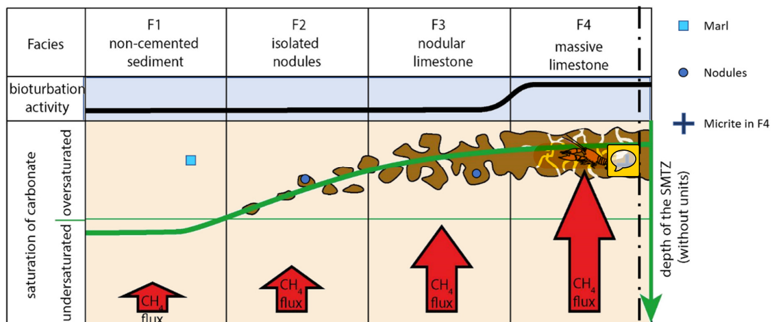
Figure 14: Change in depth of the sulfate methane transition zone (SMTZ) and methane-derived authigenic carbonates (brown) from host sediment towards the pseudobioherm; vertical dashed line marking the axis of the pseudobioherm, symbols referring to the isotope data shown in Fig. 13A. Not to scale.
