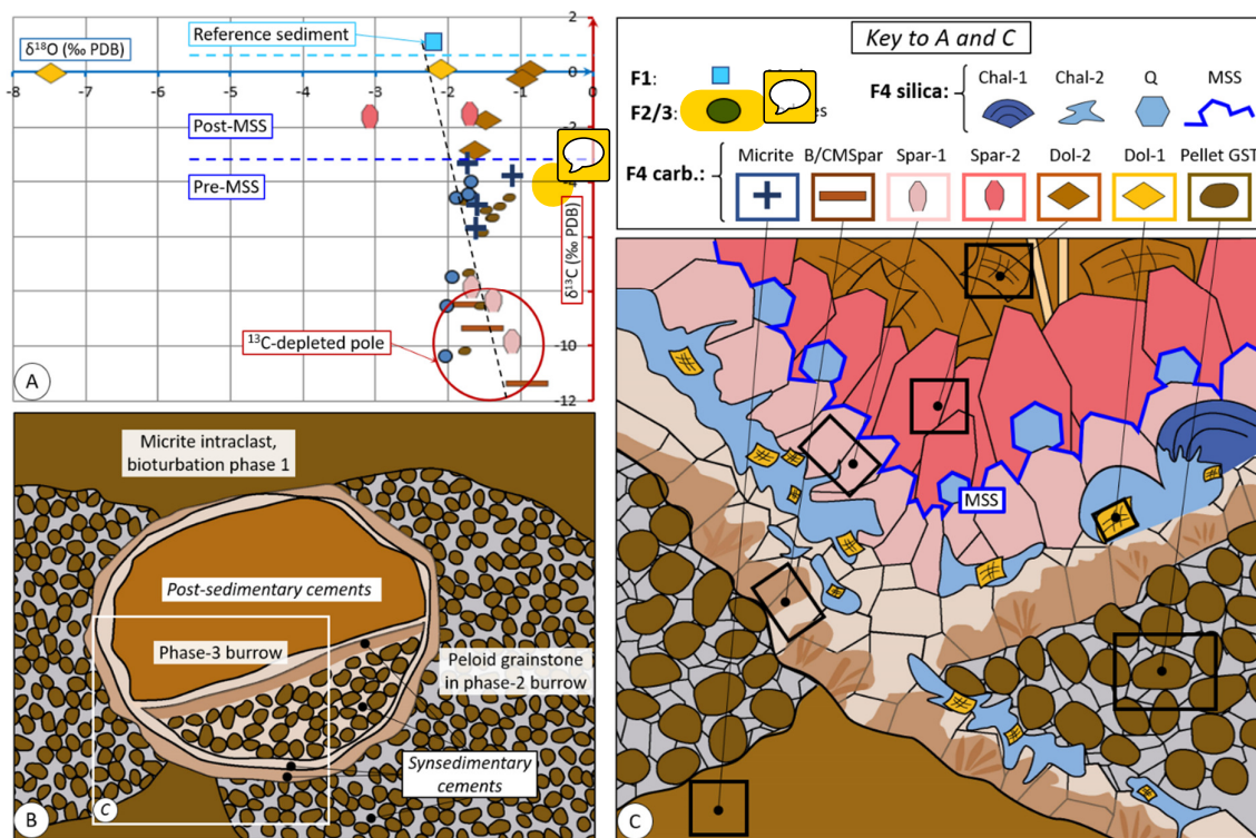
1115 Figure 13: Stable C and O isotopes and microfacies. A) Sedimentary and diagenetic carbonate phases encountered in the Aurel pseudobioherm in \delta^{13}\text{C} - \delta^{18}\text{O} plot; position of samples of facies F1 to F3 is shown in Fig. 14. MCSW = Middle Callovian seawater composition; LMCSW = subset for the lower part of the Middle Callovian (Pellenard et al., 2014). 1120 Fabric and microfacies of F4 recording successive phases of bioturbation. Schematic geometric relationships between sediment and various cement generations and their stable isotope values within facies F4; black boxes mark minimum size of samples drilled for isotope analysis, some likely mixing different phases like peloid grainstone and BMSpar/CMSpar. GST = grainstone, MSS = main silicification surface. Details, see text.
