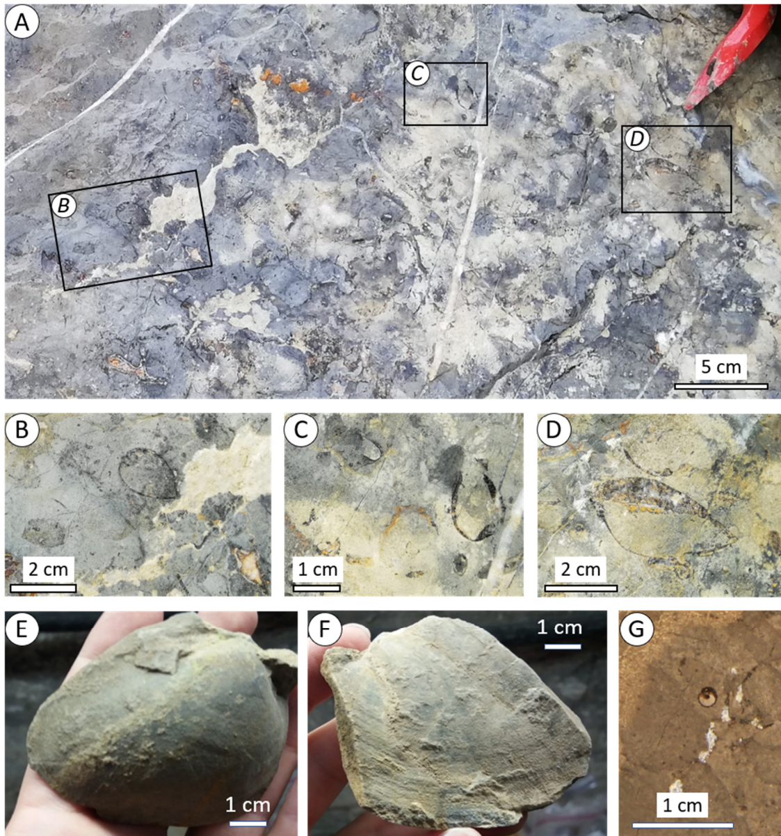
Figure 7: Facies F4, massive limestone, and associated fauna. A) Weathered surface showing three bivalves shown in (B) to (D) in detail, apparently belonging to different species. B) Bivalve with geopetal filling. E) and F) Two valves of the only lucinid found ( Beauvoisina carinata , Kiel et al., 2010). G) Section of a small gastropod. H) Bedding plane view of Thalassinoides ; smaller tape measure graduations in mm.
