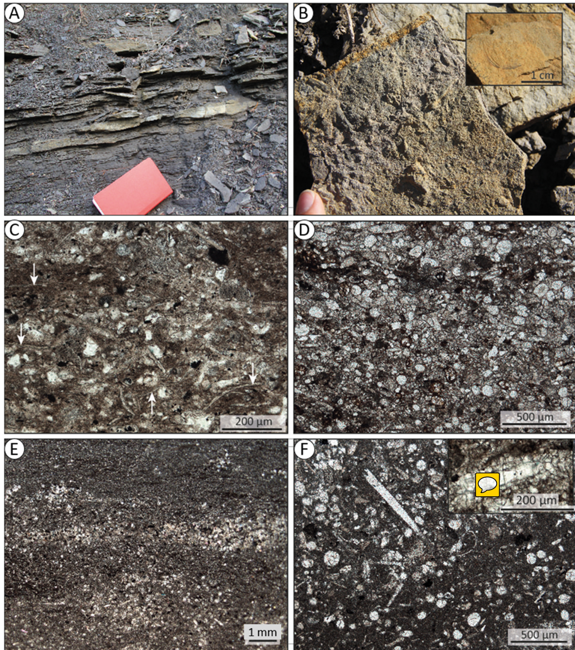
Figure 4: Background facies F1. A) Typical alternation between marl and limestone showing platy bedding. B) Surface of a slab with radiating burrow ( Gyrophyllites multiradiatus ); inset shows the bivalve Bositra , the only common fossil in F1. C) Marl with numerous filamentous structures interpreted as disaggregated Bositra shells. D) Limestone showing the same microfossil content as the marl but in microsparitic matrix. E) Limestone consisting of alternating packstone and wackestone laminae. F) Marl with numerous recrystallized microfossils in a micritic matrix; circular objects are interpreted as calcispheres or radiolarians; inset showing a tubular structure interpreted as a sponge spicule.
