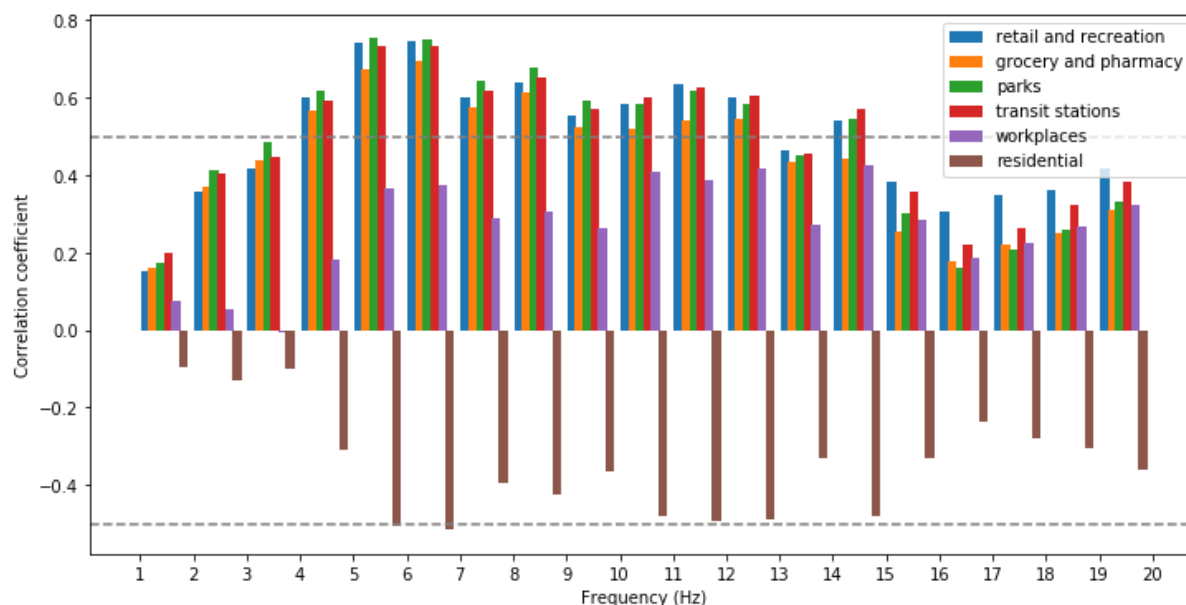
105 Figure 3. Correlation coefficient between the seismic RMS in narrow 1 Hz frequency band from 1 to 20 Hz at station R6BB7 and the Google community mobility in the high categories of retail and recreation, groceries and pharmacy, parks, transit stations, workplaces, and residential premises. The highest correlation and anticorrelation are identified between 4 and 14 Hz.
