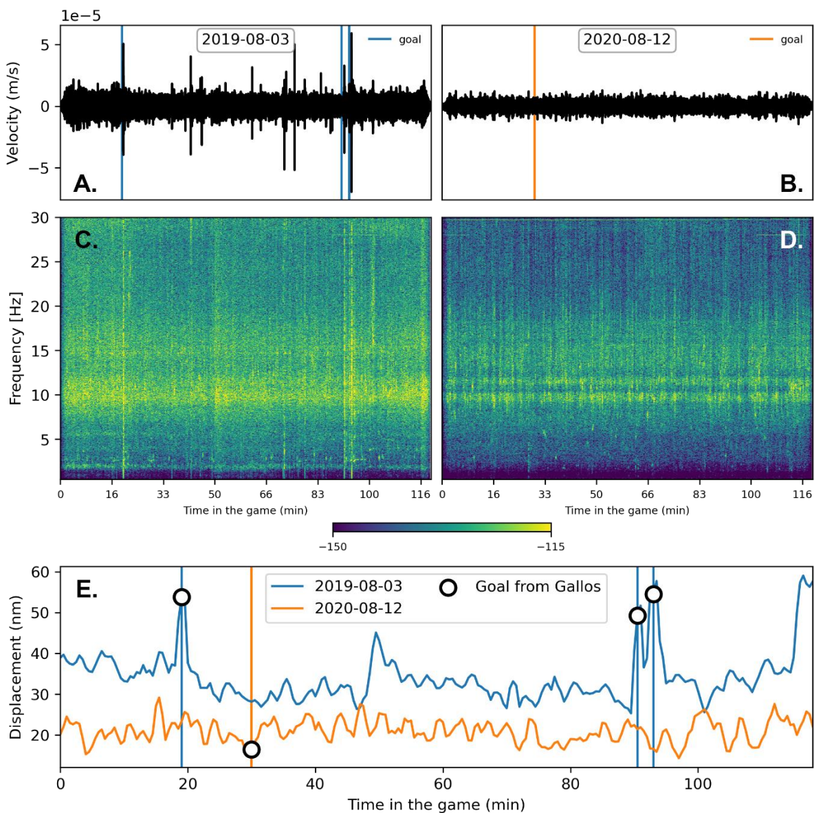
210 Figure 6. Seismic signal recorded by station REBDD during the football games between the Gallos Blancos of Querétaro and the Cruz Azul of Mexico City in the Corregidora Soccer Arena on 3 August 2019 and 12 August 2020, respectively. (A) and (B) are the waveforms, and (C) and (D) the spectrogram for each respective game. (E) compares the seismic RMS between the two games.
