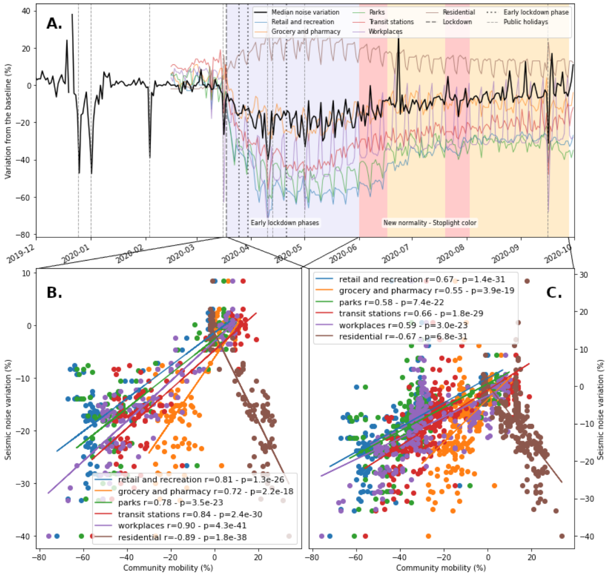
170 Figure 5. (A) Median of the variation of the seismic RMS at all stations, relative to the median of the corresponding day of the week during the baseline period of 13 January to 2 March, and variation of the Google community mobility in 6 high-level categories. The public holidays are indicated with blue dashed lines and the implementation of lockdown measures is indicated as the black dashed line. The purple span corresponds to the early lockdown phases and the red and orange spans after 1 June are the corresponding stoplight color for the “New Normality”. Cross-plot between the median seismic RMS of the network and the Google community mobility in 6 high-level categories during the early lockdown phases (B) and including the new normality (C). The spearman correlation coefficients between the median seismic RMS and each category of community mobility and the corresponding p-values are provided in the legend.
