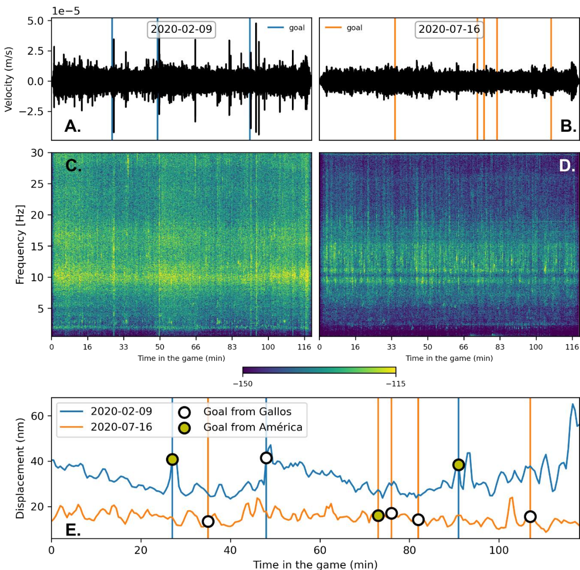
215 Figure 7. Seismic signal recorded by station REBDD during the football games between the Gallos Blancos of Querétaro and the Club América of Mexico City in the Corregidora Soccer Arena on 9 February and 16 July 2020, respectively. (A) and (B) are the waveforms, and (C) and (D) the spectrogram for each respective game. (E) compares the seismic RMS between the two games.
