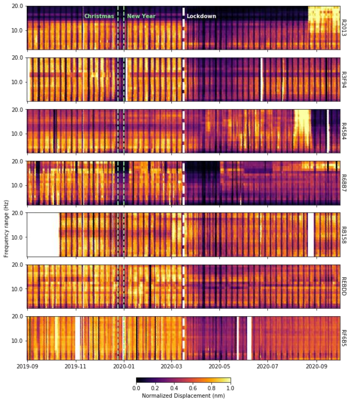
100 Figure 2. Variations of seismic RMS measured with narrow 1 Hz frequency band from 1 to 20 Hz at all stations. The typical succession of business days and weekends can clearly be observed, but the largest reductions in seismic noise levels are identified during the Christmas holiday (green dashed lines are Christmas and New Year, respectively) and following the implementation of lockdown measures mid-March 2020 (white dashed line).
