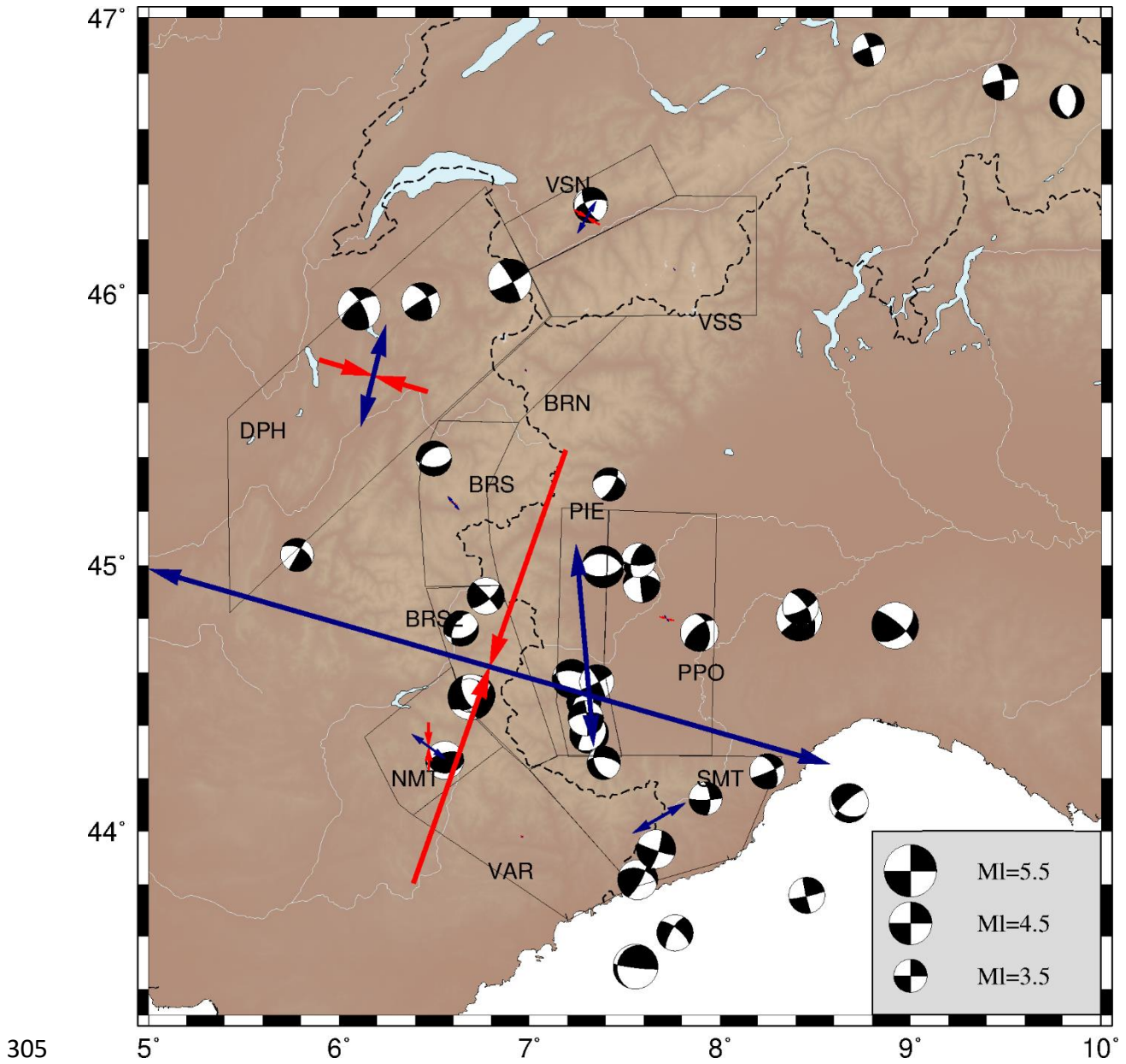
Figure 4. Seismic strain rates computed according to Kostrov's (1974) method in each of the 11 subareas, based on the 25 years of seismicity records from Potin (2016). Blue and red arrows show respectively the extensive and compressive components of the strain rate projected at the surface ( \dot{\epsilon} \cdot \cos(\delta) ), and black arrows represent the scale of the strain rate. Values used for projection are reported in Table 1. Focal mechanisms with M_I \geq 3.5 are represented in the background since strain rates mostly depend on higher moment tensors.
