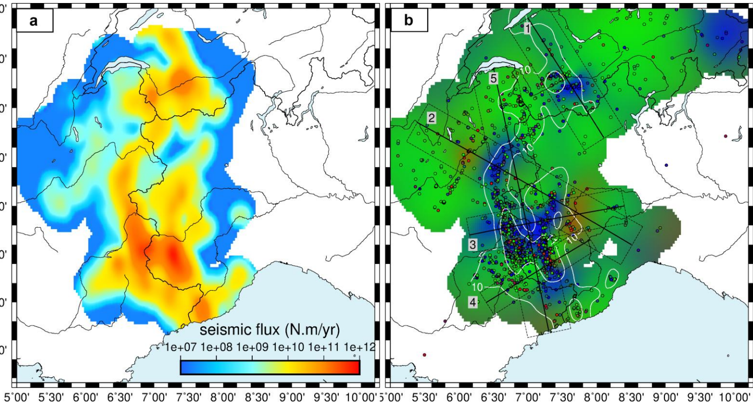
Figure 7. a) Seismic flux computed using the annualized seismic moment ( M_0 ) over the 1989-
