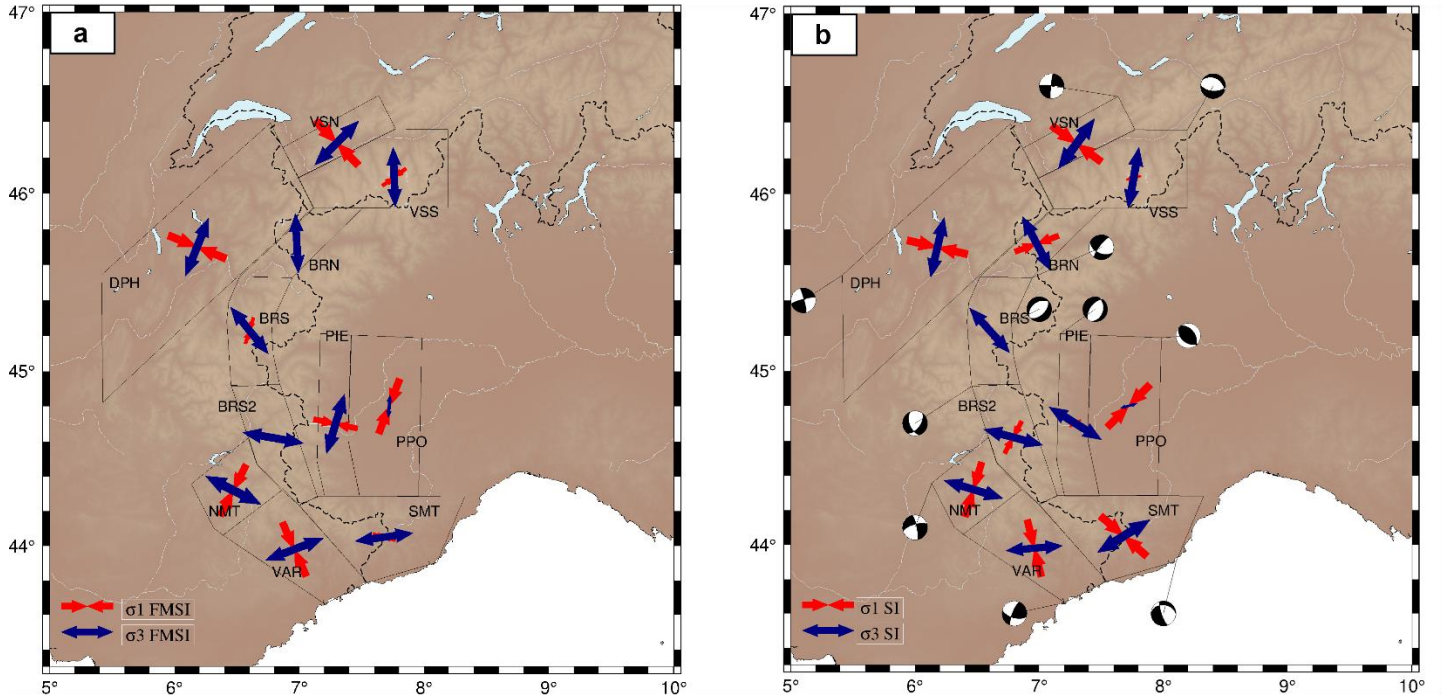
Figure 5. Comparison of stress orientations resulting from FMSI (a) and SI (b) inversions of focal mechanisms within each subarea. Most compressional ( \sigma_1 , in red) and least compressional ( \sigma_3 in blue) stresses are plotted given their plunge ( i.e. arrows length depending on the plunge: the scale arrows in the bottom left corner represent 0^\circ plunging stress axes (horizontal stresses), while 90^\circ plunging stress axes will not be seen on the map). The mean focal mechanism retrieved from SI inversion, and corresponding to each partial stress tensor, is plotted for each subarea in b).
