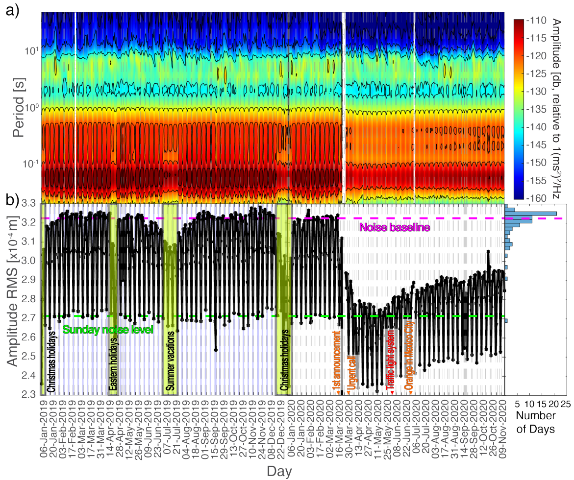
Figure 3: a) Daily median power spectral density for station PZIG. b) Daily RMS noise level for frequencies between 1 to 5 Hz.
