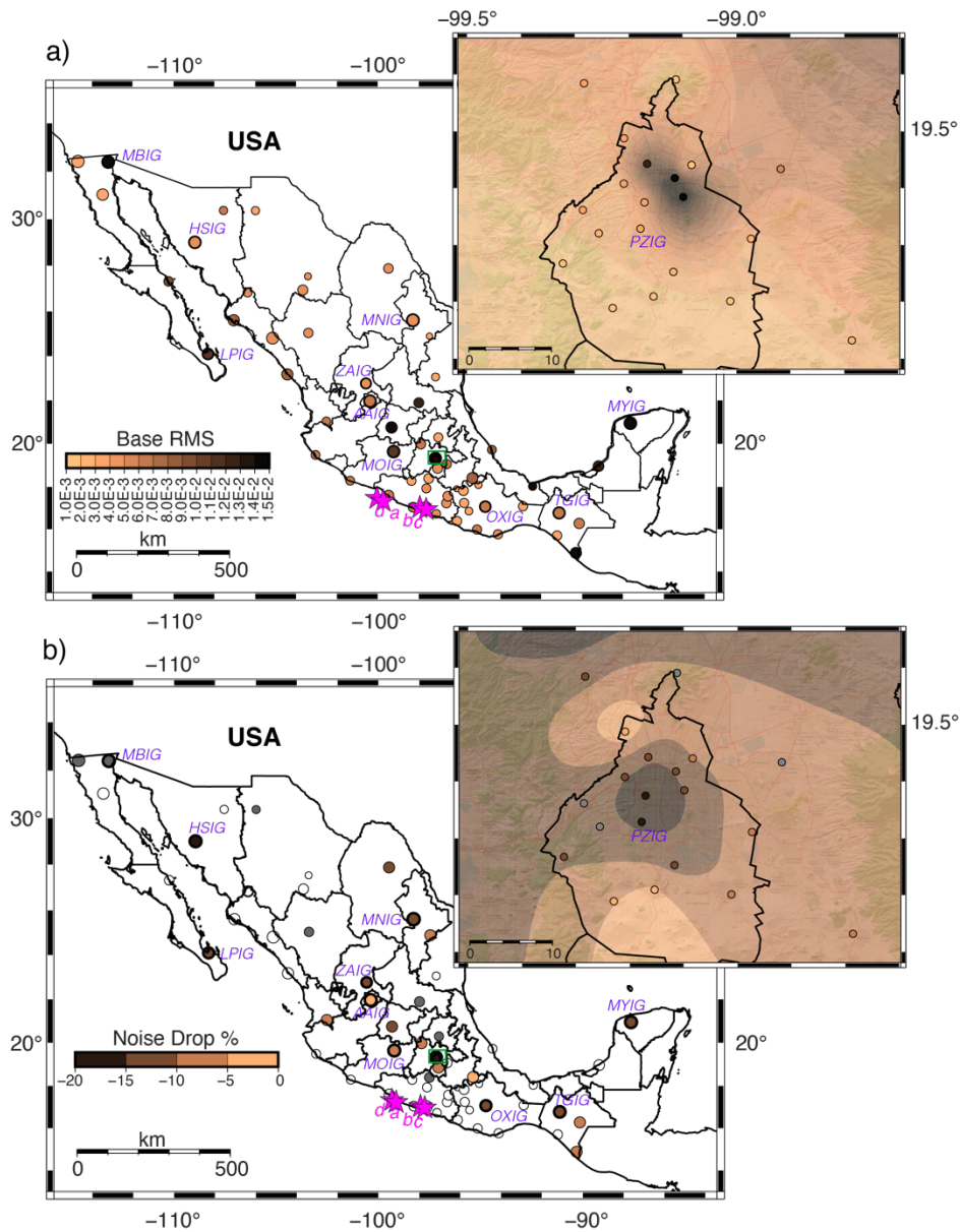
70 Figure 1: a) Noise RMS level and b) drop at seismic stations in Mexico. The pink stars indicate the location of the (a) 2020, M5.0, (b) 2019, M4.9, (c) 2017, M4.9, and (d) 2016, M5.0 earthquakes. The green box corresponds to the Valley of Mexico, shown in the inset. Symbol size is proportional to the municipality population (CEDRUS, 2019) where the station is located.
