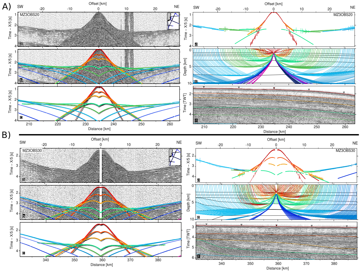
Figure 5. Same as figure 4). Sedimentary and volcano-sedimentary seismic phases on A)MZ3OBS20, B)MZ3OBS30.
