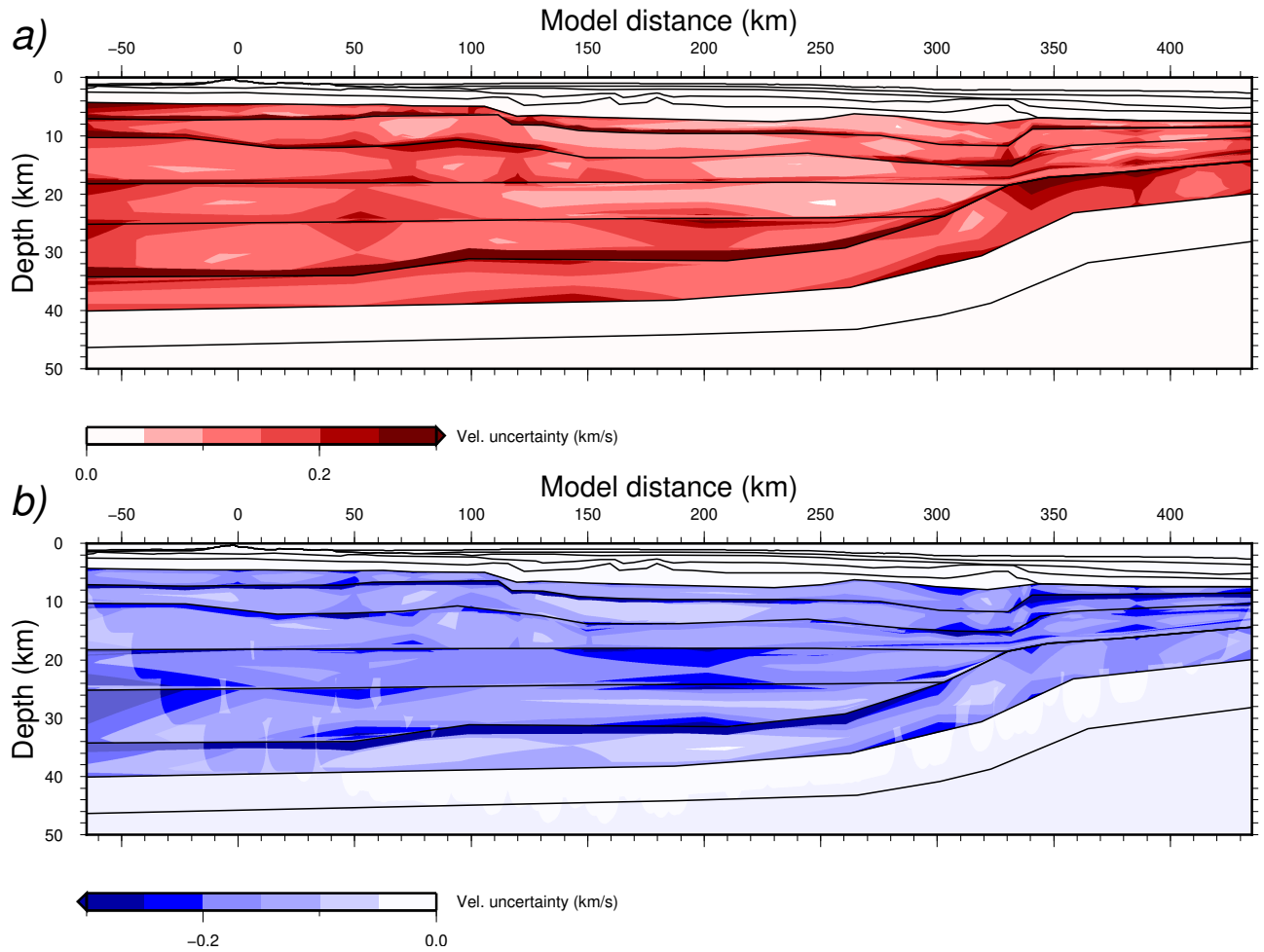
Figure 12. Global uncertainty plots for MZ3. a) Maximum and b) minimum admissible velocity deviations from the preferred model, built from 126 models within the thresholds defined in the text. Shaded areas indicate ray coverage. Preferred model's interfaces are indicated by black lines and velocity deviations are colored according to color scales.
