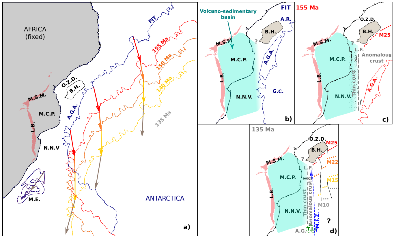
Figure 17. Evolution of the Limpopo Margin (LM). a) Kinematic of the Antarctica plate with respect to the African plate fixed according to (Thompson et al., 2019). b,c,d) Zooms on the evolution of the LM with major features annotated respectively before rifting (b), at break-up (c) and after the opening of the Mozambique Basin along the LM (d). Magnetic anomalies are from Mueller and Jokat (2019). LB: Lelebo monocline; MSM: Mateke Sabi Monocline; MCP: Mozambique Coastal Plain; NNV: North Natal Valley; ME: Maurice Ewing bank; BH: Beira high, OZD: Offshore Zambezi Depression AGA: Antractic Gravity Anomaly; GC: Grunehogna Craton; LF: Limpopo Fault; MFZ: Mozambique Fracture Zone, AG: Ariel Graben. TJ: Triple Junction.
