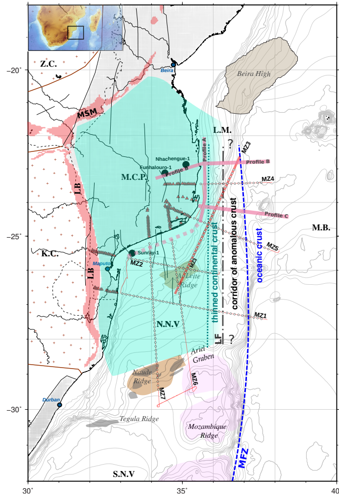
Figure 15. Map of the main segmentation and boundaries within our study area resulting from the combine interpretation of PAMELA-MOZ35 deep seismic profiles. Pink lines are locations of line drawings of commercial MCS profiles shown in figure 14. Background shows main onland geological units and structures: KC: Kaapval Craton; LB: Lebombo monocline; MSM: Mateke Sabi Monocline; MCP: Mozambique Coastal Plain; NNV: North Natal Valley; ZC: Zimbabwe Craton. Offshore bathymetric contours in the LM: Limpopo Margin; Mozambique Basin (MB) and South Natal Valley (SNV) and main geological features: Almirante Leite Ridge (ALR), Beira continental block or high (BH), Limpopo Fault (LF); Mozambique Ridge (MR), Mozambique Fracture Zone (MFZ), Tegula and Naude ridges, Ariel Graben (AG). MOZ35 seismic acquisition in the NNV and LM is shown in red with MZ3 profile highlighted in a bold red line.
