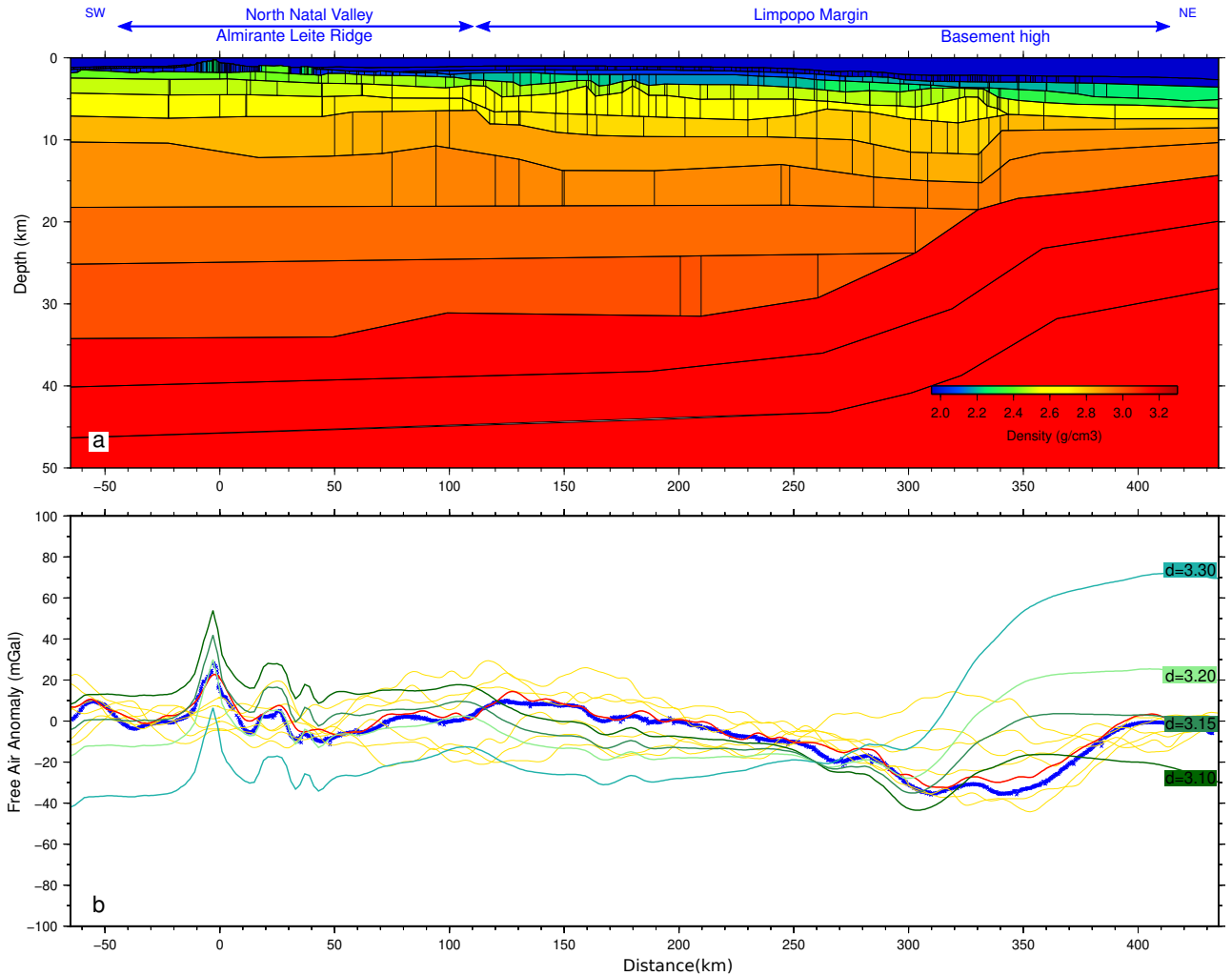
Figure 11. Gravity modeling along MZ3 profile. a) Density model showing blocks of equal density converted from the final velocity model according to (Ludwig et al., 1970) empirical function. b) Gravity anomaly along MZ3 profile. The free-air gravity anomaly derived from satellite altimetry (Pavlis et al., 2012) along the profile is in red while yellow curves correspond to similar profiles extracted at 10, 20 and 30 km laterally (yellow lines). The blue curve is the the gravity anomaly measured during the MOZ35 experiment. Green curves are calculated gravity anomaly from converted model in (a) according to several mantle densities (green labels).
