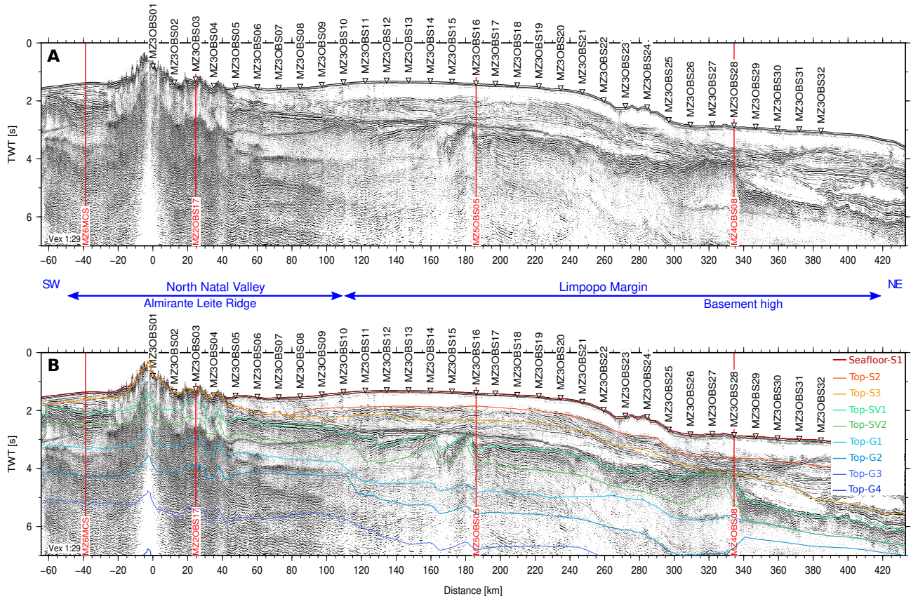
Figure 3. (a) Two-way travel-time record section of MCS data along MZ3 profile. (b) Same as (a) overlain by time converted interfaces from coincident wide-angle velocity model. Intersections with other profile from MOZ35 cruise are indicated by red line. OBS locations are indicated by inverted triangles.
