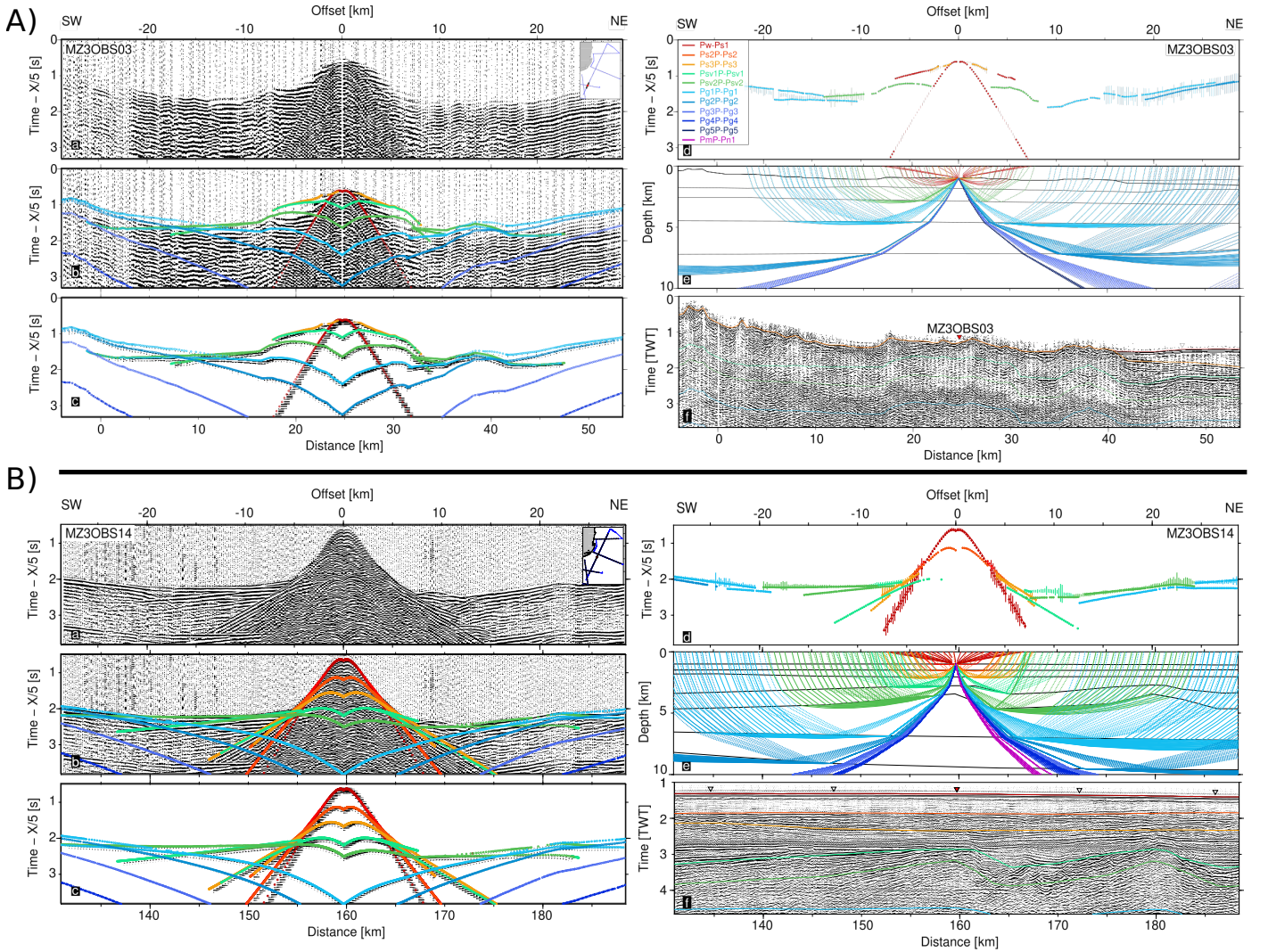
Figure 4. Sedimentary and volcano-sedimentary seismic phases on A) MZ3OBS03, B) MZ3OBS14. For each instrument 6 panels display a) seismic record; b) seismic record with color-coded predicted arrivals; c) synthetic section with color coded predicted arrivals; d) color coded picked travel-times with uncertainty bars overlain by dotted predicted times; e) color coded seismic rays; f) MCS time migrated section with color-coded model interfaces. On a, b, c, and d, travel-time is reduced by a velocity of 5 km/s.
