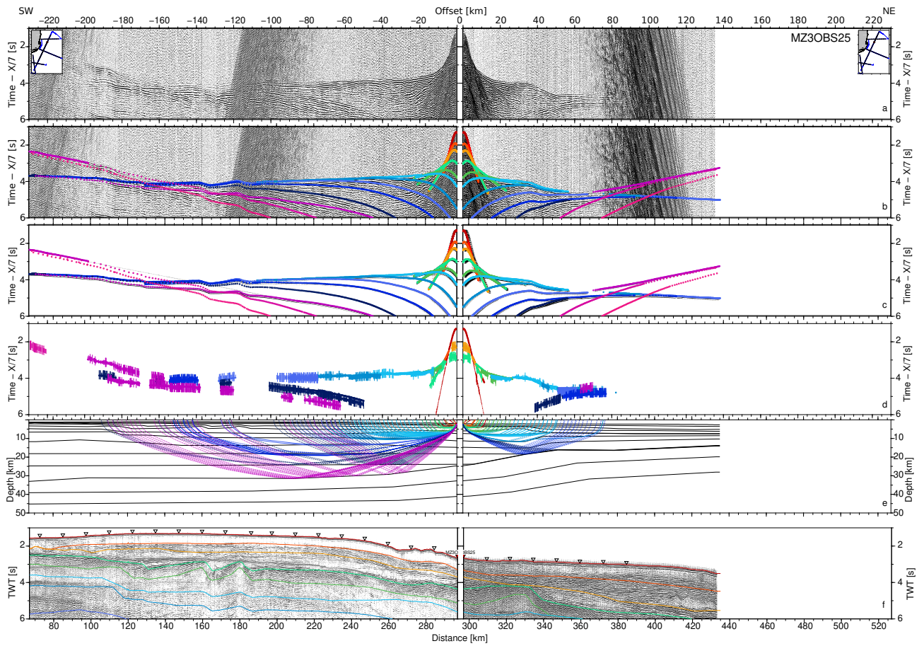
Figure 6. Seismic phases from the crust and mantle on MZ3OBS25. Left panels represent negative offsets (toward the SW) and right panels positive offsets (toward the NE). On each side 6 panels display a) Seismic record; b) Seismic record with color-coded predicted arrivals; c) Synthetic section with color coded predicted arrivals; d) Color coded picked travel-times with uncertainty bars overlain by dotted predicted times; e) Color coded seismic rays; f) MCS time migrated section with color-coded model interfaces. On a, b, c, and d, travel-time is reduced by a velocity of 7 km/s.
