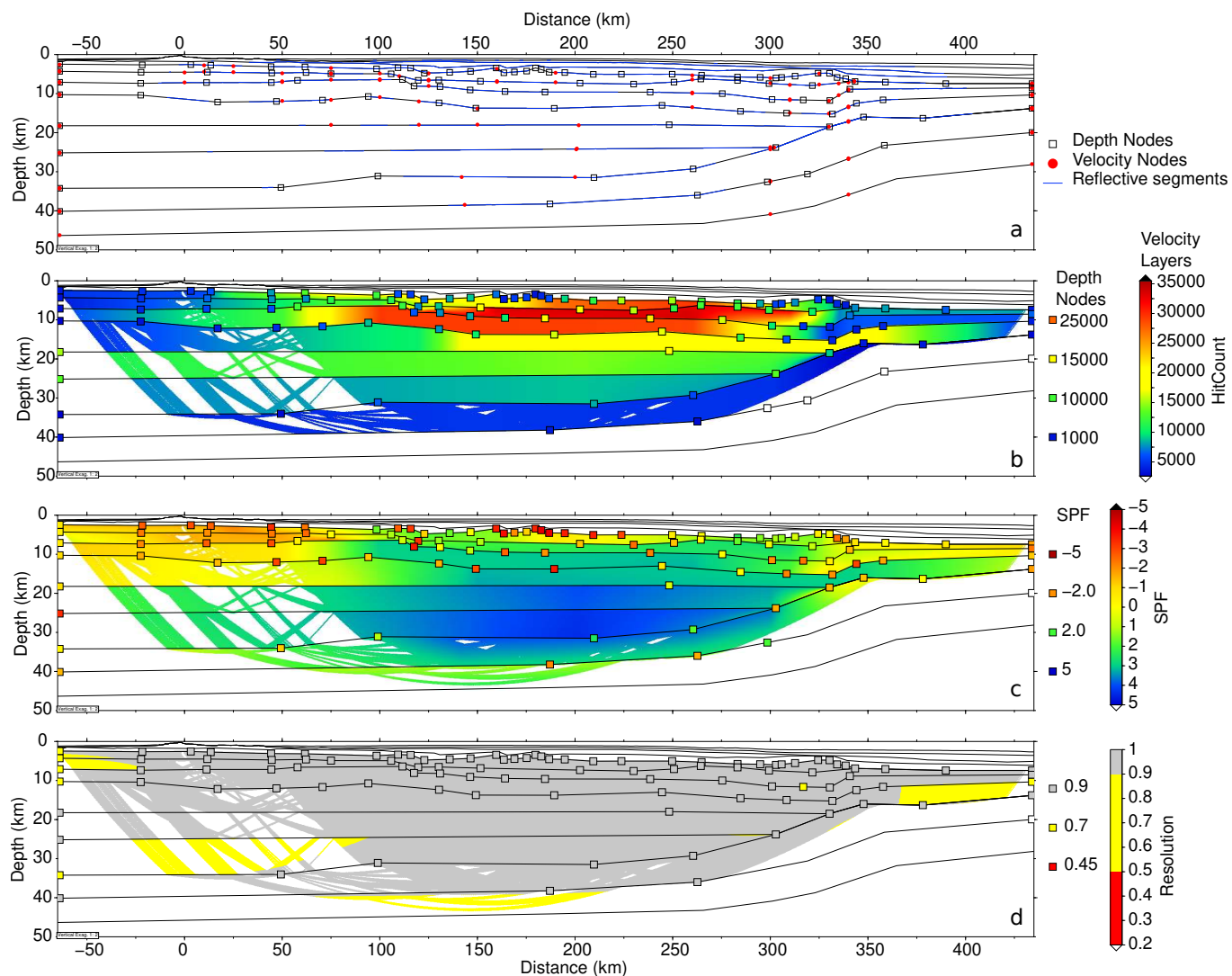
Figure 10. Evaluation of the wide-angle model MZ3. a) Model parameters including interface depth nodes (squares), top and bottom layer velocity nodes (red circles); interfaces where reflections have been observed on OBS data are highlighted in blue. b) Hit-count for velocity (colored) and depth nodes (squares). c) Smearing from Spread-Point Function (SPF) for velocity (colored) and depth nodes (squares). d) Resolution of velocity (colored) and depth nodes (squares). Zones that were not imaged are blanked.
