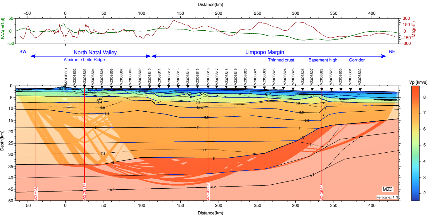
Figure 13. MZ3 Final P-wave velocity model with region constrained by seismic rays highlighted. Blue lines indicates where wide-angle reflections constrain the model interfaces otherwise in black lines. Inverted black triangles marks OBS positions. Vertical exaggeration is 1:3.
