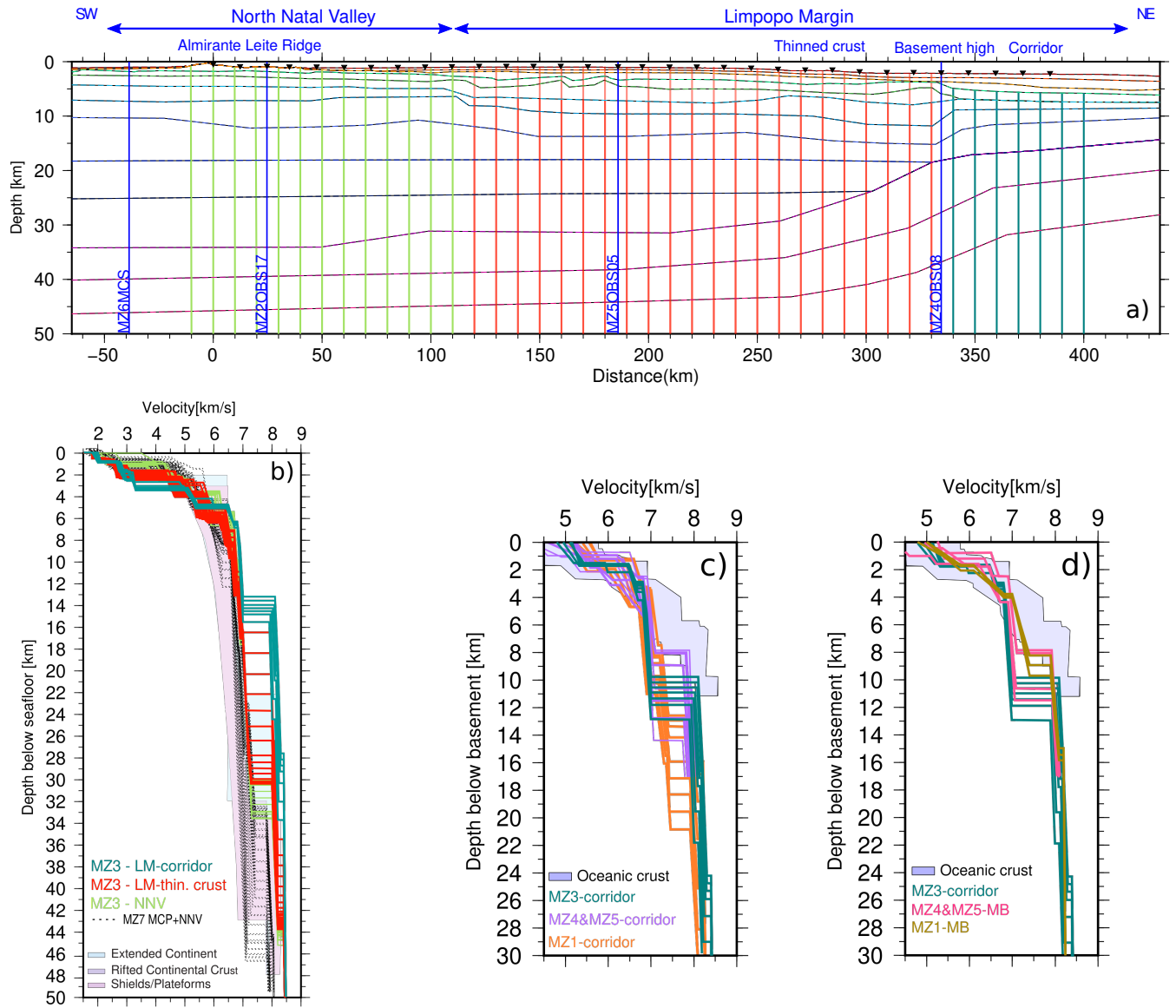
Figure 16. a) 1-D velocity-depth ( v_z ) profiles extracted along MZ3 final velocity model and color coded according to main domains and segments. b) MZ3 v_z profiles below seafloor compared to MZ7 v_z profiles of the MCP and NNV, and compiled v_z profiles of continental crust for different settings (Christensen and Mooney, 1995). c) Comparison of v_z profiles below the acoustic basement of the corridor of anomalous crust extracted from MZ1 (Moulin et al., 2020; Schnürle et al., 2018), MZ3 (this study), MZ4 and MZ5 (Watremez et al.) models with a compilation of v_z from ‘normal’ Atlantic oceanic crust (White et al., 1992). d) Comparison of MZ3 v_z profiles below the acoustic basement of the corridor of anomalous crust with v_z for the oceanic crust of the MB extracted from MZ1 (Moulin et al., 2020; Schnürle et al., 2018), MZ4 and MZ5 (Watremez et al.) and compared to the compilation of (White et al., 1992).
