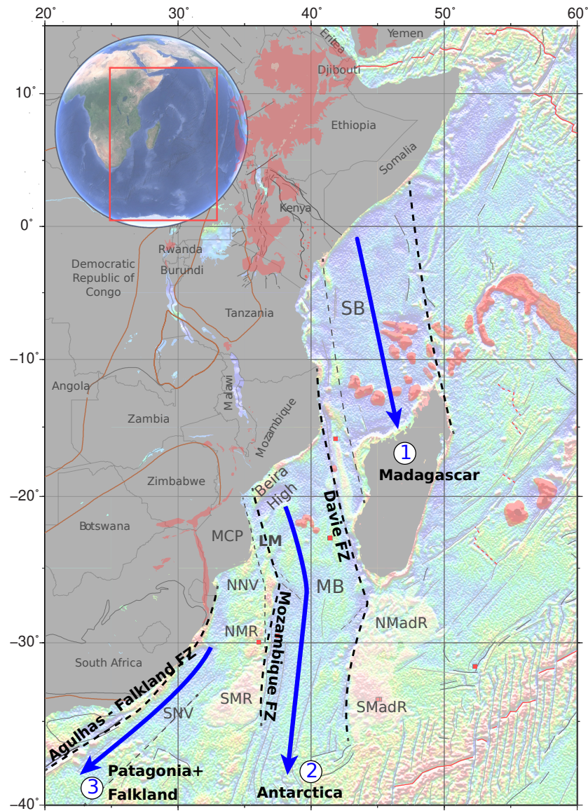
Figure 1. Free-air satellite-derived gravity anomaly of the Mozambique Channel (Sandwell et al., 2014) showing the complexity and segmentation of the East African margin (modified from Thompson et al. (2019)). Segments 1 and 2 correspond respectively to the movement of the Madagascar and Antarctica tectonic plates that opened the Somalie Basin (SB) and the Mozambique Basin (MB). The segment 3 corresponds to the drifting of the Falkland and Patagonian plates that opened the South Natal Valley (SNV). NNV=North Natal Valley; MCP=Mozambique Coastal Plain; NMR=North Mozambique Ridge; SMR=South Mozambique Ridge; NMadR=North Madagascar Ridge; SMadR=South Madagascar Ridge. Our study area is the Limpopo margin (LM, in bold). In red is volcanism without distinction about the age; black lines are major tectonic features; and brown lines denote craton contours (Mercator projection).
