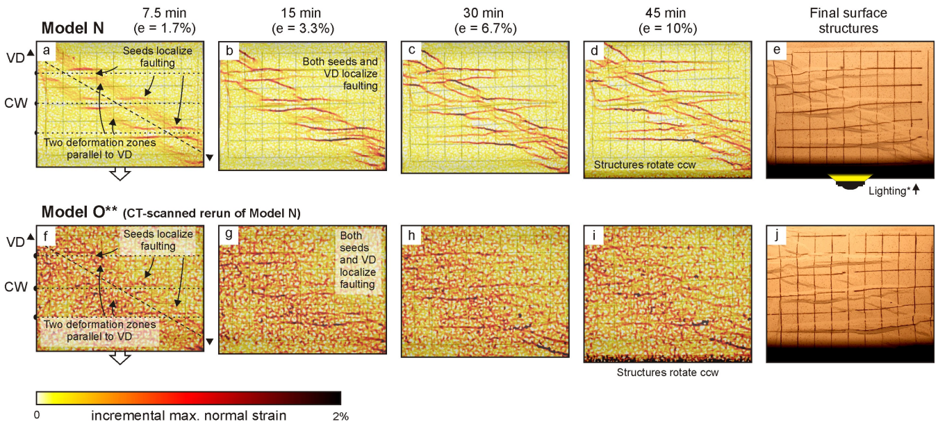
435 Fig. 9. Incremental maximum normal strain maps of models N and O from Sub-series 2.3 (with 30° oblique VD, model axis- parallel weaknesses in the brittle cover and a double extension velocity of 40 mm/h, compare to reference models G and H, Fig. 5a- j) obtained through PIV analysis, taken as a proxy of fault activity. The increments for PIV analysis were 1 min, i.e. every 0.33 mm of extension. The original models map view pictures are visible in the background. The right-hand column depicts the model surface at the end of each experiment. VD: velocity discontinuity; CW: (simulated) crustal weakness, ccw: counter-clockwise, * shadows cast by one-sided lighting allowing a better visualization of the final surface structures, ** due to technical issues, the PIV 440 analysis of Model O is less detailed.
