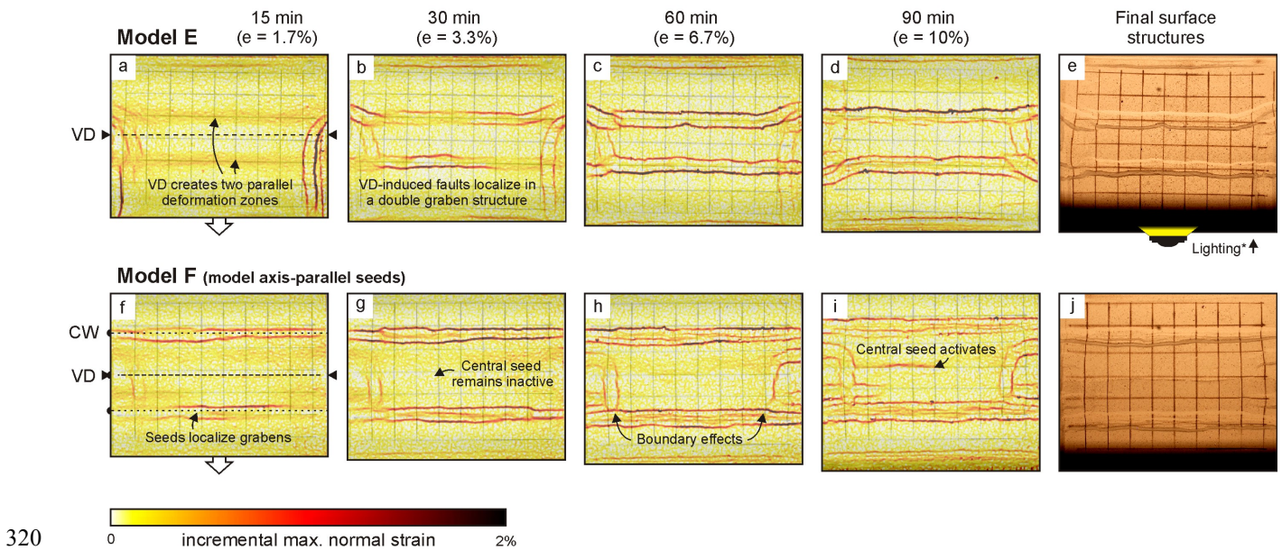
Fig. 4. Incremental maximum normal strain maps of Sub-series 1.2 models (with model axis-parallel VD, and equally oriented seeds, if applied) obtained through PIV analysis, taken as a proxy of fault activity. Note that these models have a thicker (1.5 cm) viscous layer and a thinner (2.5 cm) brittle cover than the other models in this paper (standard layering being 3 cm of brittle material on top of 1 cm of viscous material). The increments for PIV analysis were 1 min, i.e. every 0.33 mm of extension. The original model map view pictures are visible in the background. Note that Model F includes a crustal weakness (seed) above and parallel to the VD. The right-hand column depicts the model surface at the end of each experiment. The final column depicts the model surface view at the end of each experiment. VD: velocity discontinuity; CW: (simulated) crustal weakness, * shadows cast by one-sided lighting allowing a better visualization of the final surface structures
