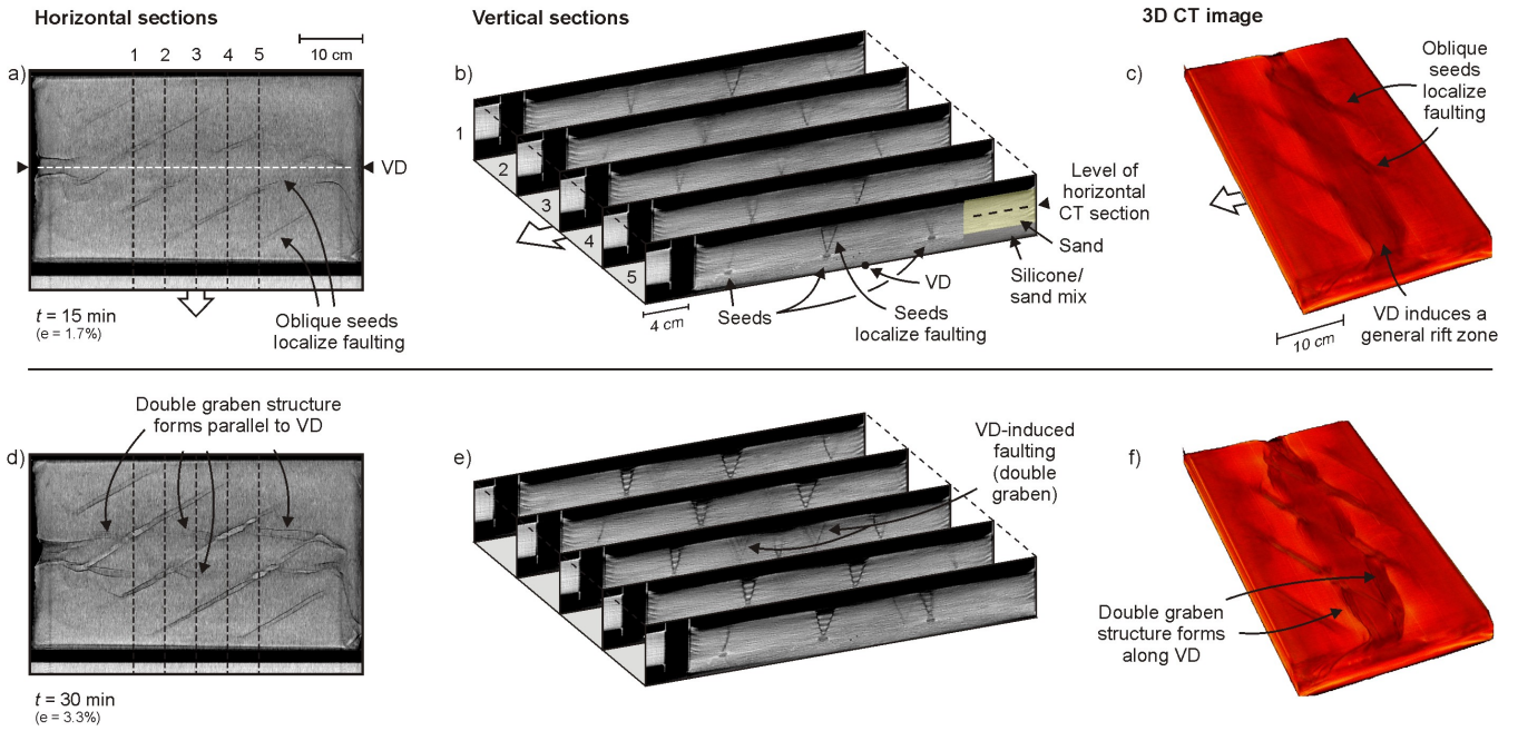
305 Fig. 3. CT analysis of Model D (model axis-parallel VD, -30^\circ oblique seeds, CT-scanned rerun of Model C). Left column: horizontal sections through the brittle layer. Middle column: serial cross-sections. Right column: 3D CT images. Note that the colours in these images represent CT-scanning intensities and are not to be interpreted as a measure of model surface altitude.
