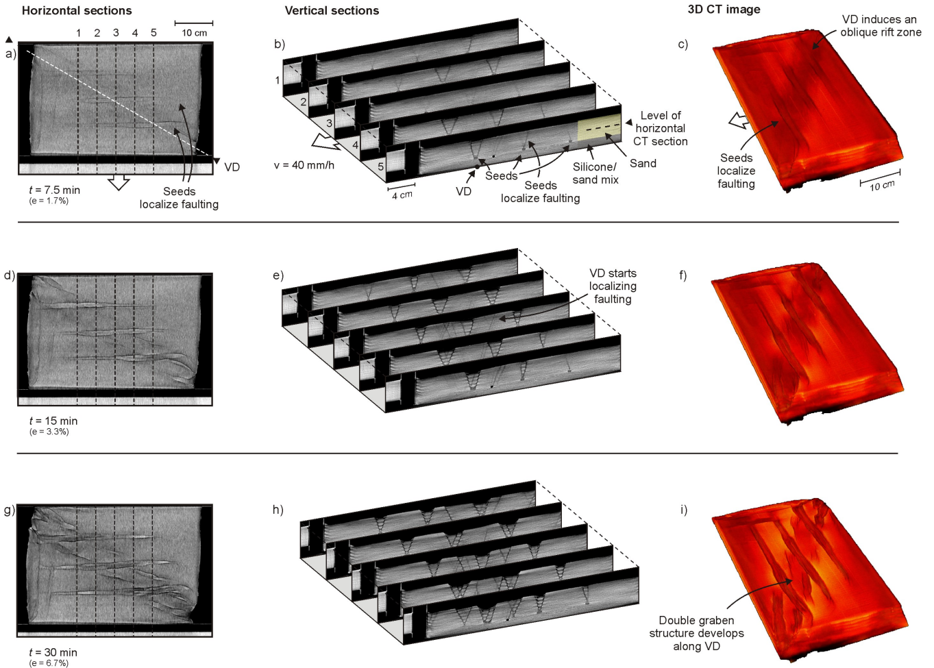
450 Fig. 10. CT analysis of Model O ( 30^\circ oblique VD, model axis-parallel seeds, doubled extension velocity, CT-scanned rerun of Model N). Left column: horizontal sections through the brittle layer. Middle column: serial cross-sections. Right column: 3D CT images. Note that the colours in these images represent scanning intensities and are not to be interpreted as a measure of model surface altitude.
