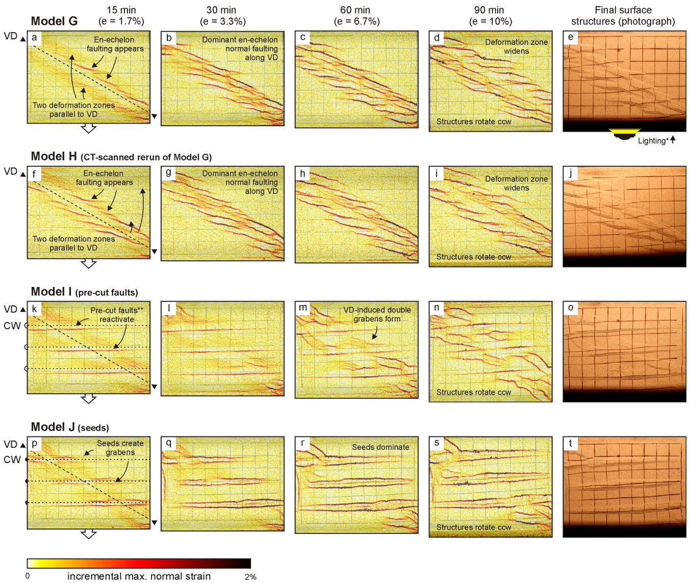
350 Fig. 5. Incremental maximum normal strain maps of models G-J from Sub-series 2.1 (with 30° oblique VD and model axis-parallel crustal weaknesses in the brittle cover, if applied) obtained through PIV analysis, taken as a proxy of fault activity. Note that these models have a thicker (1.5 cm) viscous layer and a thinner (2.5 cm) brittle cover than the other models in this paper. The increments for PIV analysis were 1 min, i.e. every 0.33 mm of extension. The original model map view pictures are visible in the background. The right-hand column depicts the model surface at the end of each experiment. VD: velocity discontinuity; CW: (simulated) crustal weakness, ccw: counter clockwise, * shadows cast by one-sided lighting allowing a better visualization of the final surface structures, ** the location of the pre-cut faults at the base of the sand layer are indicated, the offset of their surface expression is due to their inclination (Fig. 1b). 355
