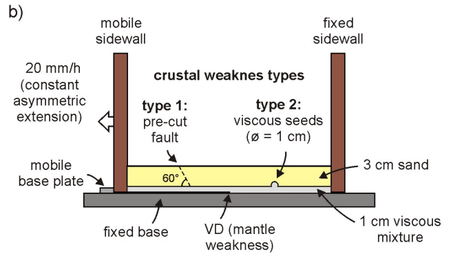
section view of model set-up
