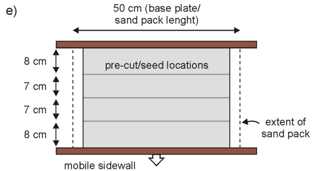
Simulated crustal weakness geometries (top view)
