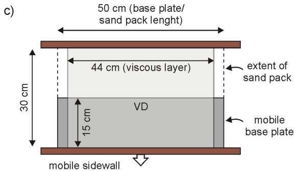
Model set-up and base plate (VD) geometries (top view)
