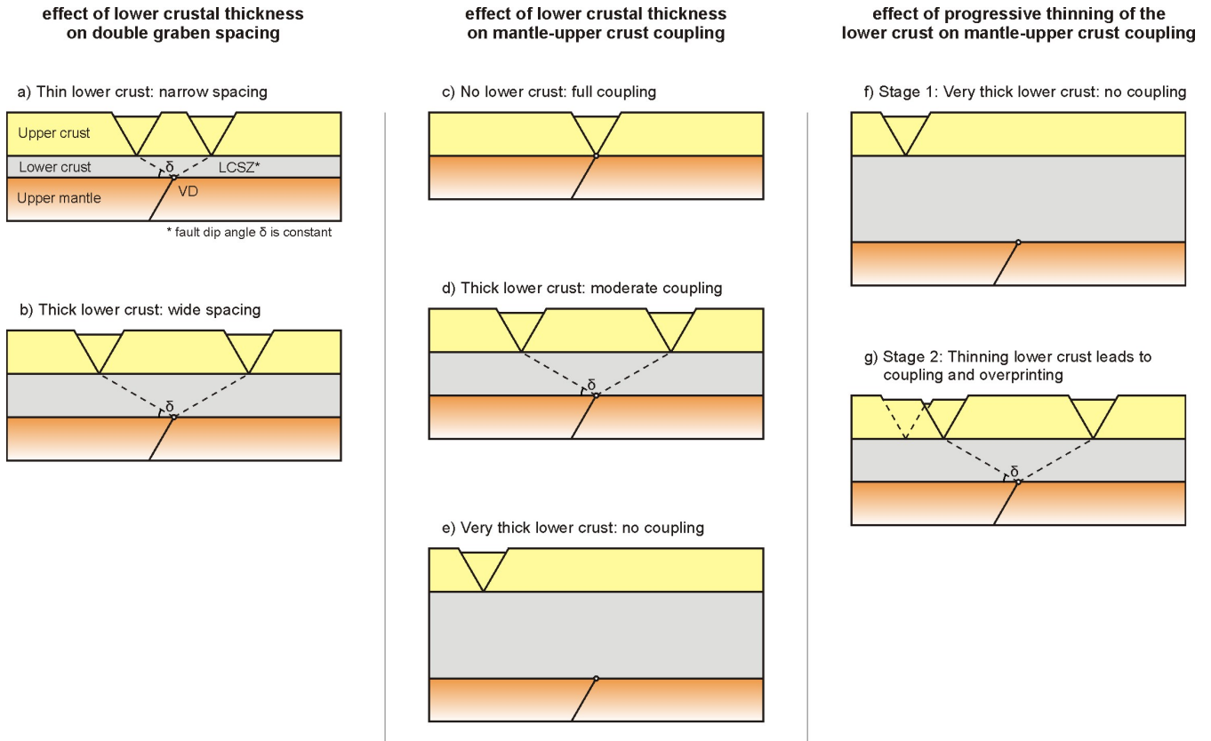
530 Fig. 12. Schematic 2D sketches depicting how lower crustal thickness variations may affect rift structures. (a-b) A thicker lower crust widens the spacing between double grabens related to lower crustal shear zones (LCSZ) originating from a mantle shear zone simulated by a velocity discontinuity (VD) in our models. (c-e) The degree of coupling between the mantle and crust is strongly affected by lower crustal thickness: the thicker the lower the crust, the less coupling occurs. When no coupling occurs, deformation in the upper crust can localize along crustal weaknesses only (e.g. Zwaan et al. 2019). Note however that coupling is also affected by extension velocity (e.g. Brun 1999; Zwaan et al. 2019, see Models F, G, N, O, Figs. 5a-j, 9, 11i, k). (f-g) Progressive 535 thinning of the lower crust during rifting may cause a previously decoupled system to become coupled, so that previous upper crustal weakness-controlled structures may be overprinted by mantle-weakness controlled structures.
