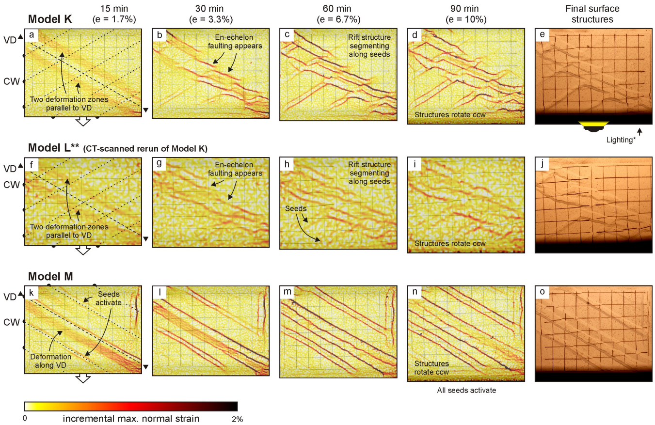
405 Fig. 7. Incremental maximum normal strain maps of models K-M from Sub-series 2.2 (with 30° oblique VD and oblique seeds in the brittle cover) obtained through PIV analysis, taken as a proxy of fault activity. Note that these models have a thicker (1.5 cm) 410 viscous layer and a thinner (2.5 cm) brittle cover than the other models in this paper. The increments for PIV analysis were 1 min, i.e. every 0.33 mm of extension. The original model map view pictures are visible in the background. The right-hand column depicts the model surface at the end of each experiment. Note that Model M includes a crustal weakness (seed) above and parallel to the VD. VD: velocity discontinuity; CW: (simulated) crustal weakness, ccw: counter clockwise, * shadows cast by one-sided lighting allowing a better visualization of the final surface structures, ** due to technical issues, the PIV analysis of Model L is less detailed.
