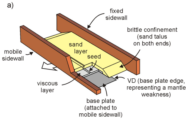
3D cut-out sketch of model set-up
