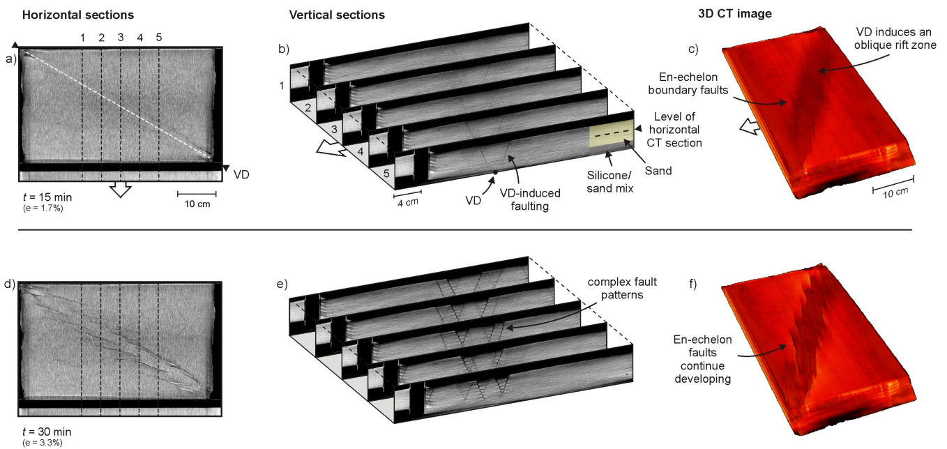
Fig. 6. CT analysis of Model H (30° oblique VD, no crustal weaknesses simulated, CT-scanned rerun of Model G). Left column: horizontal sections through the brittle layer. Middle column: serial cross-sections. Right column: 3D CT images. Note that the colours in these images represent CT-scanning intensities and are not to be interpreted as a measure of model surface altitude.
