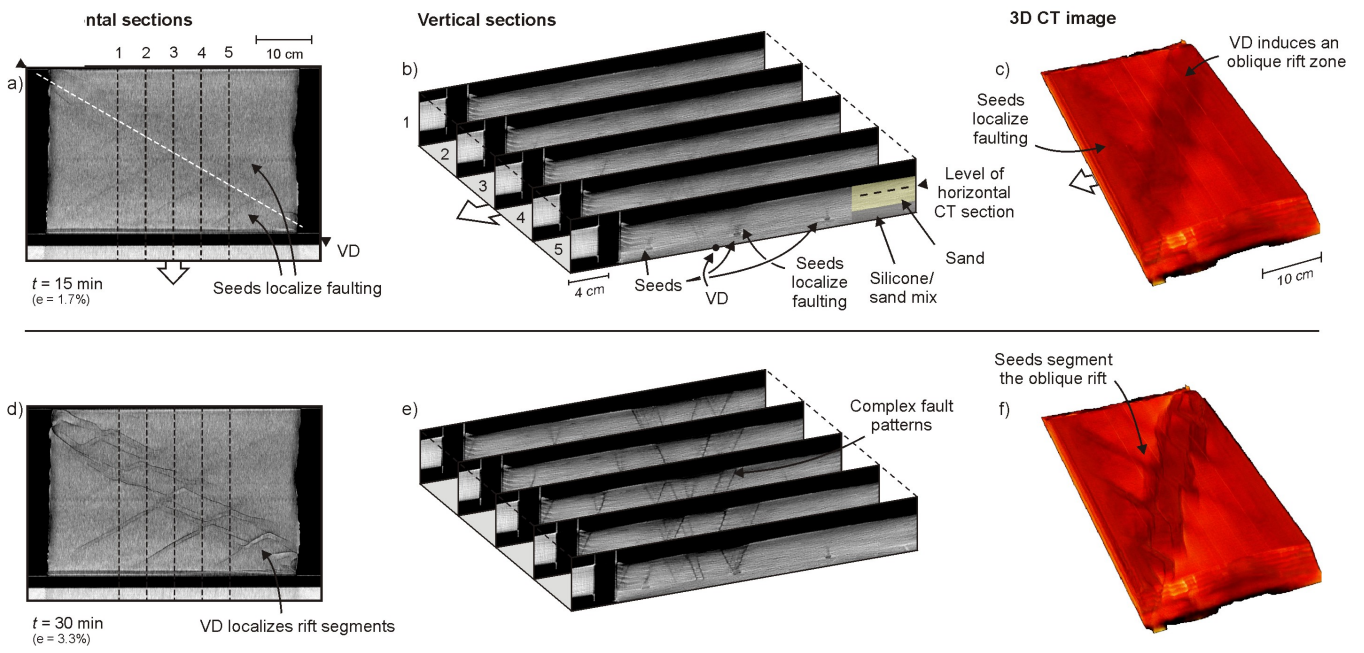
Fig. 8. CT analysis of Model L (30° oblique VD, -30° oblique seeds, CT-scanned rerun of Model K). Left column: horizontal sections through the brittle layer. Middle column: serial cross-sections. Right column: 3D CT images. Note that the colours in these images represent CT-scanning intensities and are not to be interpreted as a measure of model surface altitude.
