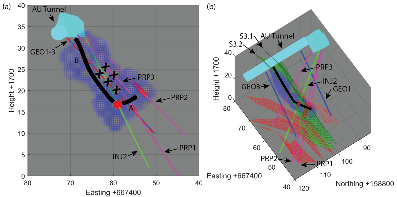
Figure 11. Interpretation of the tracer flow path reconstruction. a) Side view. The tracer indicated with the black arrows passes through the GEO plane (red/blue) at two locations, labeled A and B. b) Reconstructed flow path along with the shear zones S3 (green) and S1 (red) in the experiment volume. The PRP intervals are indicated in red.
