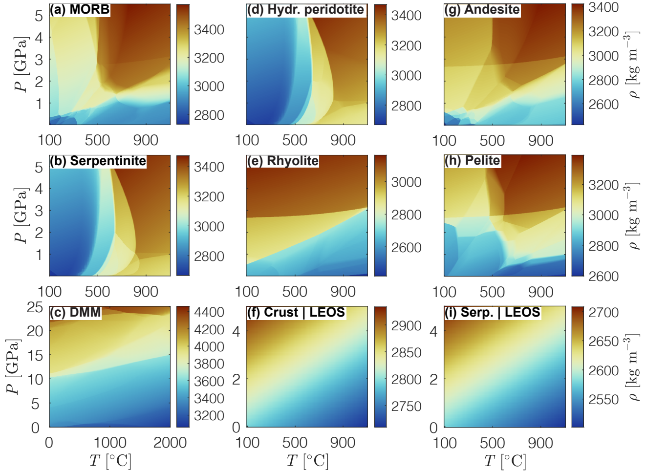
Figure 3. Density structures employed in the models presented here. (a)-(e) And and g )-(h): Phase diagram density fields calculated with Perple_X for the bulk rock compositions given in tab. 2. (f) And and (i): Density fields calculated using a linearized equation of state (Eq. A3) for an upper crustal reference density of 2800 kg m -3 and a serpentinite reference density of 2585 kg m -3 , respectively.
