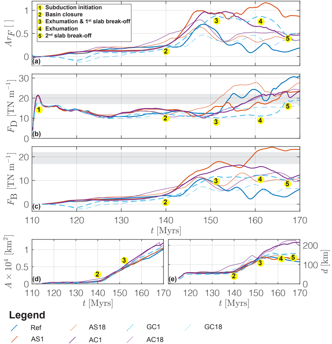
Figure 11. Force evolution. (a) Ratio of buoyancy and force to shear force, Ar_F , (b) Shear forces, (c) buoyancy forces, (d) average area of subducted material and (e) maximum depth of the orogenic wedge subducted crust. Detailed explanation on calculation of quantities see appendix C. Numbering in a panels exemplified for model GC1: 1 = onset of subduction initiation, 2 = basin closure and onset of continental subduction, 3 = onset of continental crustal exhumation and first slab detachment, 4 = onset of the second exhumation event and 5 = onset of the second slab detachment.
