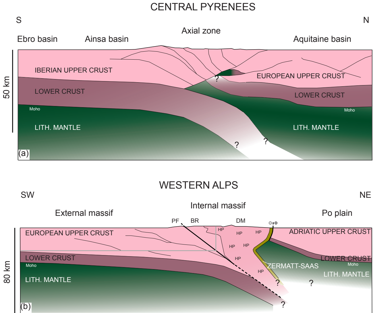
Figure 1. Tectonic-Simplified tectonic cross sections: (a) Across the Central Pyrenees, modified after Teixell et al. (2018) and (b) across the Western Alps, modified after Zhao et al. (2015) and Schmid et al. (2017). Light violet represents the upper crust, dark violet represents the lower crust and green represents the mantle lithosphere. The region of mixed violet and green in (a) represents an unit of lower crust or mantle thrust slices. Black lines indicate unit boundaries and the grey line in (b) indicates the domain captured by most crustal wedge models (compare to f.e. Malavieille, 2010; Dal Zilio et al., 2020b). Abbreviations: Penninic Front, PF, Briançonnais, BR, Dora-Maira, DM and high-pressure regions, HP.
