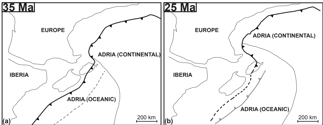
Figure 13. Plate-Simplified plate reconstruction of Europe, Iberia and Adria at (a) 35 Ma and (b) 25 Ma. Europe and Iberia are fixed, Adria is moving northward. Thick black and grey solid lines indicate active subduction zones, dashed lines indicate inactive subduction zones. Sketches modified after Schmid et al. (2017) & Malusà et al. (2015).
