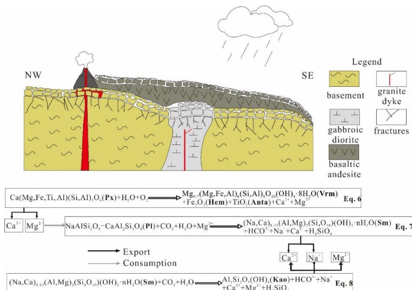
Fig. 14. Reconstructed alteration model of GA1 well in Sprengler Horst after volcanic eruption around 290 Ma; Abbreviations: Px-pyroxene.
