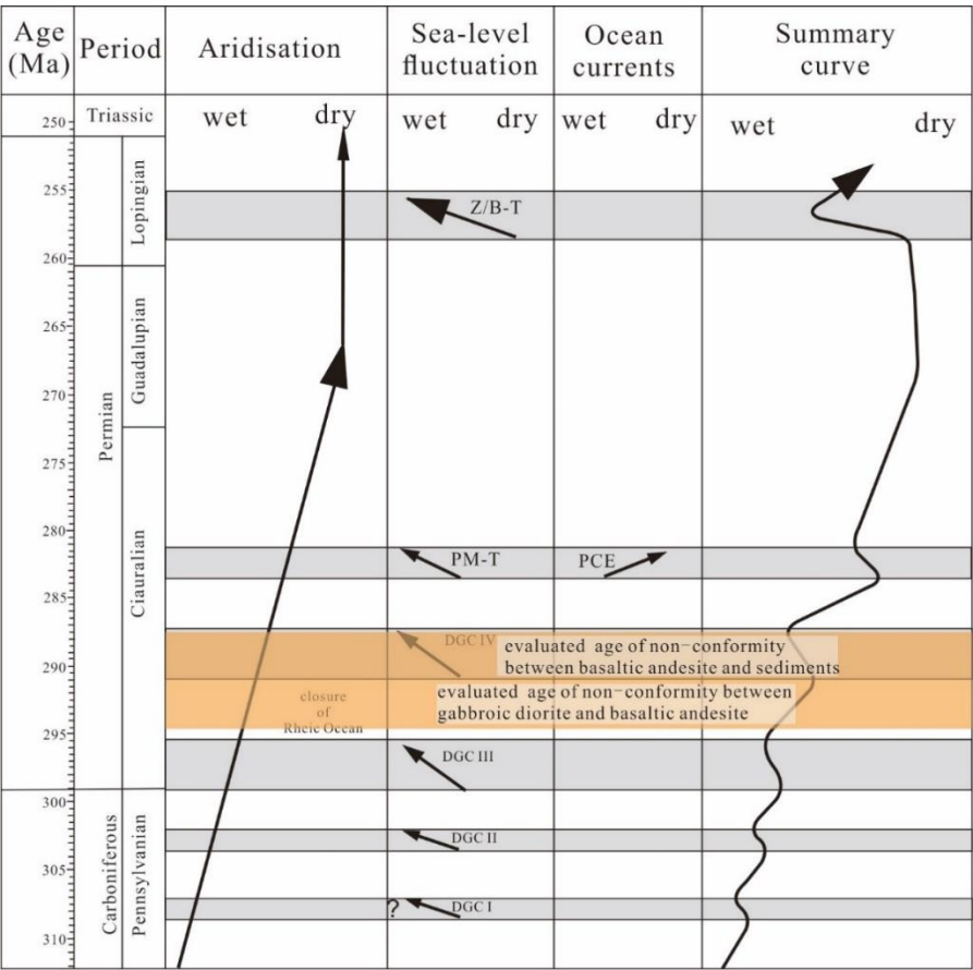
Fig. 12. Climate variation in Central Europe (modified after Roscher and Schneider (2006)), DGC- Deglaciation Cycle of Gondwana Icecap, PM-T, Pietermaritzburg Transgression; Z/B-T, Zechstein/Bellerophon Transgression; PCE, Permian Chert Event.
