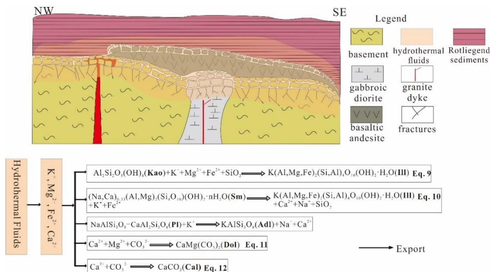
Fig. 15. Reconstructed alteration model of GAI well in Sprendlinger Horst during burial in the Jurassic and Cretaceous; Abbreviations: Adl- adularia.
