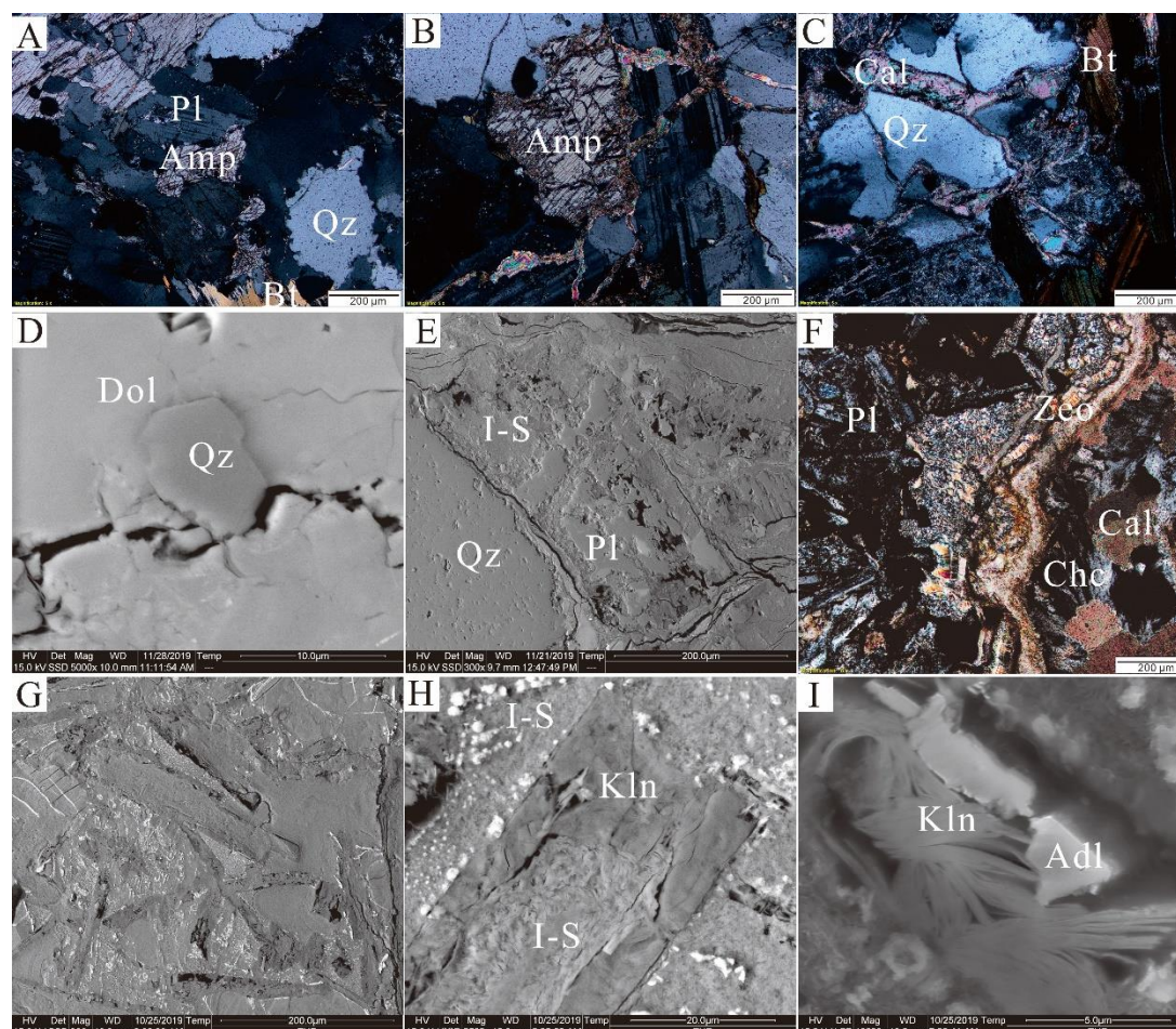
Fig. 2. Petrographic characteristic of the basement and the overlying volcanic rock in the GA1 drill core. (A) fresh gabbroic diorite (PM, z = 55.5 m); (B) gabbroic diorite (PM, z = 27.1 m), slightly weathered amphibole; (C) gabbroic diorite (PM, z = 20.6 m), fractured quartz grain; (D) gabbroic diorite (BSE, z = 21.5 m), dolomite accompanied by quartz; (E) gabbroic diorite (BSE, z = 20.6 m), partly weathered plagioclase. (F) basaltic andesite (PM, z = 17.8 m), fresh plagioclase grains with the amygdaloid consists of calcite and zeolite and chalcedony; (G) basaltic andesite (BSE, z = 13.9 m) secondary clay minerals with intact primary grain shapes; (H) basaltic andesite (BSE, z = 13.9 m), I/S surrounded by kaolinite within one residual plagioclase grain shape; (I) basaltic andesite (SEM, z = 13.9 m), kaolinite and adularia filled in void; Abbreviations: PM- polarizing microscopy; z -depth below ground surface; Amp-amphibole; Kln-kaolinite; Adl-adularia; Bt-biotite; Cal-calcite; Pl-plagioclase; Zeo-zeolite; Chc-chalcedony; Dol-dolomite; Qz-quartz.
