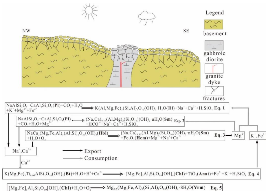
Fig. 13. Reconstructed alteration model of GA1 well in Sprengler Horst before volcanic eruption around ca. 300 Ma; Abbreviations: Anat- anatase; Bt-biotite; Chl-chlorite; Hbl-hornblende; Hem-hematite; Ill-illite; Pl-plagioclase; Sm-smectite; Vrm-vermiculite.
