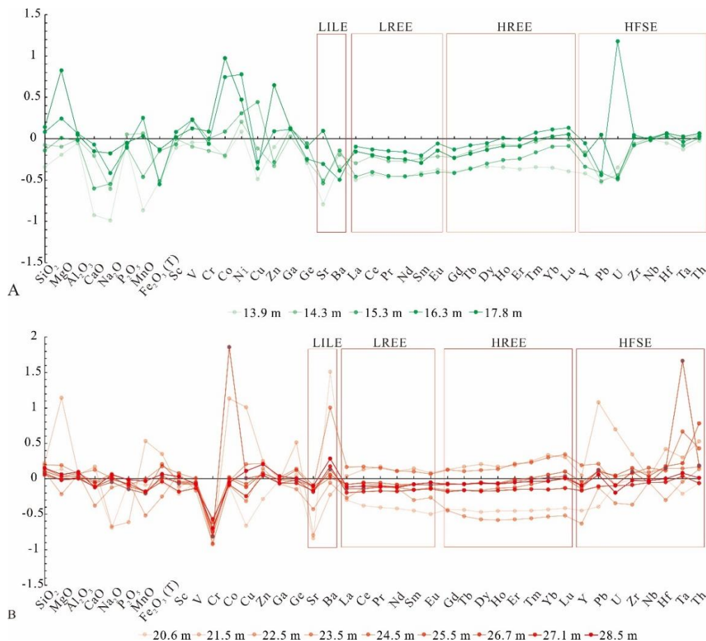
Fig. 10. \tau value features of basaltic andesite (A) and gabbroic diorite (B) in GA1 well
