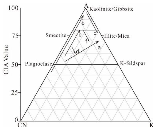
Fig. 11. Theoretical weathering tendency and retrograde tendency during burial diagenesis (Fedo et al., 1995), a-observed weathering trend for both basaltic andesite and gabbroic diorite; b-theoretical weathering trend for basaltic andesite; c-retrograde trend of topmost basaltic andesite; d-retrograde trend of the rest part of basaltic andesite; e-theoretical weathering trend for gabbroic diorite; f-retrograde trend for gabbroic diorite.
