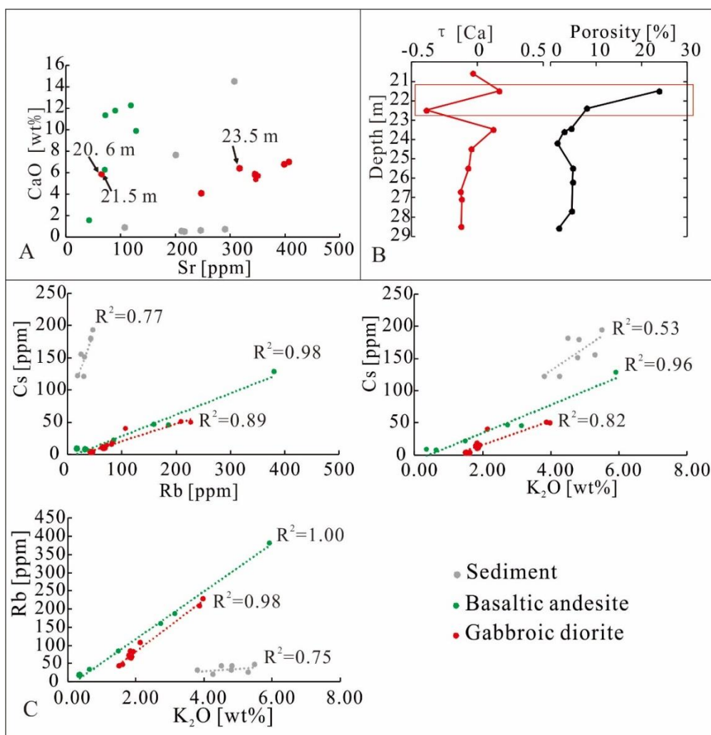
Fig. 9. Elements characteristic, (A) CaO-Sr cross-plot of the samples from the GA1 drill core; (B) Relationship between the \tau value and the porosity in the gabbroic diorite; (C) Relationship among Rb, Cs and K 2 O among sedimentary rocks, basaltic andesite and gabbroic diorite.
