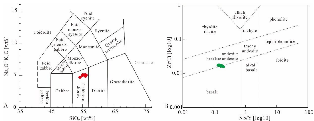
Fig. 4. Classification of rocks of the GA1 well with the TAS diagram and Revised Winchester-Floyd diagram. (A) samples from fresh and nearly fresh parts of basement; (B) samples from overlain lava profile
