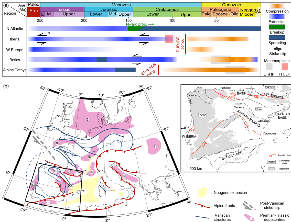
Figure 1. TS2 Geodynamic chart and localization of the study area. (a) Geodynamic chart of the main structural areas of the Iberian domain. BCB: Basque–Cantabrian Basin. (b) Location map of western Europe, showing the areas that are deformed in compression and extension and Permian–Triassic depocentres. (1) French Massif Central; (2) Aquitaine Basin and Pyrenees; (3) Germanic Basin; (4) southeastern France; (5) Iberian Basin; (6) Italy; (7) central Europe; (8) English Channel; (9) northeastern France; (10) Basque–Cantabrian Basin; (11) Betics; (12) West Iberia. Inset: Map of Iberia showing the main structures and transforms (red) and sedimentary basins (capitalized and italicized text) and sub-basins (italicized text). BC: Basque–Cantabrian; HTF: High Tagus Fault; MPF: Messejana–Plasencia Fault; NF: Nazaré Fault; NPF: North Pyrenean Fault; PYR: Pyrenean; UF: Ubierna Fault; VF: Ventaniella Fault; ZOF: Zamanza–Oña Fault.
