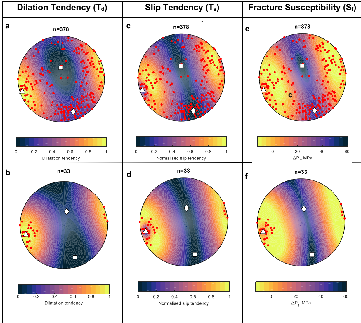
Figure 09. Lower hemisphere equal area projection for dilation tendency, slip tendency and fracture susceptibility in a given fluid pressure condition and for a specific stress state (Fractend code available via Github, 2017). (a) and (b) represents dilation tendency for high and low P_f . (c) and (d) represents slip tendency for high and low P_f . (e) and (f) fracture susceptibility for high and low P_f conditions respectively. Warm color zones in (a) and (b), represents vein orientations with higher propensity for tensional opening. In (c) and (d) warm colors indicate vein attitudes that suffered shearing. In (e) and (f) the warm color zones stand for vein attitudes that are more susceptible to reactivate under low P_f variation. ‘Thermal’ color scheme from Thyng et al., 2016. White square ( \sigma_1 ), white diamond ( \sigma_2 ) and white triangle ( \sigma_3 ).
