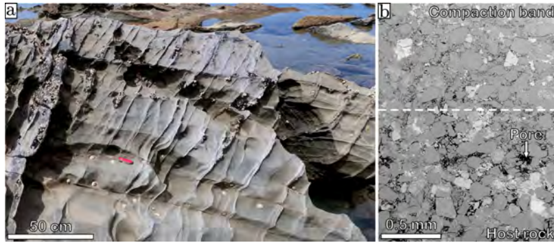
Figure 3. a) Photograph of three generations of shear-enhanced compaction bands and pure compaction bands in silt- and sandstones of the Miocene Whakataki Formation, South of Castlepoint, North Island, New Zealand. These deformation bands formed during the slow compression of the Hikurangi subduction wedge (see Elphick et al. (2021) for details). The positive relief of the metre-long bands is caused by the significant porosity reduction relative to the host rock, which renders them less susceptible to erosion. The dominant microphysical deformation mechanism for inelastic volume loss is grain crushing (see panel (b)). The bands possibly formed by hydro-(chemo)-mechanical coupling, which can explain the relatively short (diffusive) length scales (Hu et al., 2020). The regular, constant spacing may be indicative of the standing-wave phenomenon (Regenauer-Lieb et al., 2013a; Veveakis and Regenauer-Lieb, 2015). (b) Scanning-electron micrograph, recorded with the backscattered electron detector, of a compaction band (region above the white dashed line) and its host rock in fine-grained sandstone of the Whakataki Formation. Pores appear black (the white arrow marks an example). The compaction band displays a marked reduction in porosity and contains a much larger proportion of crushed grains than the host rock.
