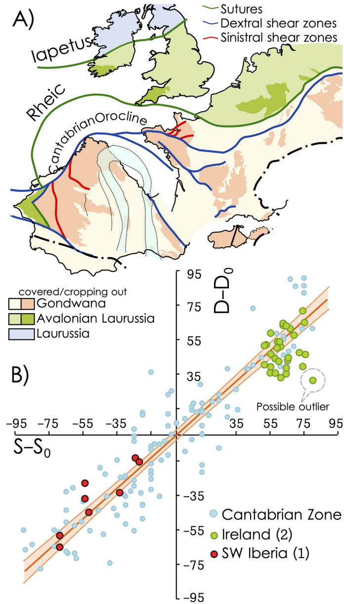
Fig. 10 Orocline test of the Cantabrian Orocline (Weil et al., 2013) compared with the magnetizations found in the adjacent Laurussian segments of the orogen: Ireland (Pastor-Galán et al., 2015b) and the South Portuguese Zone (Leite Mendes et al., in press )
