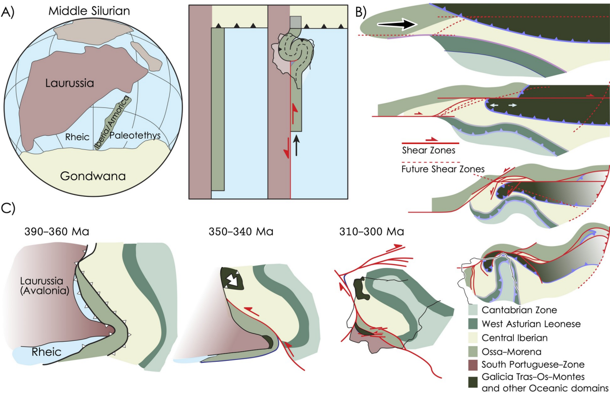
1688 Fig. 11 Pioneering hypotheses for the Central Iberian curve. Note that none of them fulfill 1689 the most recent geometric and kinematic criteria. A) Simplified ribbon continent model after 1690 Johnston et al. (2013) and Shaw and Johnston (2016). B) Dextral mega-shear model from 1691 Martínez-Catalán (2011). C) Kinematic model with indentation and left-lateral shearing after 1692 Simancas et al. (2013)
