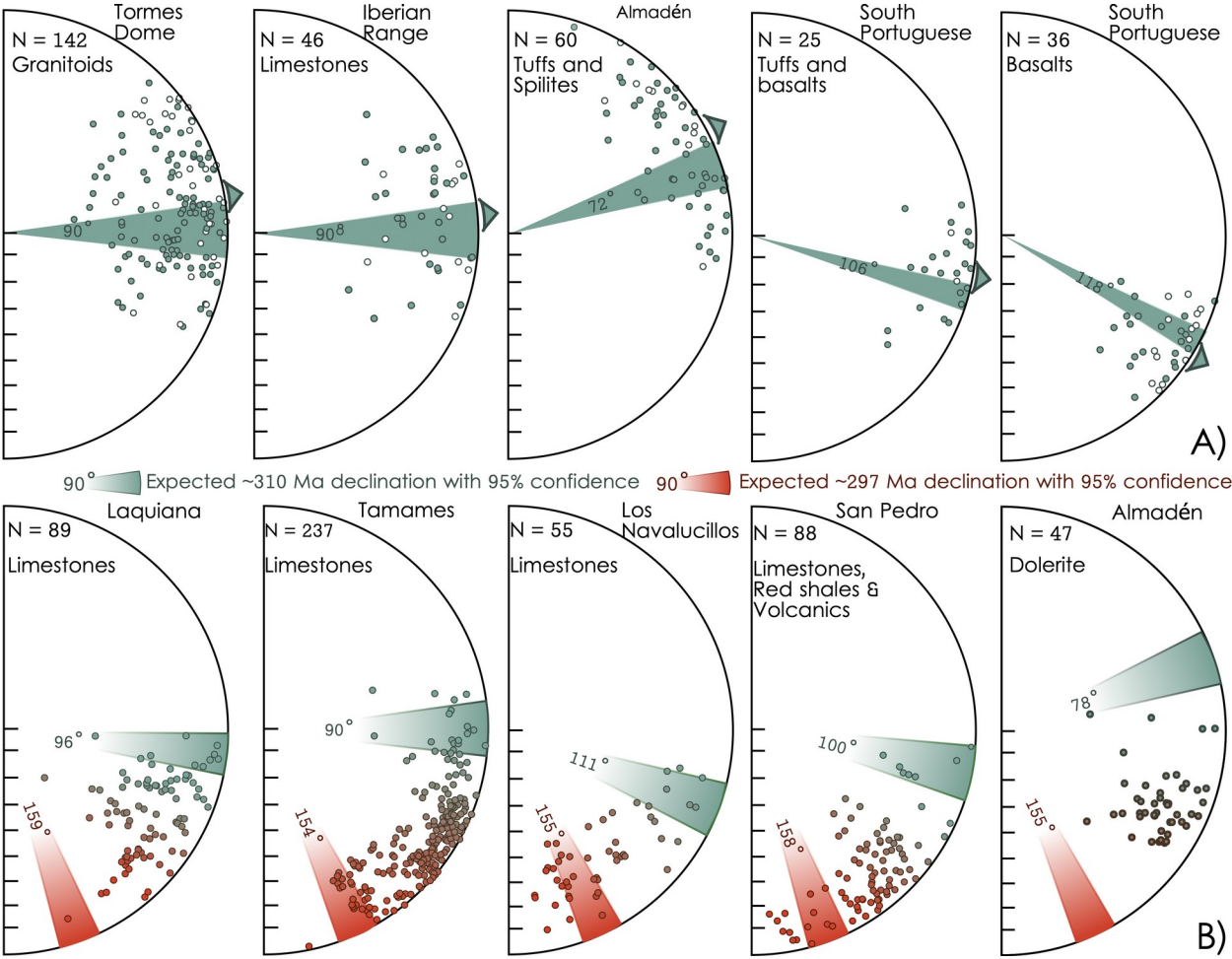
Fig. 9 Compilation of the directional distributions and average declinations with parachute of confidence ( \Delta Declination) in sites around the Central Iberian curve (see Fig. 6). The results show general CCW rotations in contrast to the expected CW rotations if the Central Iberia curve formed by vertical-axis rotations (see text). Results are compared with the expected declinations if those sites were part of the Cantabrian Orocline following the methodology described in Pastor-Galán et al. (2017b).
