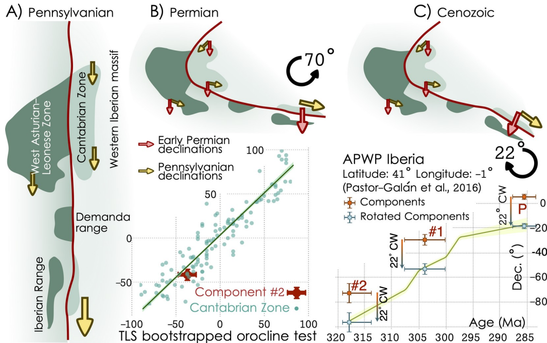
Fig. 8 Cartoon depicting the different vertical-axis rotation events that occurred in the Cantabrian Zone and the Iberian Range, modified from Pastor-Galán et al. (2018). (A) Original quasilinear Variscan Orogenic belt, B) Formation of the Cantabrian Orocline around the Carboniferous–Permian boundary after a \sim 70^\circ counterclockwise rotation in the Southern branch of the Cantabrian Zone and the Iberian Range. This rotation matches the rotation for the Cantabrian Orocline, see the fit of the Iberian Range Component #2 in the orocline test for the Cantabrian Zone (below). C) Post-Permian (Cenozoic) rotation of \sim 22^\circ clockwise (CW) likely produced by differential shortening during the Alpine orogeny (Izquierdo-Llavall et al., 2018). Below, the global magnetic polarity time-scale for the Pennsylvanian and Cisuralian (following Ogg et al., 2016). TLS = Total Least Squares. Note that once the 22^\circ CW rotation in the Iberian Range is corrected, components #2, #1, and P fit as expected with the APWP for the southern limb of the Cantabrian Orocline (Pastor-Galán et al., 2016).
