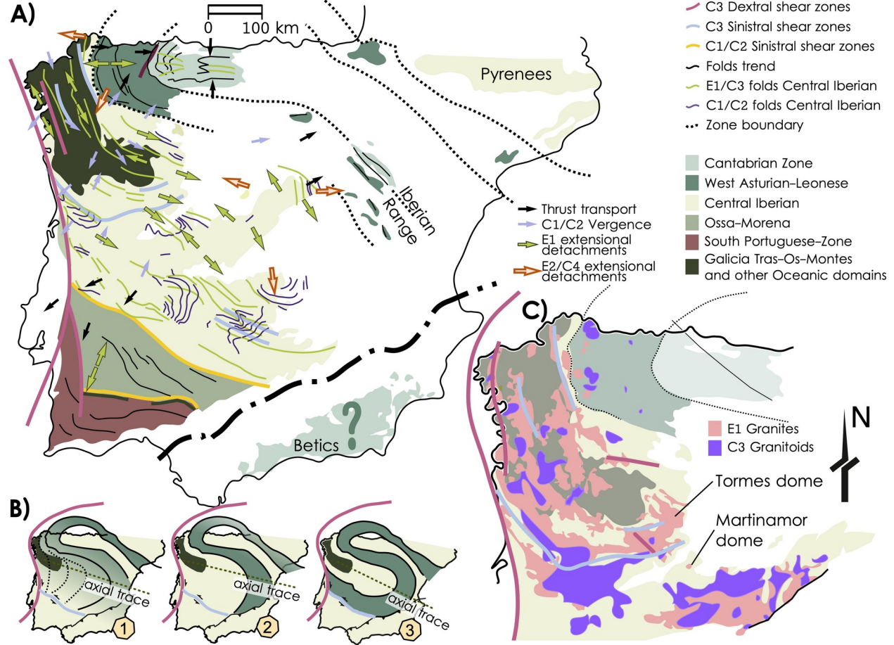
Fig. 2 A) Present-day configuration of the tectonostratigraphic zones of the Iberian Variscides and their major structures. White areas represent Mesozoic and Cenozoic cover. B) Three competing geometric proposals for the Central Iberian curve. 1) A disharmonic curvature, up to 160^\circ at the outer arc but much less pronounced at the inner arc (Aerden, 2004); 2) A harmonic, but more open curvature as suggested by Martínez Catalán (2012); 3) An isoclinal curvature model (Shaw et al., 2012). C) Distribution of the E1 (migmatitic domes) and C3 to post-C3 granitoids in the NW of Iberia (modified from Pastor-Galán et al., 2016)
