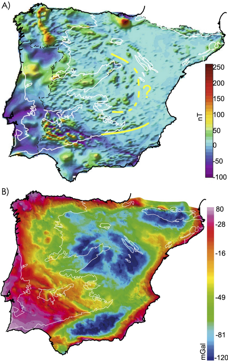
1598 Fig. 5 A) Aeromagnetic map of Spain (Ardizzone et al., 1989, for Spain and the World 1599 Digital Magnetic Anomaly Map (WDMAM project) and Portugal (modified from Martínez Catalán, 1600 2012 and Martínez Catalán et al., 2015), showing the possible trace of the Central Iberian 1601 curve. B) Bouguer anomalies of the Iberian Peninsula, modified from Ayala et al., 2016. Gravity 1602 anomalies do not reflect the geometry of the Cantabrian Orocline nor the Central Iberian curve 1603 but are related to the Cenozoic Alpine lithospheric structure.
