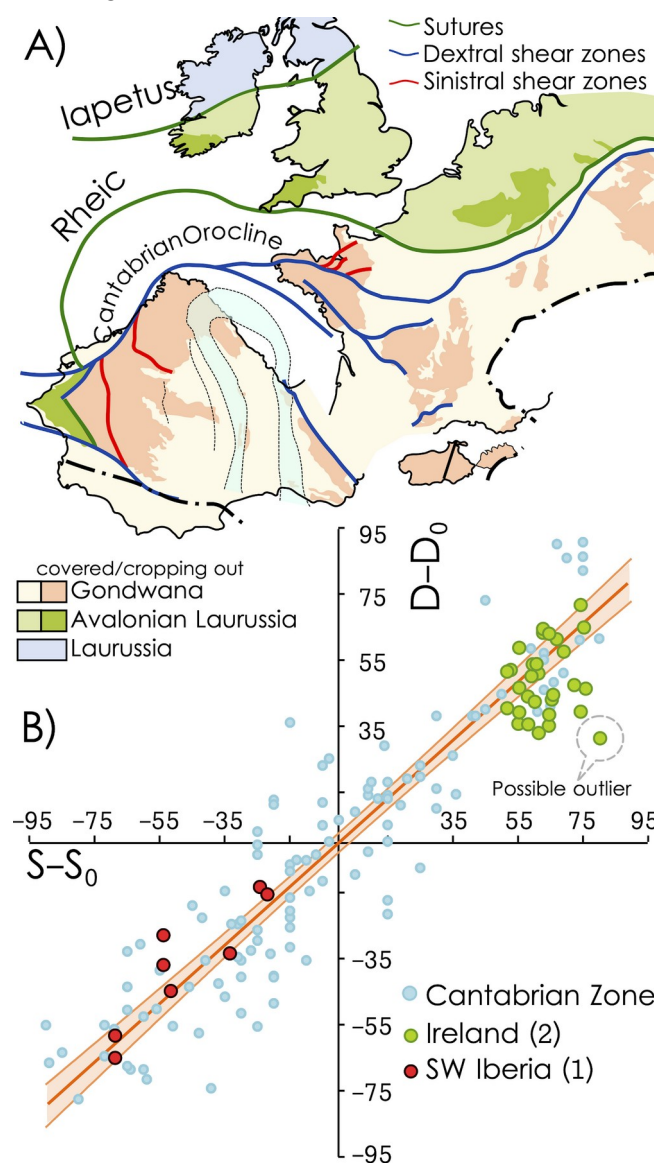
1639 Fig. 10 Orocline test of the Cantabrian Orocline (Weil et al., 2013) compared with the 1640 magnetizations found in the adjacent Laurussian segments of the orogen: Ireland (Pastor-Galán 1641 et al., 2015b) and the South Portuguese Zone (Leite Mendes et al., in press)
