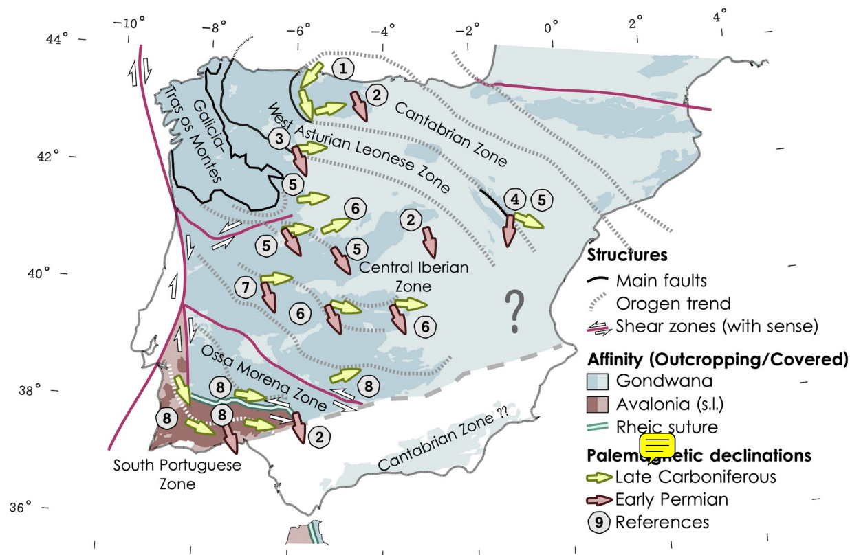
1604 Fig. 6 Paleomagnetic studies related to the Cantabrian Orocline and the Central Iberian 1605 curve: (1) Synthesis of paleomagnetism in the core of the Cantabrian Orocline (see Weil et al., 1606 2013); (2) Permian (eP) components synthesized in Weil et al. (2010); (3) Ordovician volcanics 1607 and limestones (Laquiana) in the boundary between the West Asturian-Leonese and Central 1608 Iberian Zones (Fernández-Lozano et al., 2016); (4) Devonian sedimentary sequences and 1609 Permian subvolcanics in the Iberian ranges (Pastor-Galán et al., 2018); (5) Permian dykes and 1610 sills (Calvín et al, 2014); (5) Anatectic granites (E1) and mantle derived granitoids (C3) from 1611 Tormes Dome and Central System (Pastor-Galán et al., 2016); (6) Cambrian limestones from 1612 Tamames (N) and los Navalucillos (S) (Pastor-Galán et al., 2015a); (7) Ediacaran-Early 1613 Cambrian sedimentary rocks in the southern sector of the Central Iberian Zone (Pastor-Galán et 1614 al., 2017b); (8) Almadén volcanics from the Central Iberian Zone (Perroud et al., 1991; Parés 1615 and van der Voo, 1992; Leite Mendes et al. in press) and Volcanic rocks from southern Ossa 1616 Morena and the South Portuguese Zone (Leite Mendes et al, in press)
