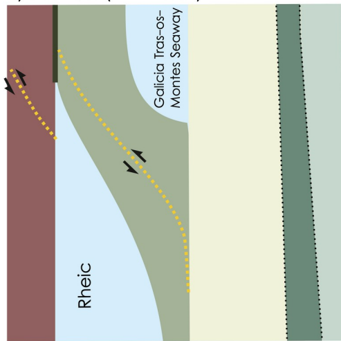
D) C3 (~315-300 Ma)
