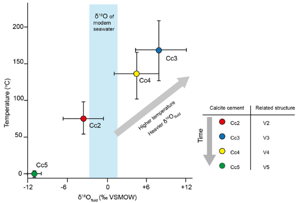
955 Figure 10: Temperatures (°C) vs \delta^{18}\text{O}_{\text{fluid}} calculated for cements Cc2 to Cc5. The typical \delta^{18}\text{O} values for modern seawater (blue band) are from (Veizer et al., 1999).
