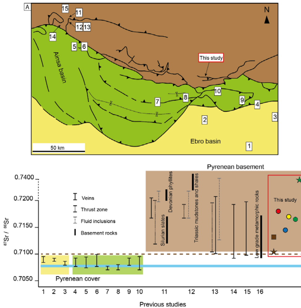
960 Figure 11: Simplified geological map of the south-central Pyrenees showing the location of structures where ^{87}\text{Sr}/^{86}\text{Sr} analysis have been carried out. Below, ^{87}\text{Sr}/^{86}\text{Sr} ratios from this study compared to results from other structures involving either cover units (1- 10) or basement rocks (11-16). The blue thick line refers to the ^{87}\text{Sr}/^{86}\text{Sr} range of Phanerozoic seawater and the dashed brown line represents the ^{87}\text{Sr}/^{86}\text{Sr} limit value between basement and cover structures. 1. El Guix anticline (Travé et al., 2000), 2. Puig Reig 965 anticline (Cruset et al., 2016), 3. L'Escala thrust (Cruset et al., 2018), 4. Vallfogona thrust (Cruset et al., 2018), 5. Ainsa basin (Travé et al., 1997), 6. Ainsa-Bielsa area (McCaig et al., 1995), 7. Minor Bóixols thrust (Muñoz-López et al., under review), 8. Bóixols anticline (Nardini et al., 2019), 9. Lower Pedraforca thrust (Cruset et al., 2020a), 10. Upper Pedraforca thrust (Cruset, 2019), 11. Gavarnie thrust (McCaig et al., 1995), 12. Pic de Port Vieux thrust (Banks et al., 1991), 13. Pic de Port Vieux thrust (McCaig et al., 2000b), 14. Plan de Larri thrust (McCaig et al., 1995), 15. La Glere shear zone (Wayne and McCaig, 1998). 16. Trois Seigneurs Massif (not in the map) (Bickle et al., 1988).
