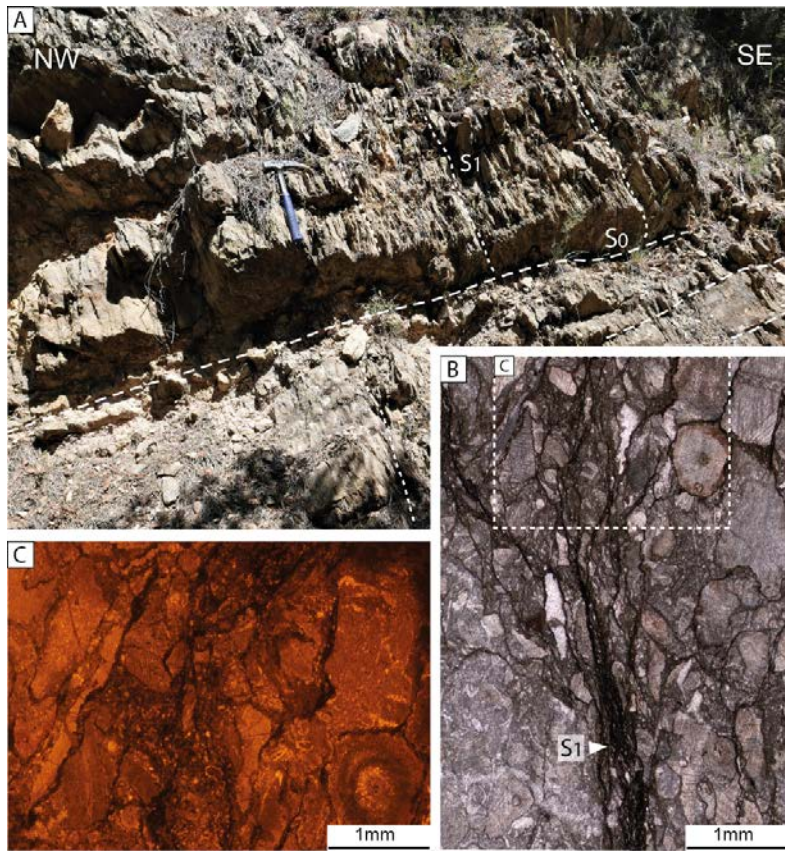
910 Figure 5: Devonian protolith. A) Field image showing the relationship between bedding ( S_0 ) and regional foliation ( S_1 ). B) Plane polarized light and C) Cathodoluminescence microphotographs of the encrinurites alternating with pelitic rich bands, where the S_1 is concentrated.
