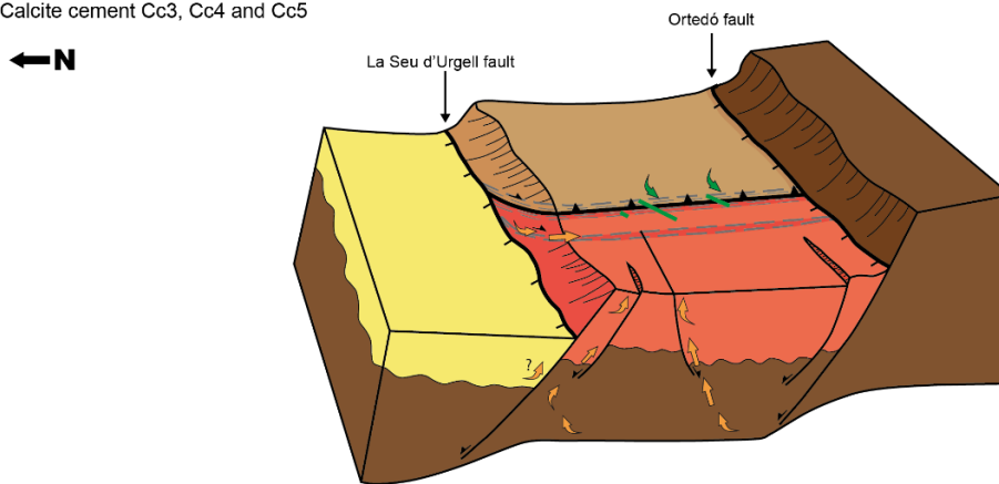
980 Figure 13: Tectonic and geochemical evolution of the study area (not to scale) and relationships with the evolution of the fluid system. A) During the Alpine reactivation of the Estamariu thrust, a meteoric fluid (red arrows) interacted at depth with basement
