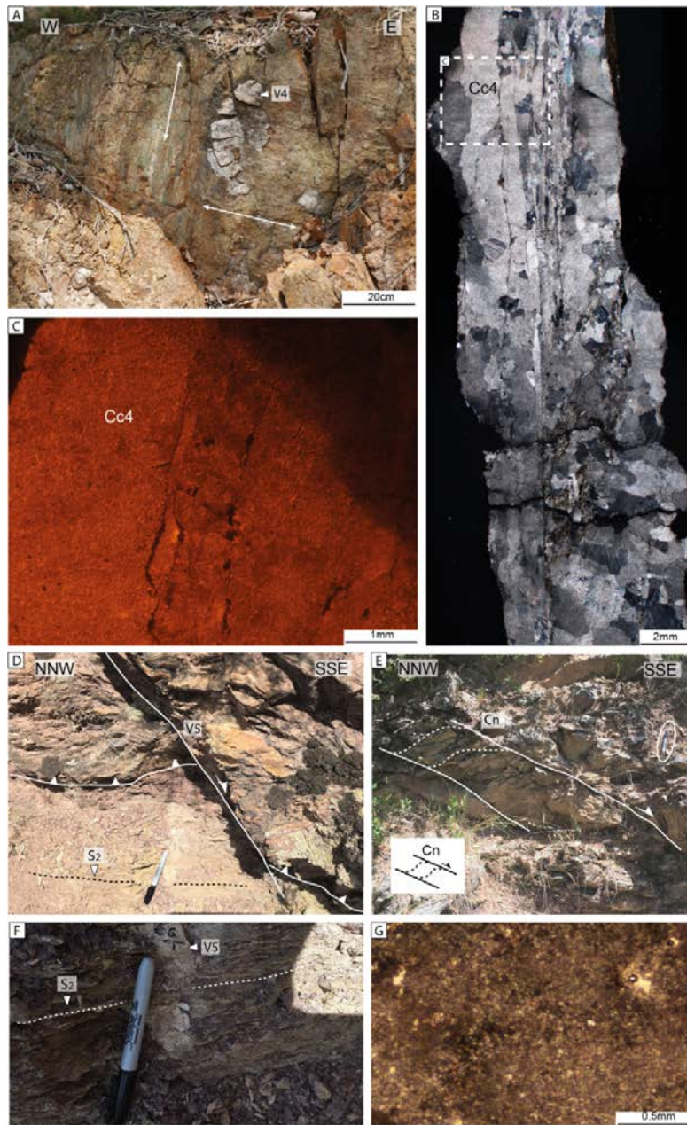
930 Figure 8: A) Field image of a subvertical and E-W fault plane mineralized with calcite (veins V4) and showing two striae set generations (white arrows) indicating dip-slip and strike-slip kinematics. B) Crossed polarized light and C) cathodoluminescence microphotographs of the vein-related calcite cement (Cc4). D) Shear fracture postdating the thrust zone foliation, locally mineralized with calcite veins V5. E) Shear bands (Cn) with normal kinematics located in the main thrust zone, indicating a later reactivation of the Estamariu thrust. (F) Field image of a calcite vein V5 and (G) Plane polarized light of the vein-related cement 935 (Cc5).
