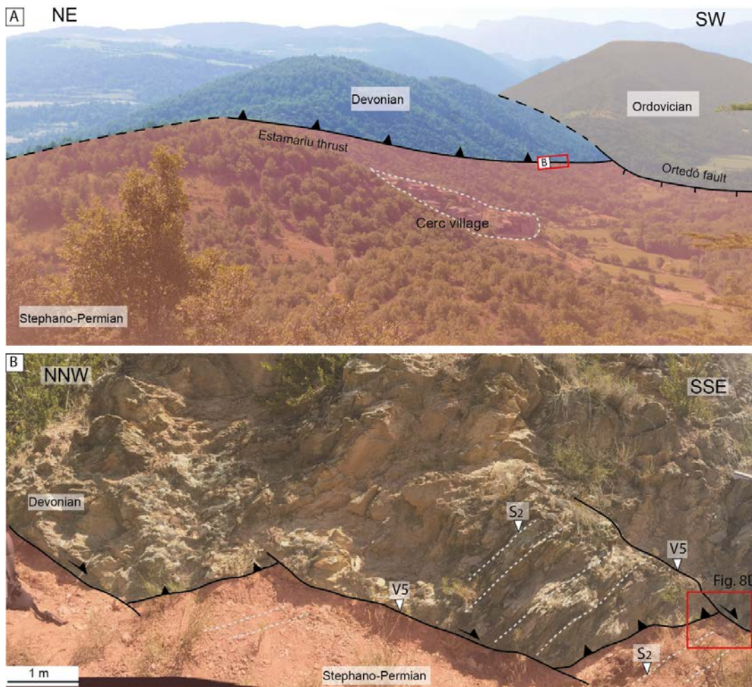
900 905 Figure 4: Main outcrop of the Estamariu thrust. A) Panoramic view from the Sant Antoni hill showing the extensional Ortedó fault postdating the Estamariu thrust. B) Main outcrop showing the Estamariu thrust and the related thrust zone foliation developed in the Devonian hanging wall and in the Stephano-Permian footwall ( S_2 ). The thrust is displaced by later shear fractures locally mineralized with calcite (V5).
