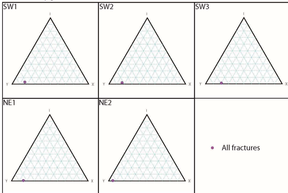
995 Fig. 12: Ternary plots visualizing the node distributions. For the manual interpretations, the different network stages in terms of fracture generations are plotted. The automatic networks only show the final stage of the network, which corresponds to generations 1 – 5 in the manual interpretation. Nodes with four and more than four intersecting branches have been binned as type X nodes.
