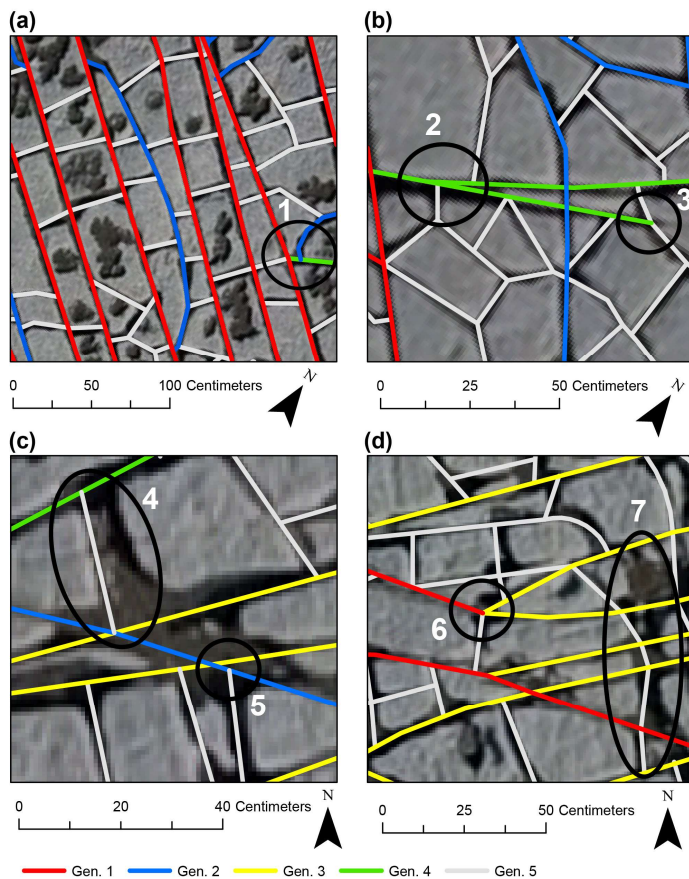
1075 Fig. 24: Details of the manual interpretation of fracture generations showing examples that allow for different interpretations of the generation and network geometry. (a) The fracture in the center of the image was assigned to gen. 2 (blue) because it abuts twice at the same gen.1, fracture, which is atypical for fractures of gen. 2 and was decided by elimination of the other interpreted generations. Mark 1 shows an interpretation where gen.2 appears to abut on gen. 4, which then abuts on gen. 1 towards the left. This is an example in which the initial tracing of the network was unclear because of the widely eroded intersection of the fractures and has been revised during the assignment of generations. (b) Mark 2 shows a splaying gen. 4 fracture, which is a rare case and could also be interpreted as a younger fracture abutting on gen. 4. Mark 3 shows the tip of gen.4 which apparently abuts on gen. 5. The small darker in front of the tip suggests, that the fracture may continue, or the surface of the rock has been eroded in that place or is wet, in which case the interpreter decided to end the trace. (c) Mark 4 shows a widely eroded fracture which has been traced along one of the edges instead along its median axis. The reasoning behind this decision is the assumption, that the left edge sharper and straighter than the one on the right, which suggests a stronger erosion in that part. Therefore, the left edge was interpreted as the best representation of the fracture geometry in this case. Mark 5 shows a gen. 5 fracture abutting on gen.2. However, the wide erosion of the fracture itself and the junction of gen. 2 and gen. 3 towards the left, also allow the interpretation as a triple junction of generations 2, 3 and 5. (d) Mark 6 shows a junction where the gen.1 fracture was interpreted to stop, while the trace continues as gen.3 which initially follows the rough strike direction of gen. 1 and then bends towards the strike direction of gen. 3. Mark 7 shows another strongly eroded area that hinders the interpretation of fractures.
