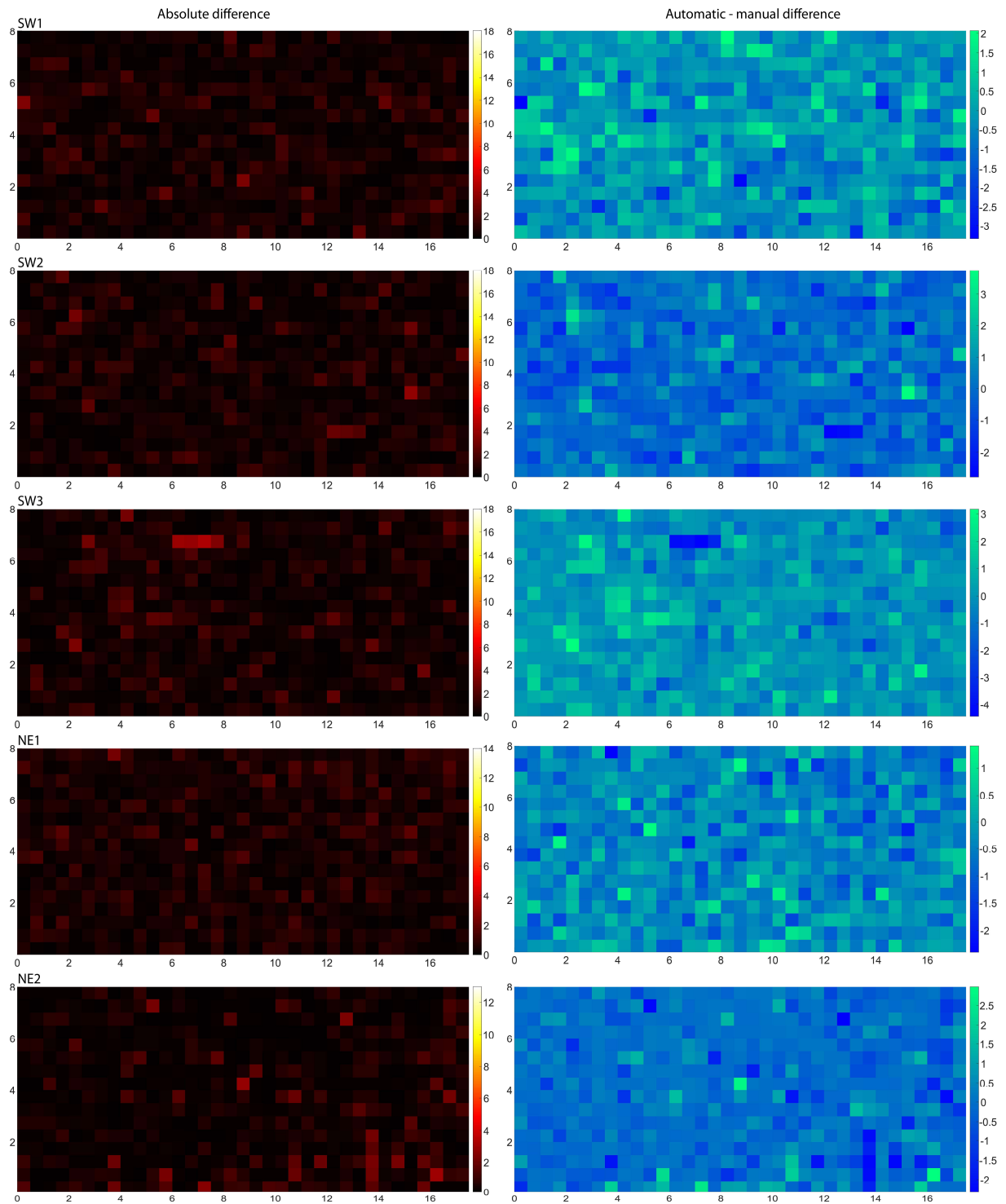
Fig. 9: Differences of the P_{21} fracture segment intensity between manually- and automatically-traced fracture segments for all five domains. Absolute differences are shown in the left column, relative differences in the right column. Unit of the axes in (m), unit of the color bar in ( m^2 ).
