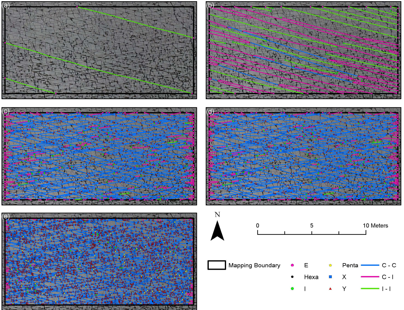
Fig. 18: Development of the fracture network in time steps for SW1 from generation 1 to 5, visualized as branches and nodes. The consecutive fracture generation is added for each panel from (a) to (e).
