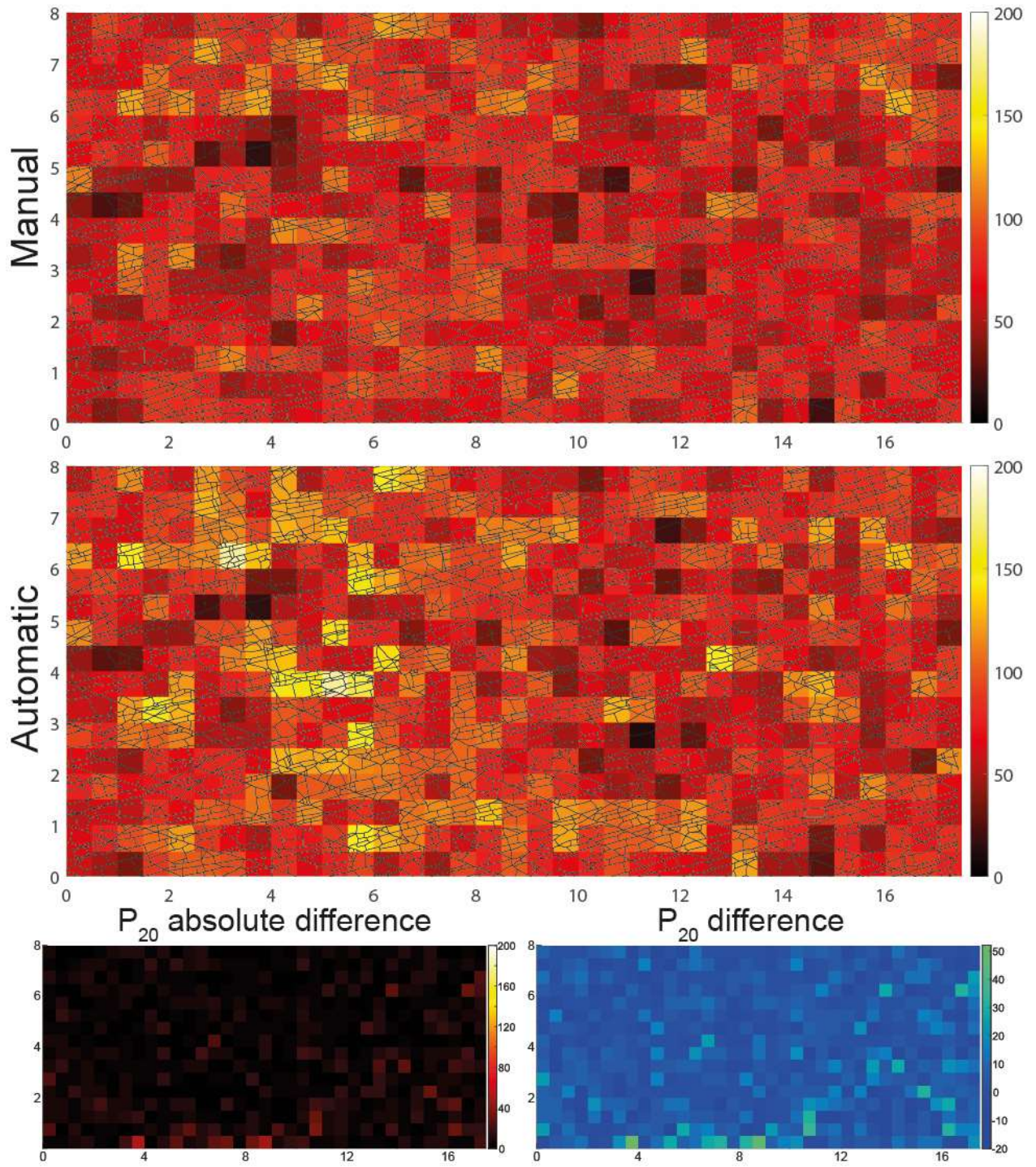
Fig. 6: Comparison of the P_{20} fracture segment density between manually an automatically-traced fracture segments for SW3. Absolute and relative differences are shown in the bottom line. Unit of the axes in (m), unit of the color bar in ( 1/m^2 ).
