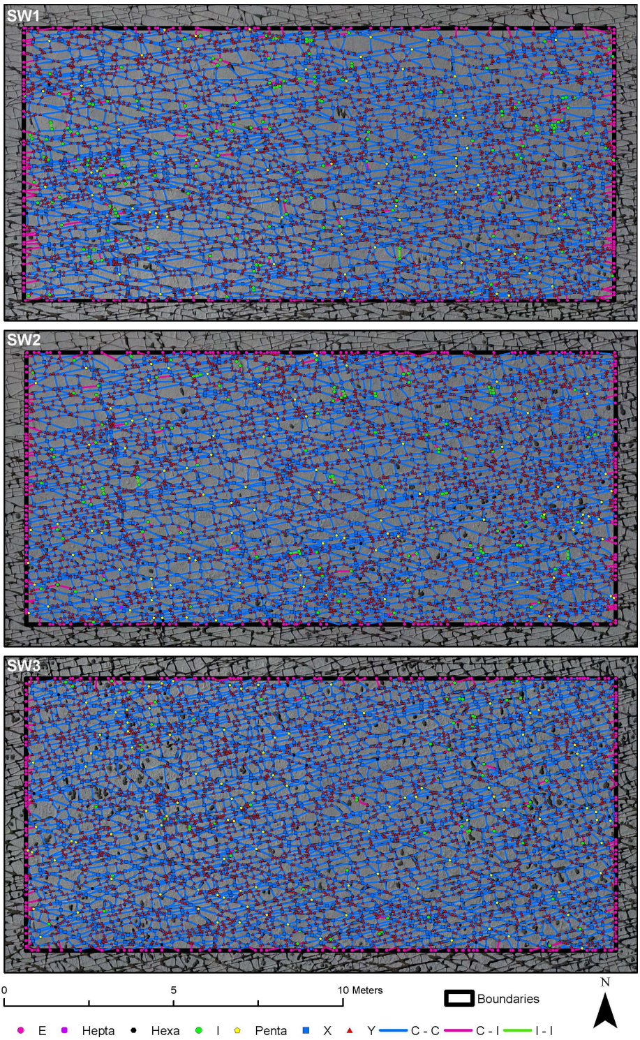
Fig. 10: SW fracture networks, automatically-traced and plotted as branches and nodes.
