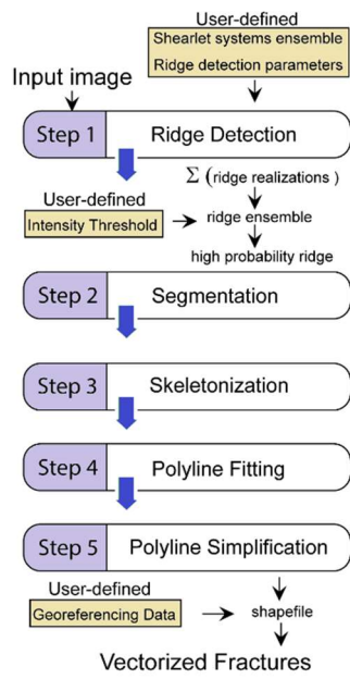
Fig. 3: Overview of the automated fracture detection process (reproduced with permission from Prabhakaran et al, 2019)
