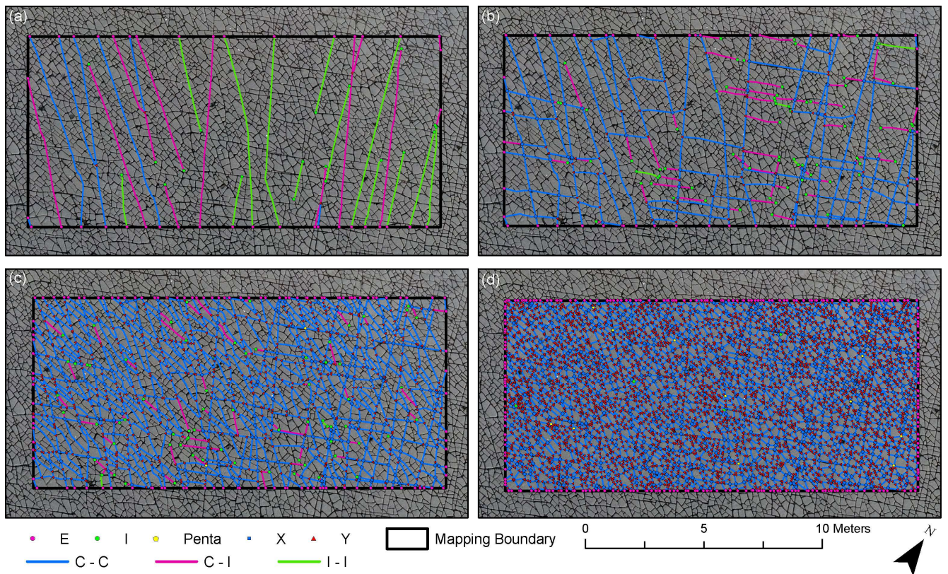
1050 Fig. 21: Development of the fracture network in time steps for NE1 from generation 1 to 5, visualized as branches and nodes. The consecutive fracture generation is added for each panel from (a) to (d). Note that no fractures belonging to gen. 3 were identified in this domain.
