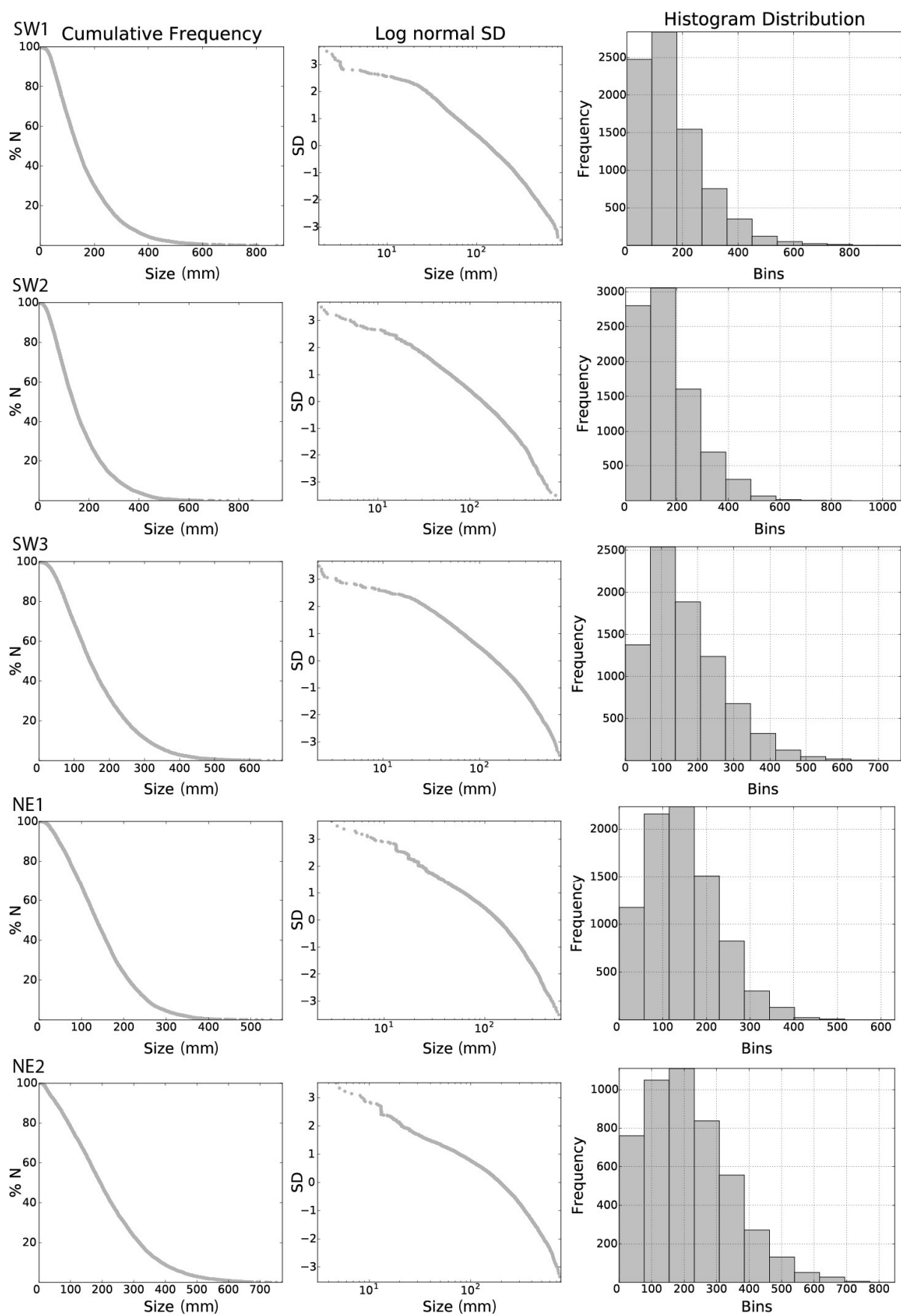
Fig. 4: Cumulative length, log normal standard deviation and histogram distributions of the automatically-traced fractures (branches) in the five domains.
