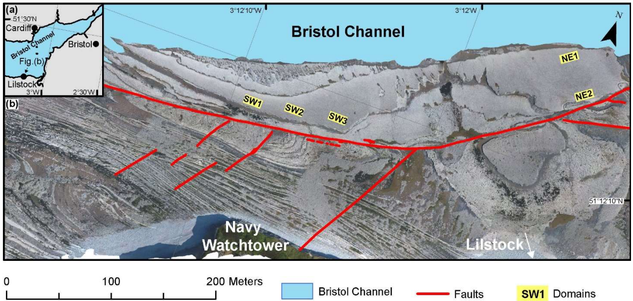
950 Fig. 1: (a) Location of the study area in the Bristol Channel, Great Britain. (b) Ortho-rectified photo-mosaic of UAV-photographs taken from 100 m. The ortho-mosaic shows the coast at Lilstock during low tide, exposing the fractured limestone. The map domains on “the bench” are marked as yellow rectangles.
