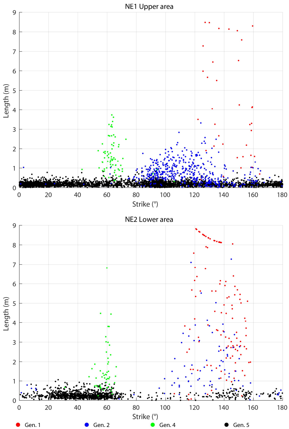
1035 Fig. 17: Plots of strike direction (°) on the x-axis and length (m) on the y-axis for every fracture mapped in the domains in the NE, color coded by generation.
