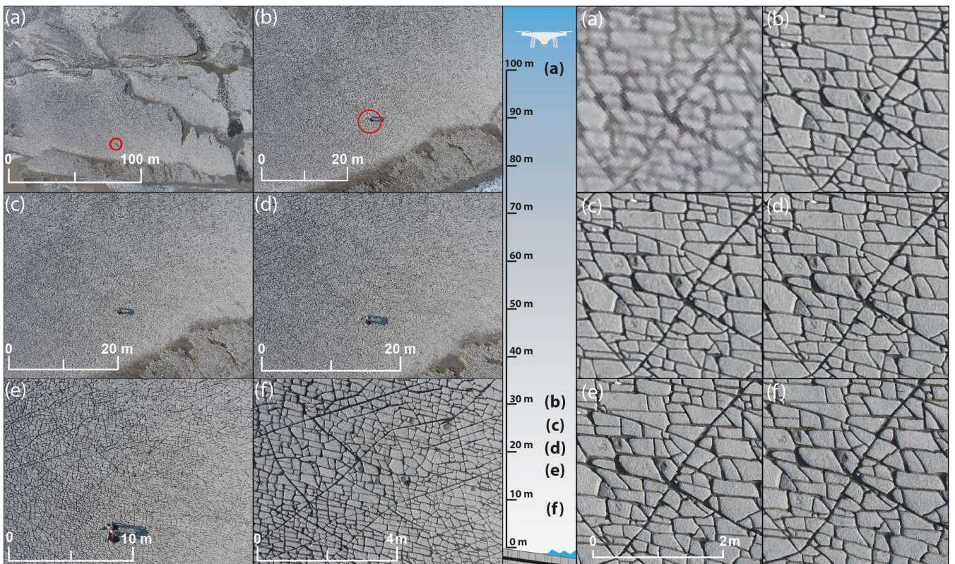
955 Fig. 2: The fractured limestone captured from above by UAV. Left: View from different altitudes with altitudes decreasing from (a) to (f). The exact altitudes from which the photographs have been taken can be viewed in the sketch in the center. Right: Same photographs as on the left, zoomed in to the same degree and location in every image. With increasing altitude, the spatial resolution of the image decreases. Note: persons for scale and encircled for better visibility in (a) and (b) on the left.
