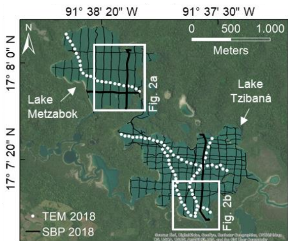
755 Figure 1: Layout of the geophysical survey on lakes Metzabok and Tzibaná during high-level stands in March 2018. Black lines show the sub-bottom profiler (SBP) survey grid, bold lines highlight those profiles discussed in detail in this manuscript, white circles represent individual transient electromagnetic soundings (TEM). The optical satellite image in the background (source: Bing Maps data base) shows lake water surface similar to the high-level stands encountered during March 2018.
