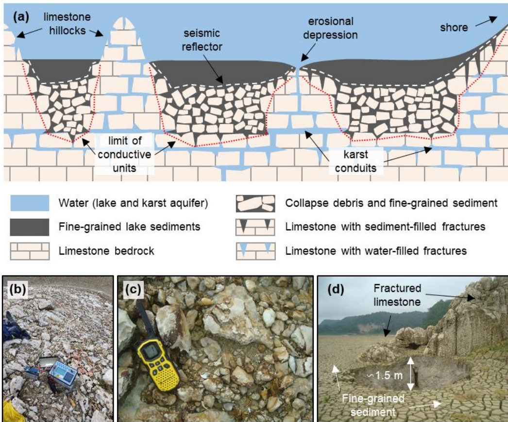
805 Figure 8: (a) Schematic sketch summarizing the geological conditions below Lake Metzabok interpreted from the geophysical survey (details not drawn to scale). The limit between the fine-grained lake sediments and the collapse debris with sediment-filled interspaces indicated by the white dashed line stands out as a strong reflector in all sub-bottom profiler images. All units containing fine-grained sediment are characterized by low electrical resistivity values; a strong resistivity increase marks the upper limit of the limestone bedrock as indicated by the red dotted line. Photographs show (b) and (c) limestone debris with fine-grained sediment as 810 well as (d) fractured limestone and fine lake sediments exposed during the low-level stands in October 2019.
