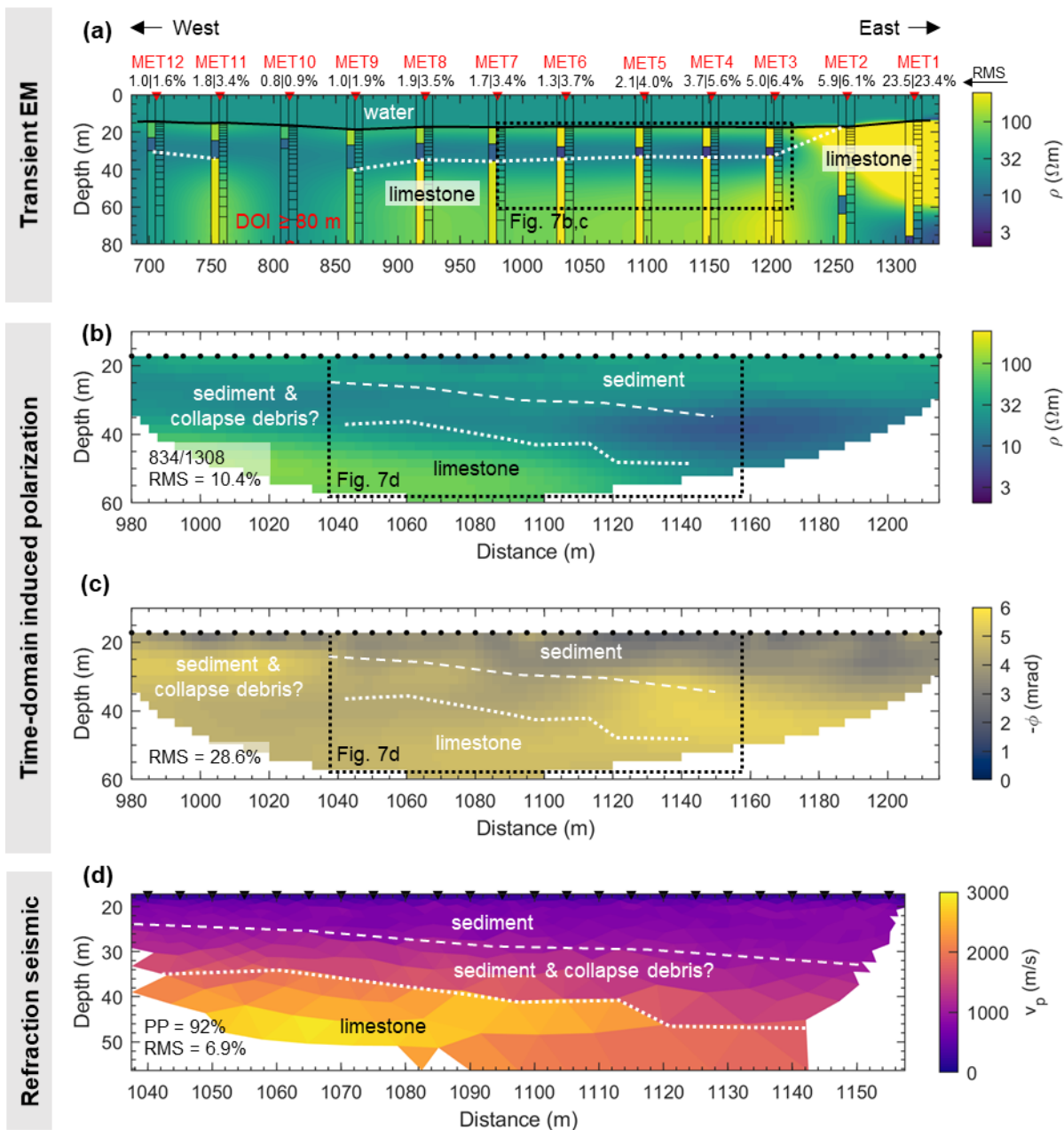
795 Figure 7: Geophysical sections along Profile 4 of Lake Metzabok: (a) Interpolated TEM image based on smooth 1D models, left bar graphs show layered, right bar graphs smooth models; individual percentage RMS deviations are given for layered and smooth models, respectively. The black solid line in the section indicates the water-sediment contact, the dotted line the top of the limestone bedrock inferred from this image. (b) Electrical resistivity and (c) phase images including electrode positions (black dots along the surface), and the main lithological units as interpreted from the SRT image in (d) (dotted lines). Labels in the lower left corners of 800 (b) and (c) represent the amount of data points used for the inversion compared to the total measured data (same for resistivity and phase) and the respective percentage RMS of the inversion. (d) Seismic refraction tomogram with main lithological units including picking percentage (PP) and RMS of the inversion.
