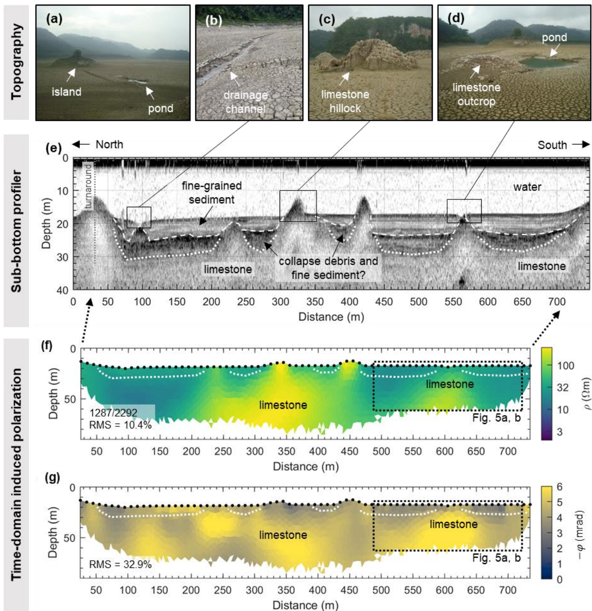
Figure 4: Topographic features and geophysical sections along Profile 1 of Lake Metzbok. Photographs of topographical features taken in October 2019: (a) lake basin with flat bottom, (b) drainage channel, (c) limestone hillock, (d) deep fracture and pond next to shallow limestone outcrop. (e) Sub-bottom profiler (SBP) section with dashed lines highlighting the main reflector encountered below the lake floor and dotted lines outlining a zone of high diffuse reflectivity, (f) and (g) electrical resistivity and phase images, respectively, including electrode positions (black dots along the surface) and dotted lines taken from SBP section. Electrical sections are shifted by 25 m with respect to the SPB section. Labels in the lower left corners of (f) and (g) represent the amount of data points used for the inversion compared to the total measured data (same for resistivity and phase) and the respective percentage root mean square deviations (RMS) of the inversion.
