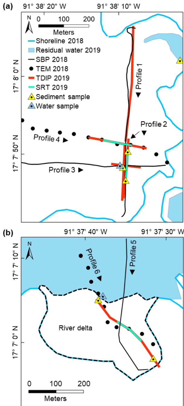
760 Figure 2: Layout of the geophysical survey on lakes Metzabok (a) and Tzibaná (b) in October 2019 (after the sudden lake-level drop) 765 including sub-bottom profiler (SBP), transient electromagnetic (TEM), time-domain induced polarization (TDIP), and seismic refraction tomography (SRT) measurements. The geophysical measurements discussed here are grouped into five profiles; black triangles next to the profile names indicate the profile orientations. Yellow and blue triangles indicate sampling locations for sediment and water samples analysed in the laboratory, respectively. The dashed black line in (b) indicates the dry part of the river delta exposed during October 2019.
