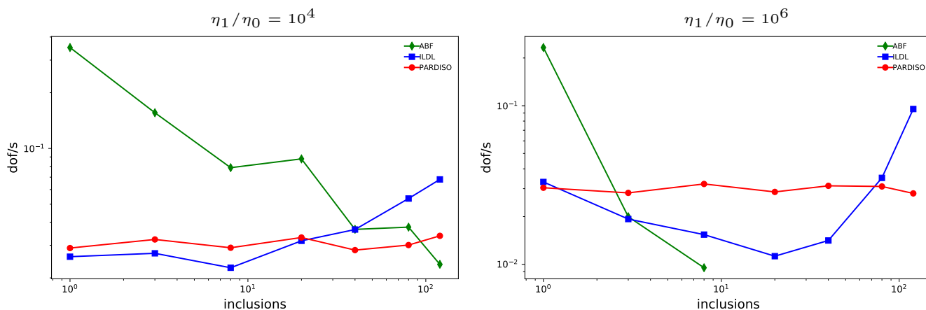
Figure 2. The effect of increasing the number of viscous inclusions on the effectiveness of solvers, for a 32^3 element simulation. ILDL preconditioning becomes more competitive for more challenging structures, showing much greater robustness to viscosity structure than ABF solvers while maintaining a lower memory footprint than direct solution. Missing ABF data indicate that the solver failed to converge. Memory footprints are similar to those shown in Figure 1; the direct solve (red) requires approximately 4\times as much memory as the ILDL-preconditioned solve.
