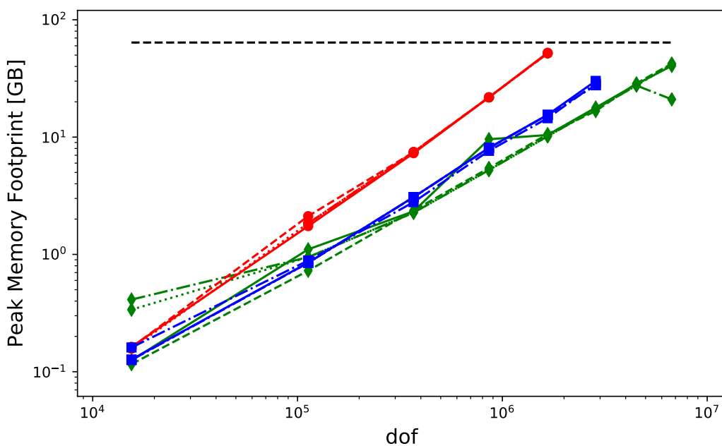
Figure 1. Additional experiments, analogous to those in Table 1. Solver performance is assessed in terms of degrees of freedom solved to the prescribed tolerance ( 10^{-6} relative error in the true residual norm) over the solution time, and by peak memory footprint.
