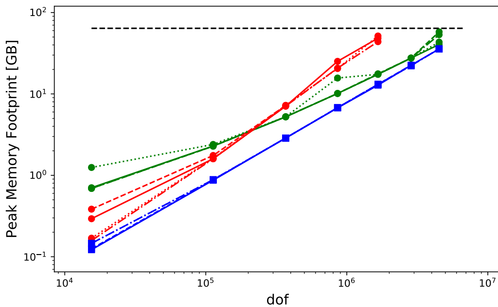
(c) 1 inclusion, \lambda_1/\lambda_0 = 10^4
