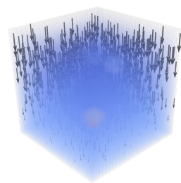
(a) 3 inclusions, \lambda_1/\lambda_0 = 10^4
