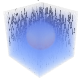
(c) 1 inclusion, \lambda_1/\lambda_0 = 10^4
