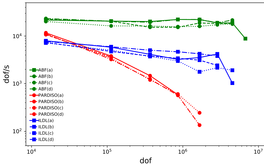
(a) 3 inclusions, \lambda_1/\lambda_0 = 10^4
