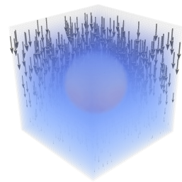
(b) 1 inclusion, \lambda_1/\lambda_0 = 10^2
