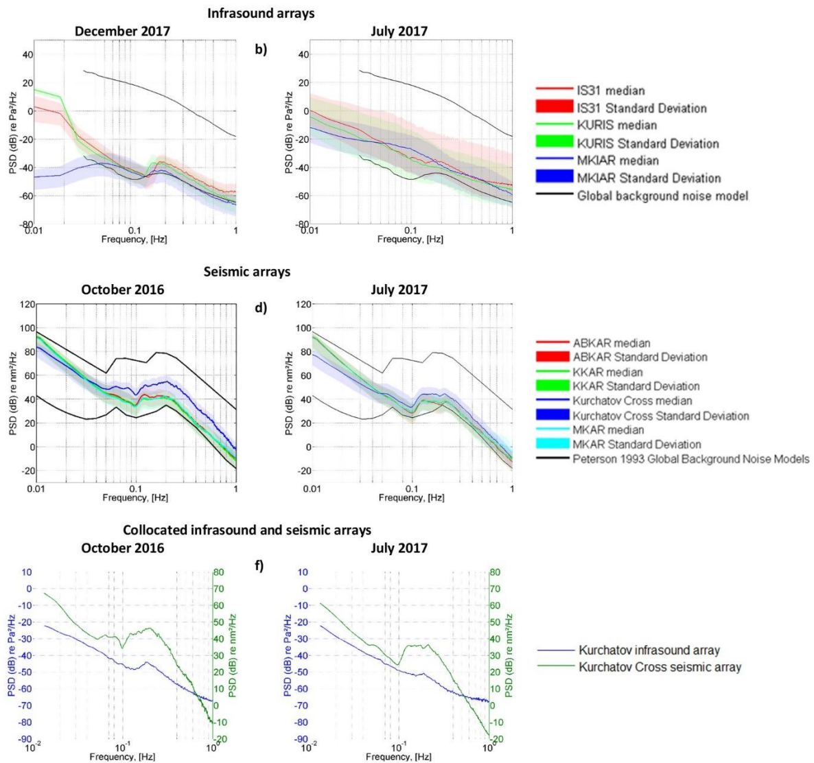
525 Figure B1. PSD noise spectra at infrasound arrays (a,b) and seismic arrays (c,d). Comparison of noise spectra at colocated KURIS and Kurchatov Cross arrays.
