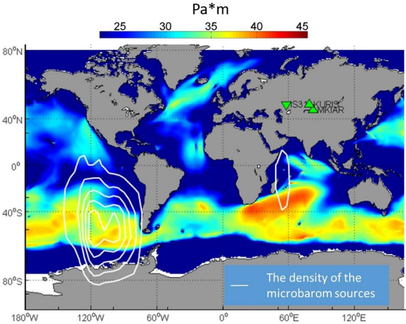
535 Figure C2. Spatial distribution of the epicentres of microbarom sources in July-August 2017. White contours represent the density of the microbarom source locations obtained via cross-bearing using detections at IS31, KURIS and MKIAR, during same time periods. At each station, back-azimuths are daily averaged. 25
