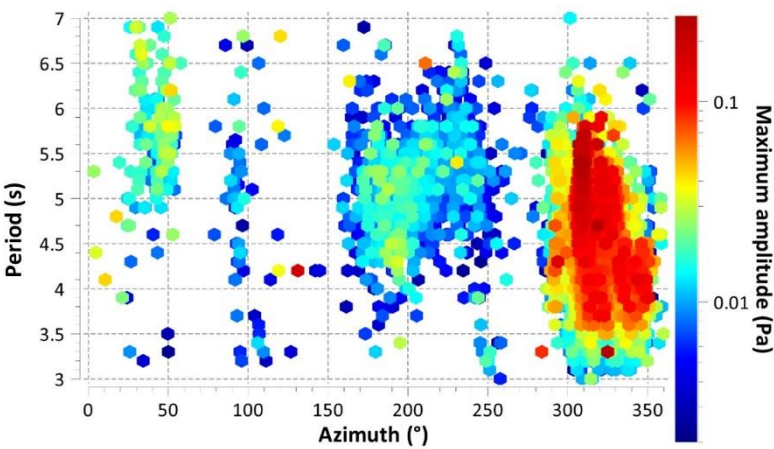
530 Figure C1. Signal periods versus back-azimuths at IS31 observations in 2017. The amplitude is color coded (in Pa).
