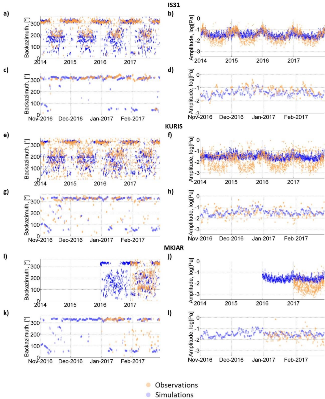
Figure 2. Time variations of observed back-azimuths and amplitudes of microbaroms at IS31 (a-d), KURIS (e-h), and MKIAR (i-l), with a time resolution of 6 hours from January 1, 2014 to December 31, 2017 (orange circles). Blue circles denote simulated values. Details at IS31 (c,d), KURIS (g,h) and MKIAR (k-l).
