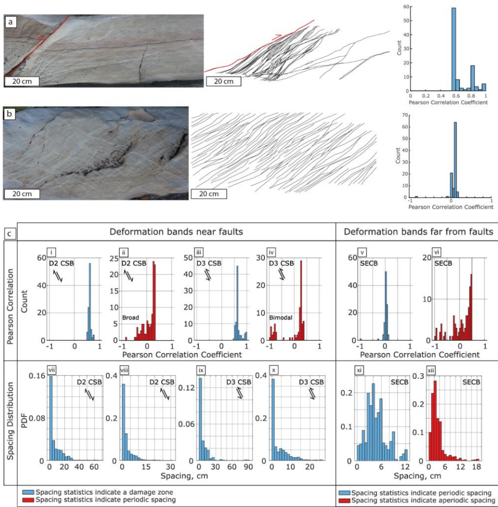
975 Figure 17. [a] Spacing analysis of CSBs hosted in the damage zone of a small reverse-fault with up to 20 cm displacement. The image documents the upper end of the fault, approaching the tip. [b] Spacing analysis of dominantly SECBs with rare CSBs not associated with the damage zone of faults. The bands show a near constant spacing with a median spacing of 1.3 cm. 100 scan-lines were taken for images [a] and [b]. The Pearson correlation coefficient values for [a] are mostly >0.5 indicative of a positive correlation between
