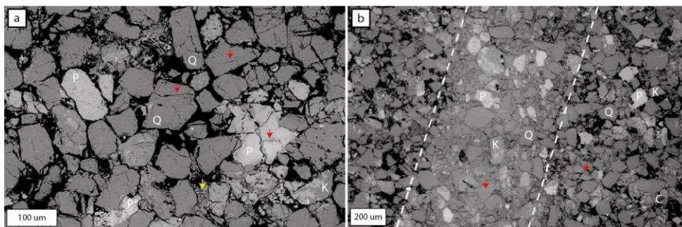
Figure 8. Microseopic-BSE images of D2 normal-sense compactional shear bands and associated host rock. [a] A normal-sense compactional shear band hosted within less deformed host rock. The white dashed lines indicate the edge of the deformation bands. [a], [b], [c], [d], [e], [f] images of deformation bands. The deformation bands associated with D2 horizontal extension have diffuse edges and are characterised by reduced porosity and increased clay content. The red arrows denote the location of microfractures. Microfractures are observed in grains present within the deformation band, and within grains hosted within the host rock. The host rock is characterised by higher porosity when compared to the deformation band. Panel [b] is an image of host rock sampled within 5 cm of a normal-sense deformation band. [g] and [h] are images of host rock surrounding deformation bands. Within the host rock microfractures are present, with some examples highlighted by red arrows. In addition, pockets of smaller grain size can be seen with higher clay content indicating the lithological heterogeneity of the unit. Such an example is indicated by the yellow arrow. Q = quartz. C = zones of clay-sized particles. K = potassium feldspar. P = plagioclase. P* = deformed plagioclase.
