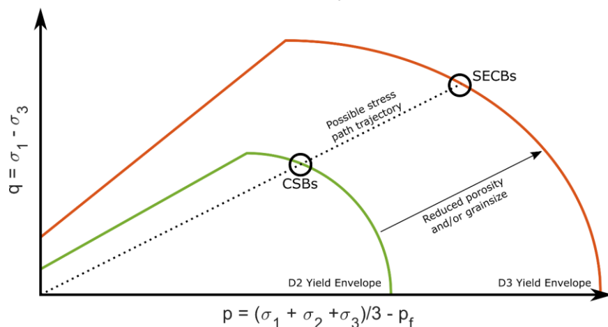
Figure 24-19. Schematic diagram of the potential yield envelopes for the Whakataki Formation during D2 horizontal extension and D3 horizontal contraction. During D2, the unit is still lithifying and being buried, therefore, in D3 when the unit has lithified, the yield cap has expanded (red line). For a generic increase in effective stress ( p ) and differential stress ( q ), the yield cap may be intersected at different points due to the evolution of the yield envelope through time. With only two points to constrain the stress path, there are many possible trajectories, all of which could result in the observed deformation band kinematics and distributions. In fact, the linear stress path shown here for illustration purposes cannot be correct because the stress regime in the Whakataki Formation switched at least two times. This figure follows the models developed in Soliva et al. (2013).
