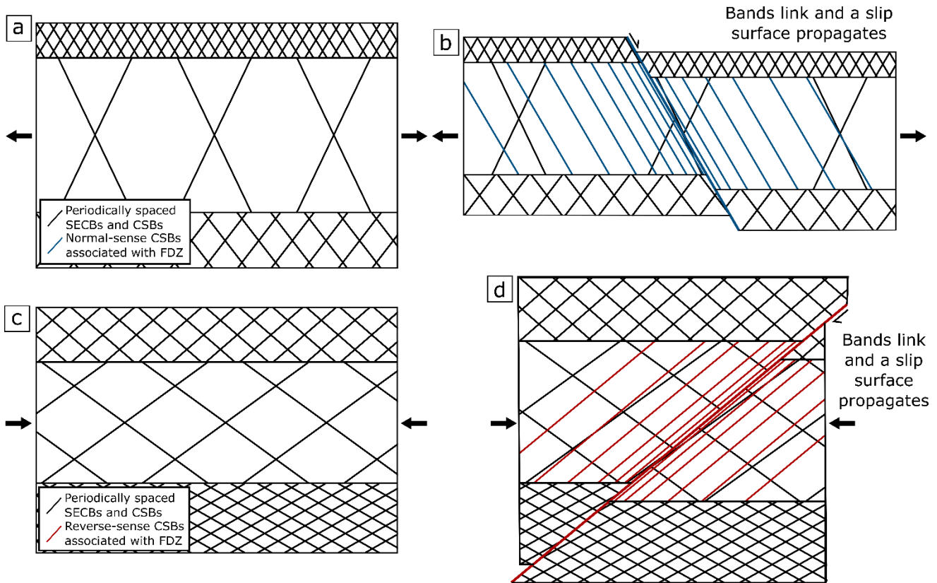
870 Figure 20. A schematic to show the evolution of spatial distributions in normal- (a & b) and reverse-faulting (c & d) tectonic regimes. Initially, bands with an equal spacing form. Band spacing is theorised to be proportional to the layer thickness, as is observed with joints (Pollard and Aydin, 1988; Gross, 1993). Eventually, bands link across layers and a fault propagates (Aydin and Johnson, 1983). The fault movement causes the local stress field to be perturbed resulting in new band formation with orientations and kinematics matching that of the new local stress field.
