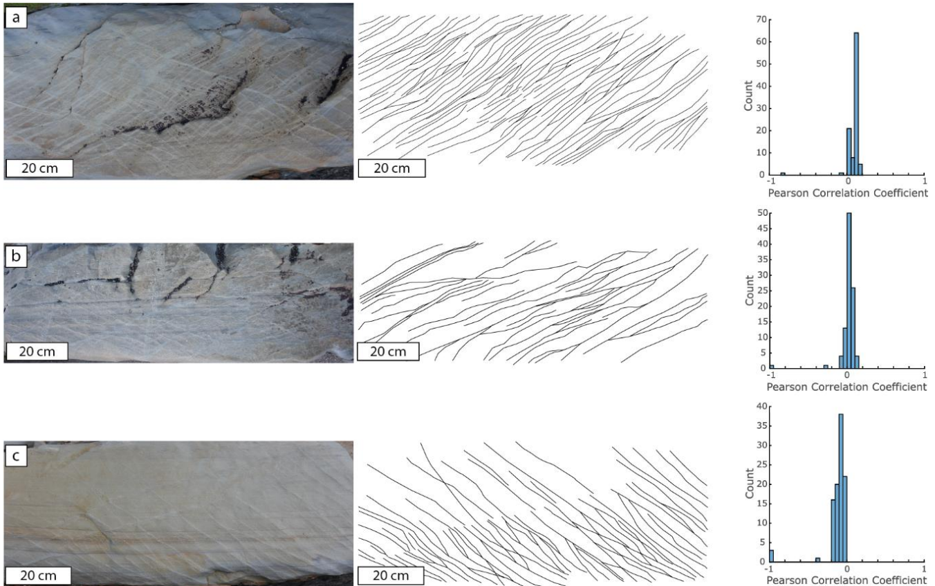
705 Figure 18. Spacing analysis of dominantly SECBs with rare CSBs not associated with the damage zone of faults. 100 scan-lines were taken for each image during analysis. Each image shows a general lack of correlation of the distance with the spacing between deformation bands. Pearson correlation coefficient values close to 0 further suggest a lack of correlation. These bands show a near-constant spacing. Median spacing: [a] = 1.3 cm; [b] = 1.8 cm; and [c] = 2.3 cm.
