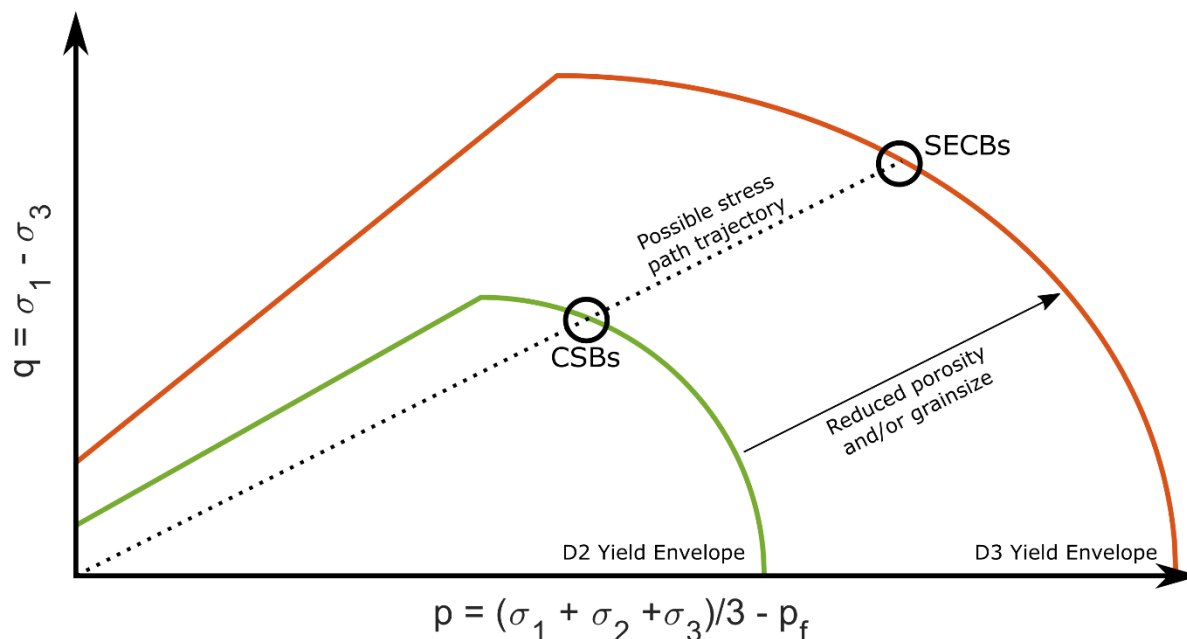
Figure 21. Schematic diagram of the potential yield envelopes for the Whakataki Formation during D2 horizontal extension and D3 horizontal contraction. During D2, the unit is still lithifying and being buried, therefore, in D3 when the unit has lithified, the yield cap has expanded (red line). For a generic increase in effective stress ( p ) and differential stress ( q ), the yield cap may be intersected at different points due to the evolution of the yield envelope through time. With only two points to constrain the stress path, there are many possible trajectories, all of which could result in the observed deformation band kinematics and distributions. In fact, the linear stress path shown here for illustration purposes cannot be correct because the stress regime in the Whakataki Formation switched at least two times. This figure follows the models developed in Soliva et al. (2013).
