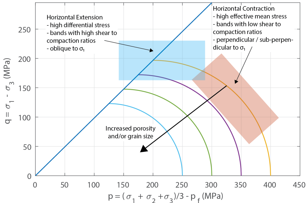
55 Figure 1. Cam-cap yield envelope showing the relationship between the stress state at the point of inelastic yielding and the type and orientation of the deformation band that nucleates. In horizontal contraction, higher effective mean stresses are predicted which results in the formation of bands characterised by low shear to compaction ratios. Comparatively, during horizontal extension, higher differential stresses are predicted resulting in bands characterised by high shear to compaction ratios. The yield envelope shrinks with increased porosity and/or grain size of the material. Adapted from Fossen et al. (2007).
