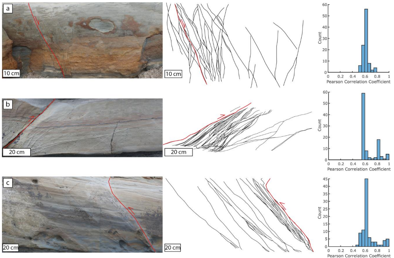
680 Figure 17. Spacing analysis of CSBs associated with the damage zone of faults. 100 scan-lines were taken for each image during analysis. [a] represents a D2 normal fault and [b] and [c] show small D3 reverse faults. Each of the three faults show an increase in spacing between deformation bands with increasing distance from the fault plane. This is reflected in the Pearson correlation coefficient. Values are approaching 1, which shows a dependence of distance on spacing.
