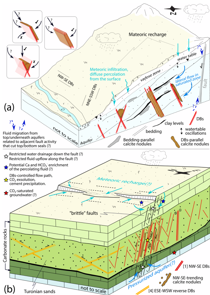
Figure 13. Generalized conceptual model for calcite nodules precipitation in the two study areas: (a) Loiano and (b) Bollène. See text (Sect. 7.2) for details. The inset sketches in (a) show possible paleo-fluid flow direction at the time of calcite precipitation for different “DBs-nodule” configurations.
