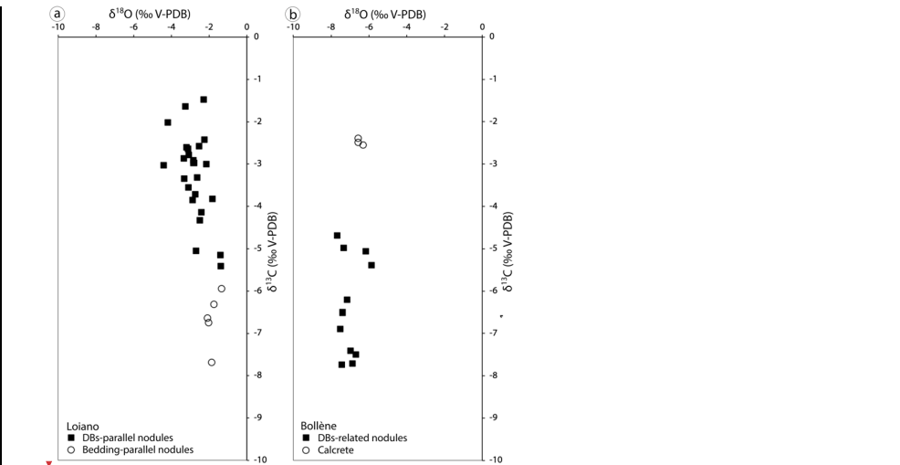
Figure 12. Stable isotopes analysis results. (a) Cumulative isotopic data characterizing the DBs-parallel nodules (black full-dots) and bedding-parallel ones (empty-dots) inside the Loiano Sandstones. (b) Isotopic data from the DBs-related nodules (black full-dots) and cement sampled in the calcrete (empty-dots) in Bollène quarry (see the Supplement S2 for details).
